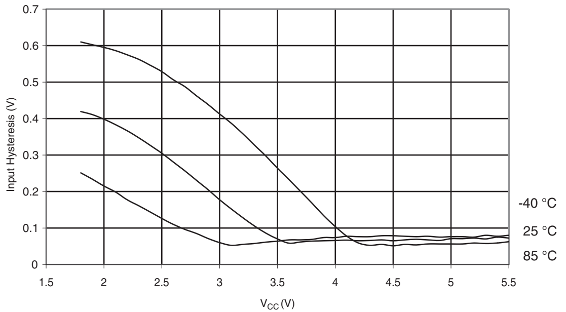
Figure 29-352. ATmega328P: Reset Pin Input Hysteresis vs. V_{CC}
