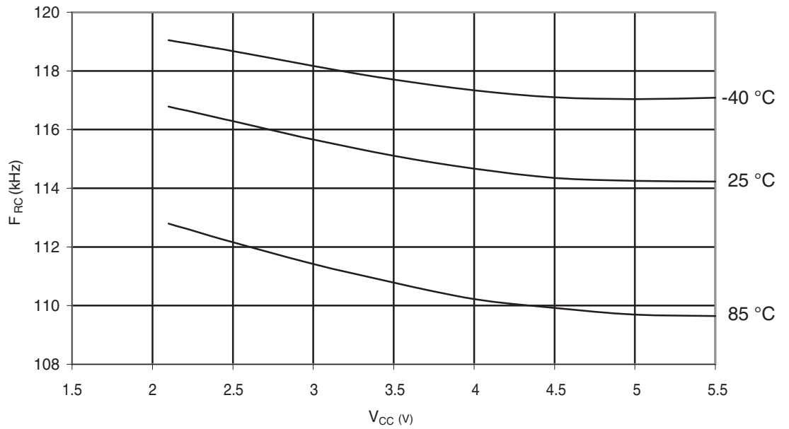
Figure 29-311. ATmega328: Watchdog Oscillator Frequency vs. V_{CC}
