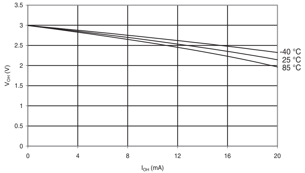
Figure 29-69. ATmega48PA: I/O Pin Output Voltage vs. Source Current ( V_{CC} = 3\text{ V} )
