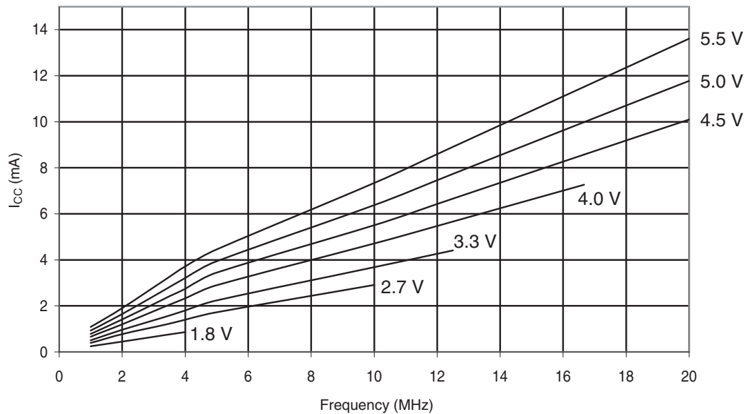
Figure 29-324. ATmega328P: Active Supply Current vs. Frequency (1-20 MHz)
