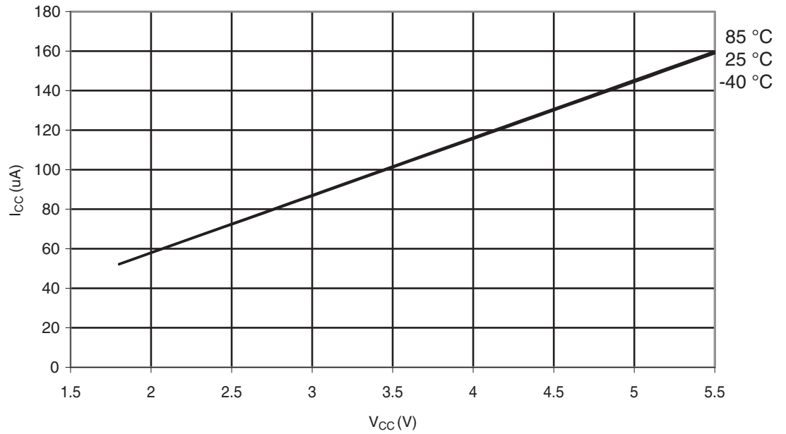
Figure 29-363. ATmega328P: AREF External Reference Current vs. V_{CC}
