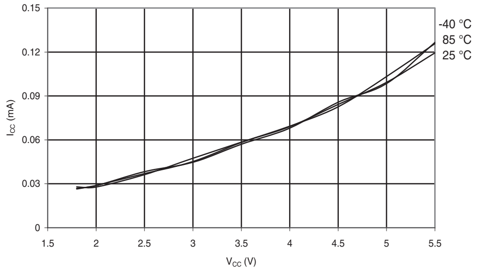
Figure 29-187. ATmega168A: Active Supply Current vs. V_{CC} (Internal RC Oscillator, 128 kHz)
