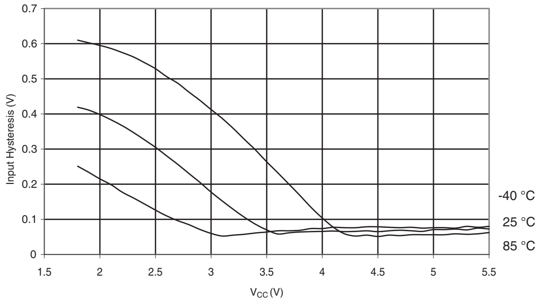
Figure 29-306. ATmega328: Reset Pin Input Hysteresis vs. V_{CC}
