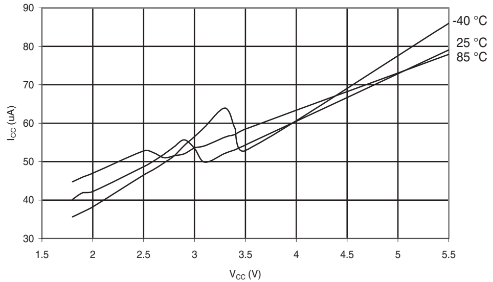
Figure 29-270. ATmega168PA: Analog Comparator Current vs. V_{CC}
