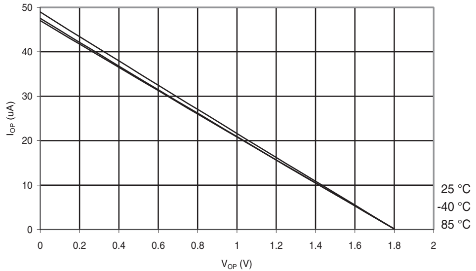
Figure 29-199. ATmega168A: I/O Pin Pull-up Resistor Current vs. Input Voltage ( V_{CC} = 1.8\text{ V} )
