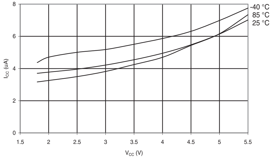
Figure 29-196. ATmega168A: Power-Down Supply Current vs. V_{CC} (Watchdog Timer Enabled)
