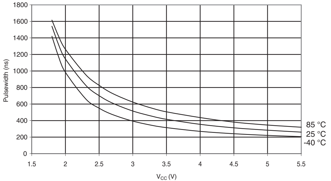
Figure 29-368. ATmega328P: Minimum Reset Pulse width vs. V_{CC}
