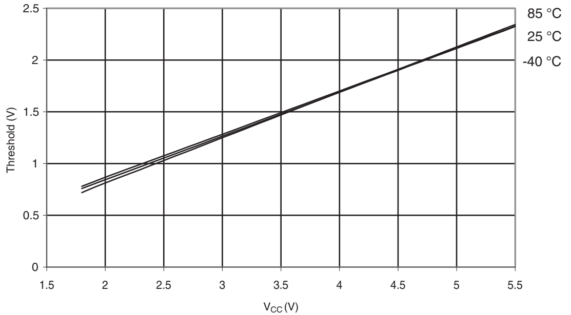
Figure 29-351. ATmega328P: Reset Input Threshold Voltage vs. V_{CC} ( V_{IL} , I/O Pin read as '0')
