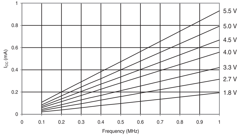
Figure 29-139. ATmega88PA: Active Supply Current vs. Low Frequency (0.1-1.0 MHz)
