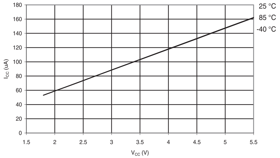
Figure 29-271. ATmega168PA: AREF External Reference Current vs. V_{CC}
