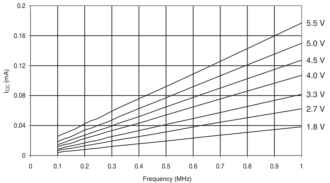
Figure 29-282. ATmega328: Idle Supply Current vs. Low Frequency (0.1-1.0 MHz)
