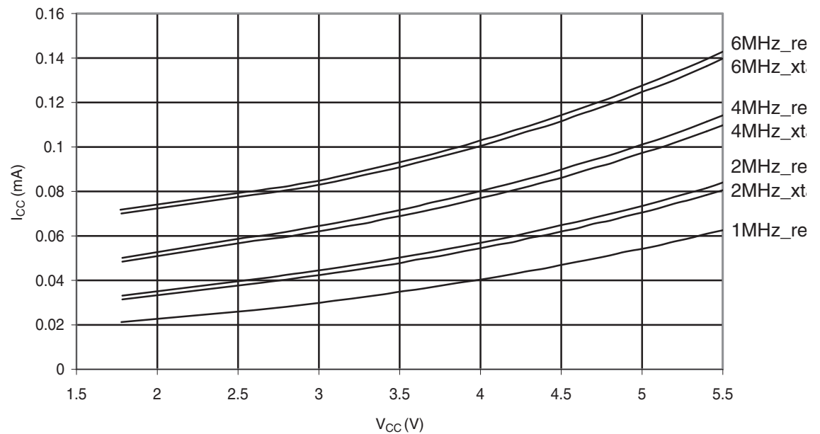
Figure 29-290. ATmega328: Standby Supply Current vs. V_{CC} (Watchdog Timer Disabled)
