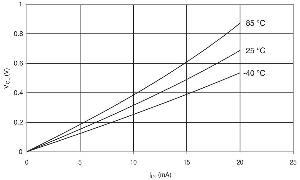
Figure 29-343. ATmega328P: I/O Pin Output Voltage vs. Sink Current ( V_{CC} = 3\text{ V} )
