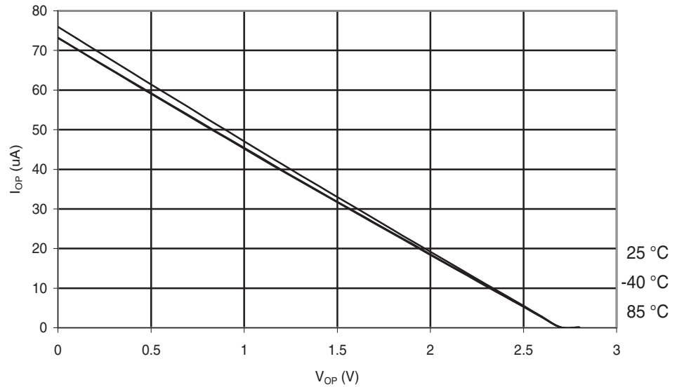
Figure 29-246. ATmega168PA: I/O Pin Pull-up Resistor Current vs. Input Voltage ( V_{CC} = 2.7\text{ V} )
