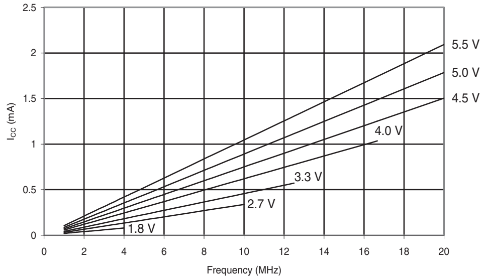
Figure 29-275. ATmega168PA: Reset Supply Current vs. Frequency (1 - 20 MHz)
