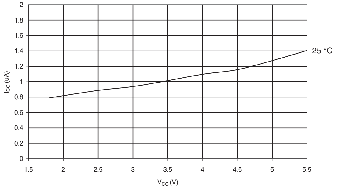
Figure 29-289. ATmega328: Power-Save Supply Current vs. V_{CC} (Watchdog Timer Disabled and 32 kHz Crystal Oscillator Running)
