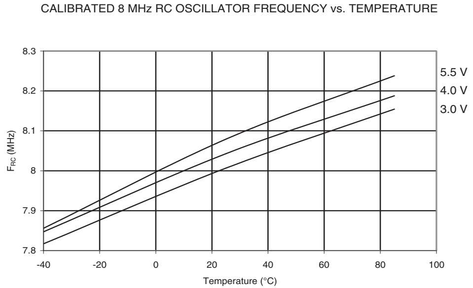
Figure 29-129. ATmega88A: Calibrated 8 MHz RC Oscillator Frequency vs. Temperature
