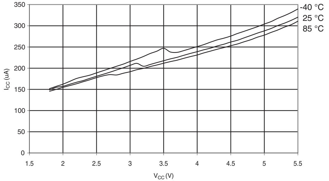
Figure 29-315. ATmega328: ADC Current vs. V_{CC} (AREF = AV_{CC} )
