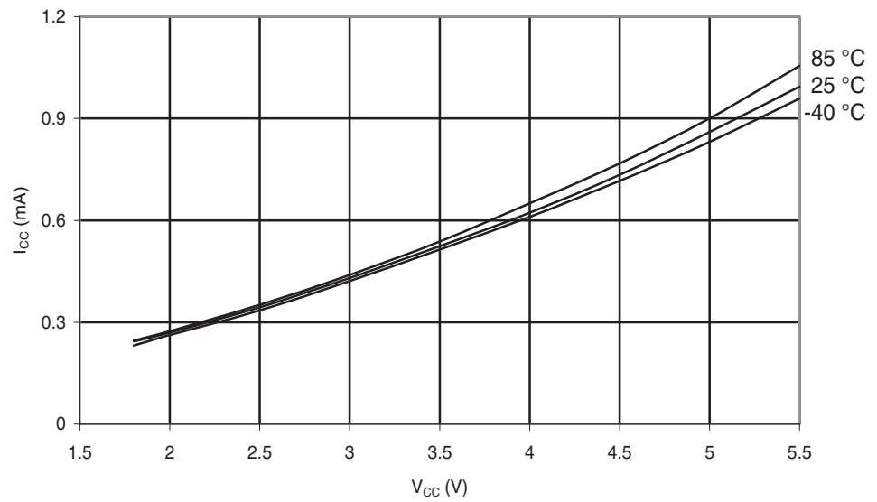
Figure 29-102. ATmega88A: Idle Supply Current vs. V_{CC} (Internal RC Oscillator, 8 MHz)
