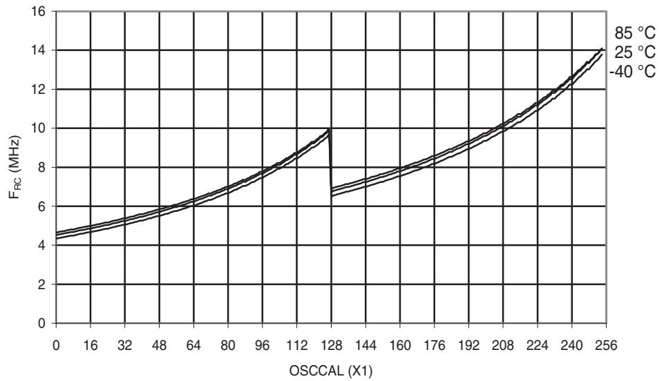
Figure 29-38. ATmega48A: Calibrated 8 MHz RC Oscillator Frequency vs. OSCCAL Value
