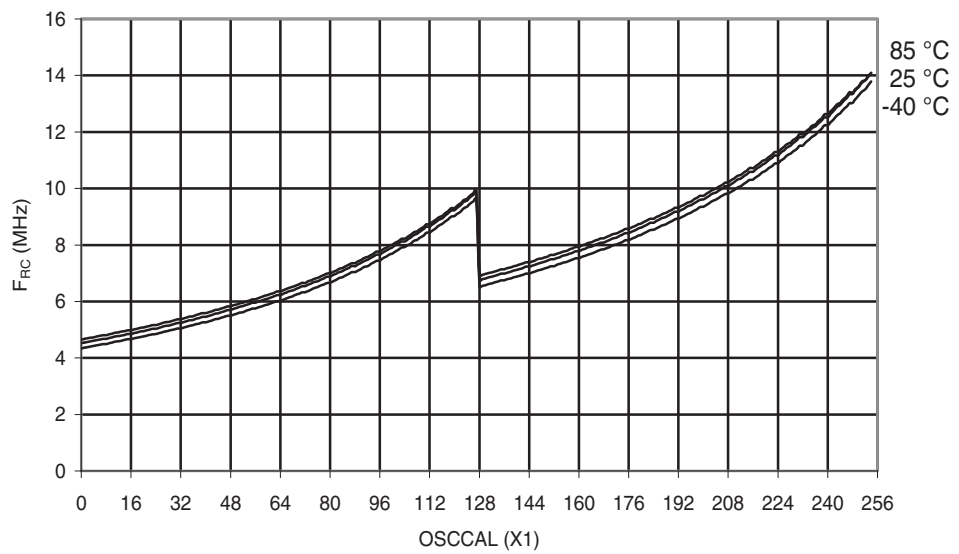
Figure 29-84. ATmega48PA: Calibrated 8 MHz RC Oscillator Frequency vs. OSCCAL Value
