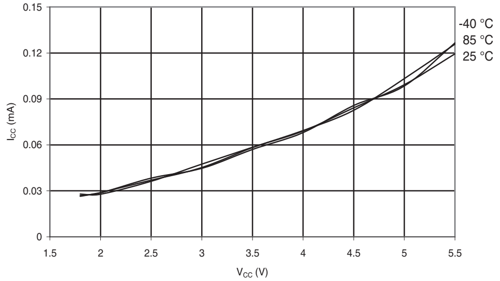
Figure 29-233. ATmega168PA: Active Supply Current vs. V_{CC} (Internal RC Oscillator, 128 kHz)
