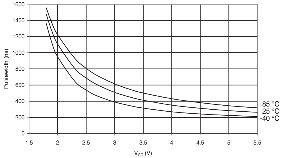
Figure 29-46. ATmega48A: Minimum Reset Pulse width vs. V_{CC}
