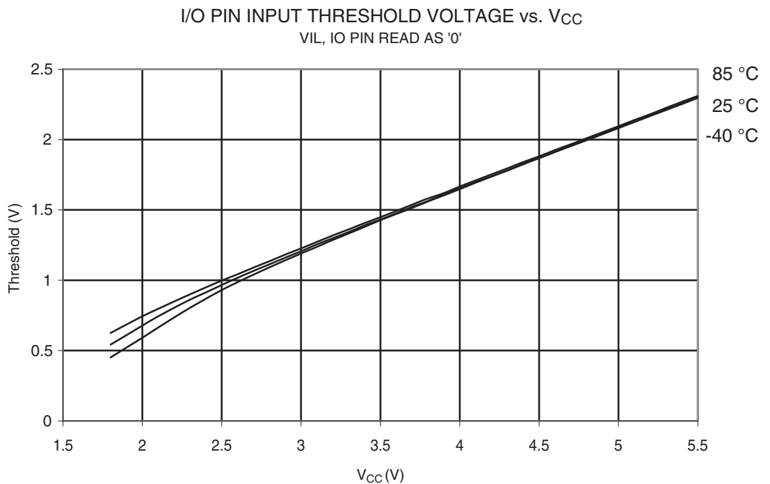
Figure 29-302. ATmega328: I/O Pin Input Threshold Voltage vs. V_{CC} ( V_{IL} , I/O Pin read as '0')
