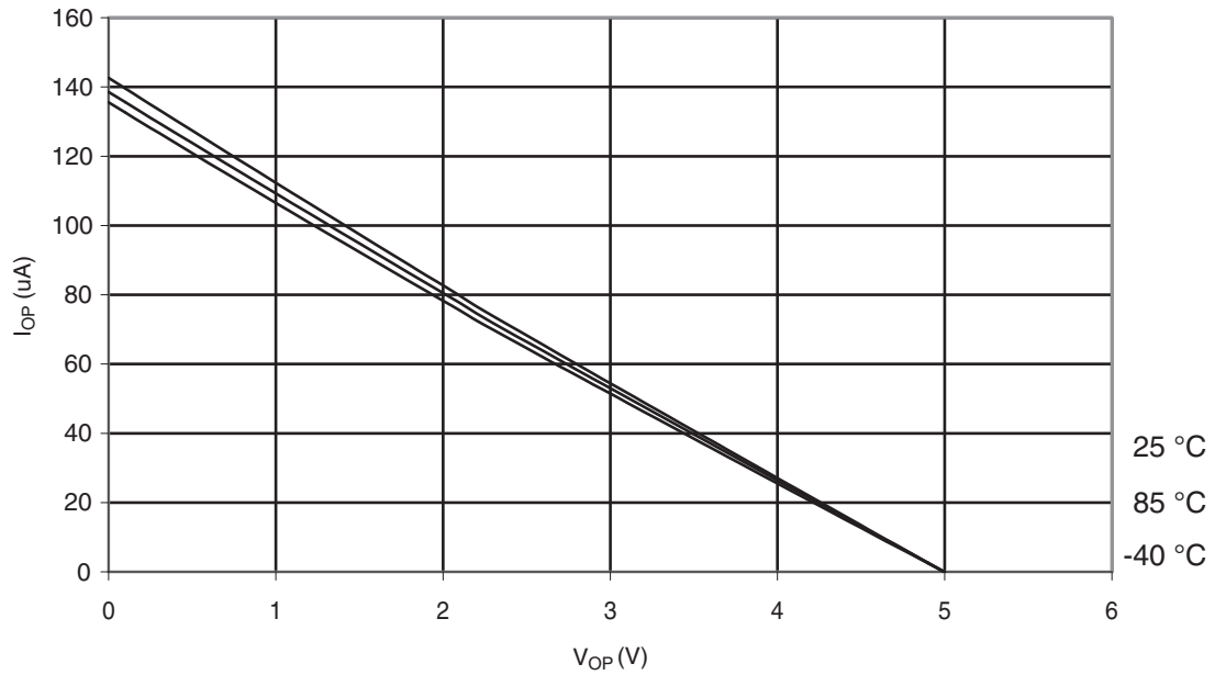
Figure 29-339. ATmega328P: I/O Pin Pull-up Resistor Current vs. Input Voltage ( V_{CC} = 5\text{ V} )
