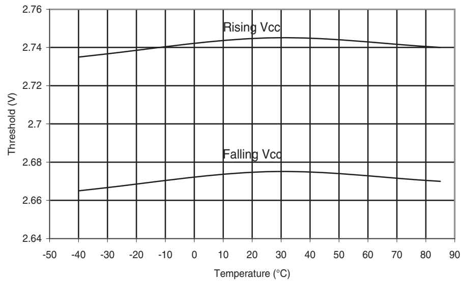
Figure 29-124. ATmega88A: BOD Thresholds vs. Temperature (BODLEVEL is 2.7 V)
