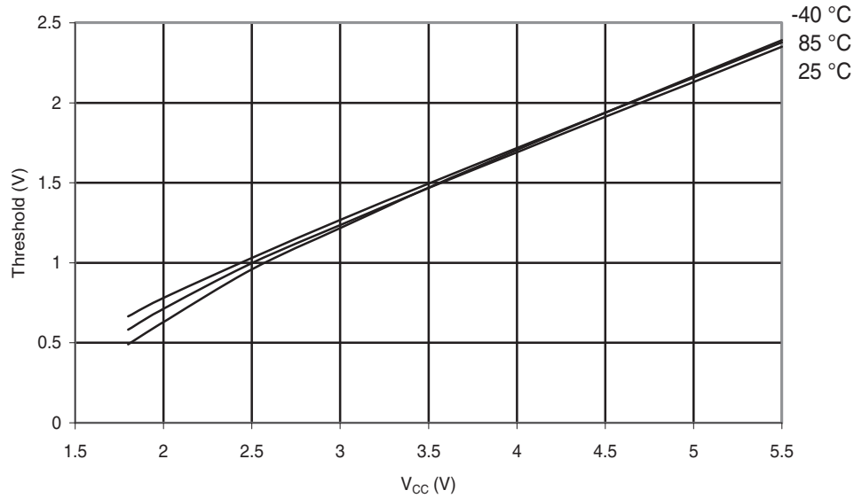
Figure 29-118. ATmega88A: I/O Pin Input Threshold Voltage vs. V_{CC} ( V_{IL} , I/O Pin read as '0')
