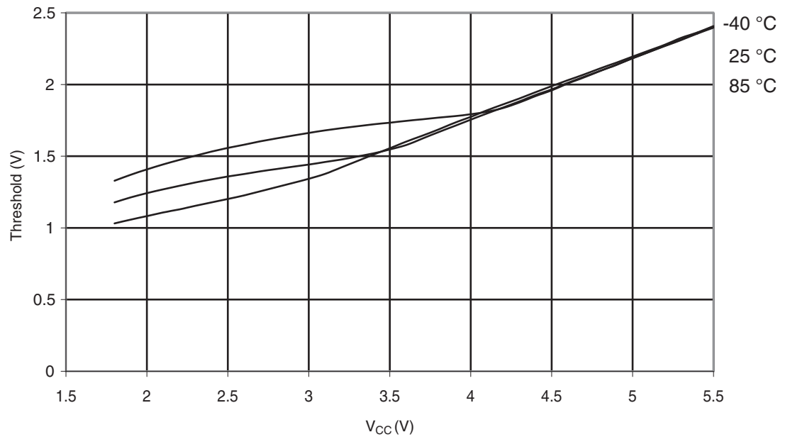
Figure 29-304. ATmega328: Reset Input Threshold Voltage vs. V_{CC} ( V_{IH} , I/O Pin read as '1')
