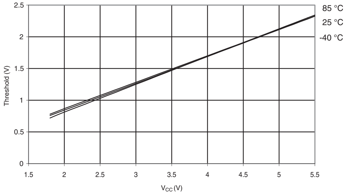
Figure 29-305. ATmega328: Reset Input Threshold Voltage vs. V_{CC} ( V_{IL} , I/O Pin read as '0')
