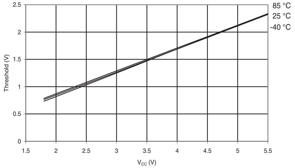
Figure 29-167. ATmega88PA: Reset Input Threshold Voltage vs. V_{CC} ( V_{IL} , I/O Pin read as '0')
