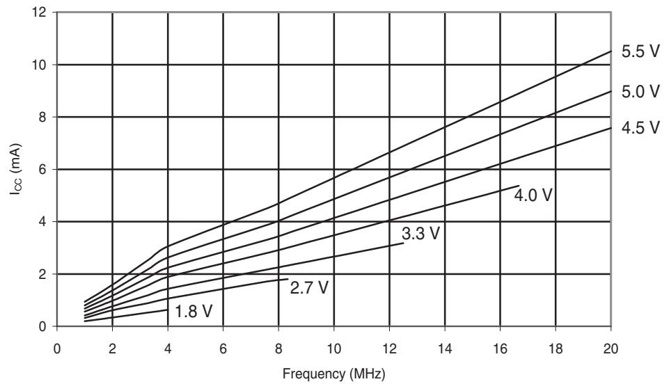
Figure 29-48. ATmega48PA: Active Supply Current vs. Frequency (1-20 MHz)
