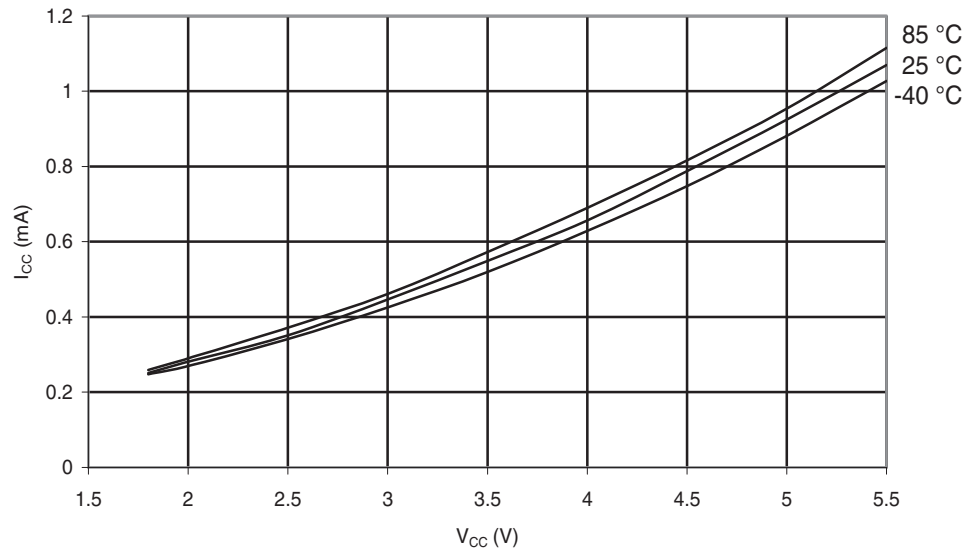
Figure 29-50. ATmega48PA: Active Supply Current vs. V_{CC} (Internal RC Oscillator, 1 MHz)
