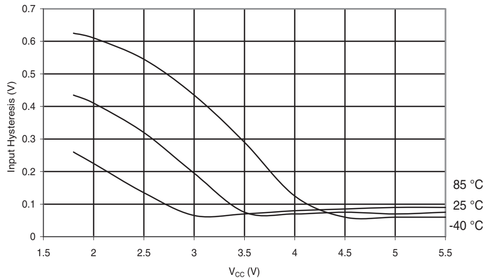
Figure 29-260. ATmega168PA: Reset Pin Input Hysteresis vs. V_{CC}
