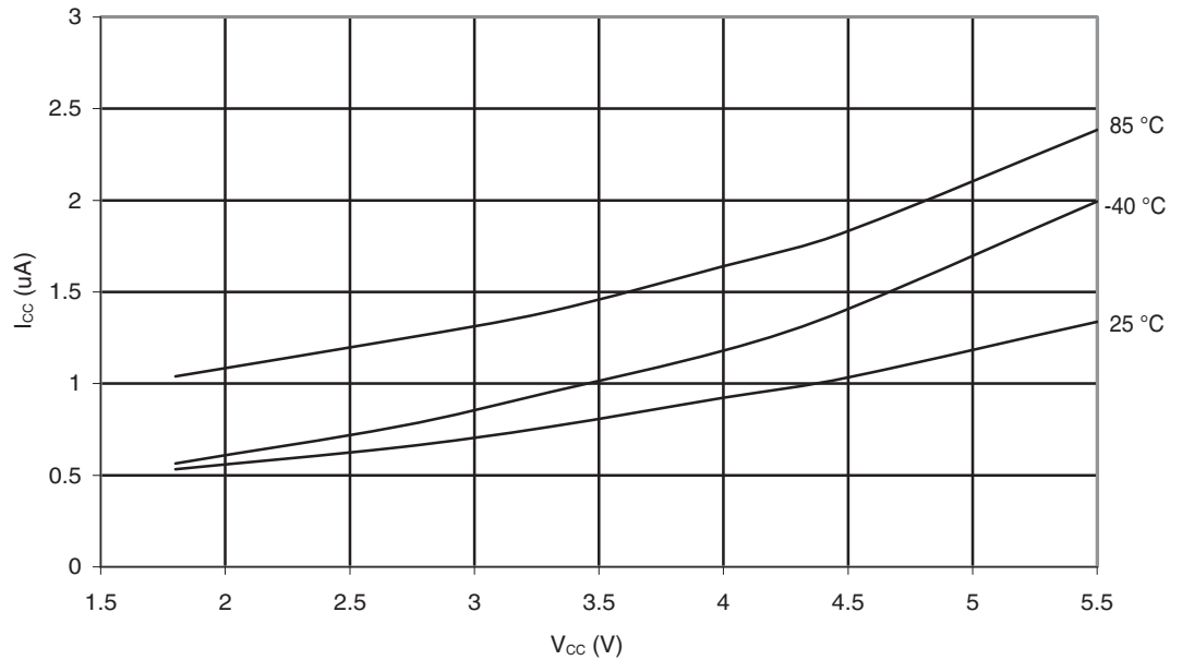
Figure 29-151. ATmega88PA: Power-Save Supply Current vs. V_{CC} (Watchdog Timer Disabled and 32 kHz Crystal Oscillator Running)
