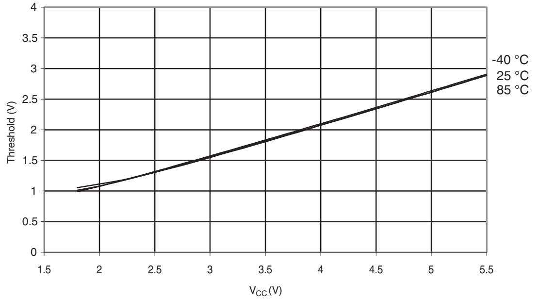
Figure 29-347. ATmega328P: I/O Pin Input Threshold Voltage vs. V_{CC} ( V_{IH} , I/O Pin read as '1')
