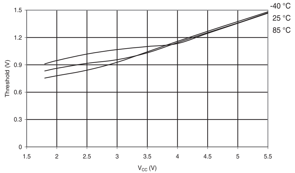
Figure 29-120. ATmega88A: Reset Input Threshold Voltage vs. V_{CC} ( V_{IH} , I/O Pin read as '1')
