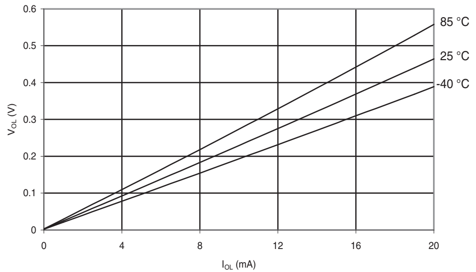
Figure 29-160. ATmega88PA: I/O Pin Output Voltage vs. Sink Current ( V_{CC} = 5\text{ V} )
