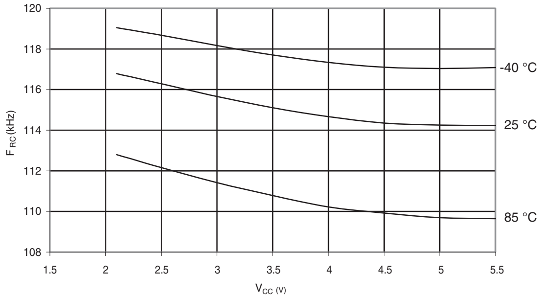
Figure 29-357. ATmega328P: Watchdog Oscillator Frequency vs. V_{CC}
