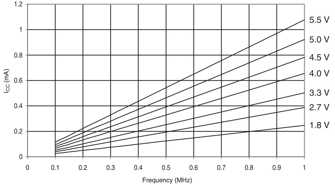
Figure 29-277. ATmega328: Active Supply Current vs. Low Frequency (0.1-1.0 MHz)
