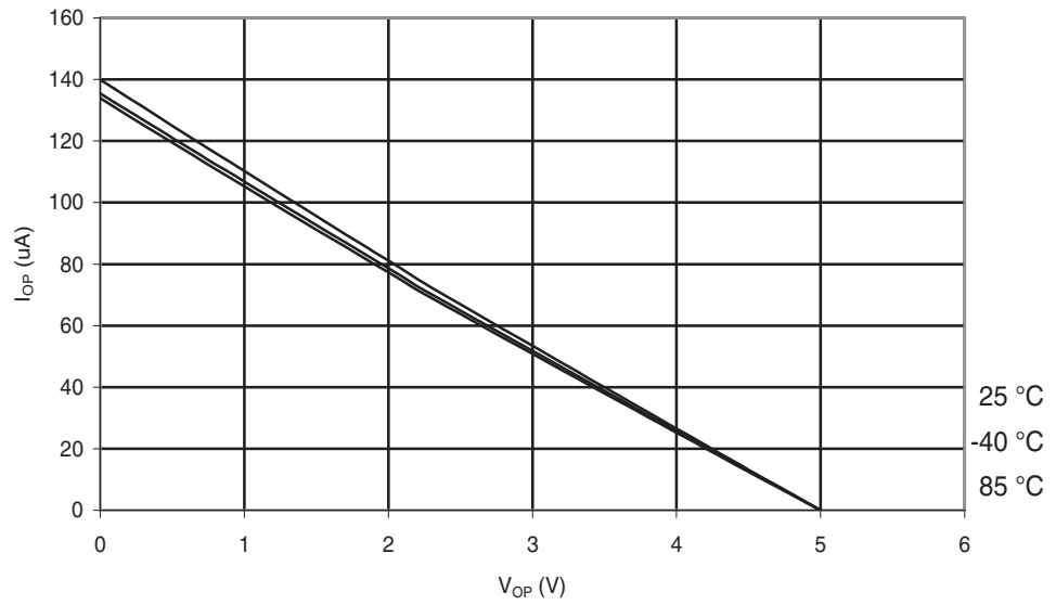
Figure 29-247. ATmega168PA: I/O Pin Pull-up Resistor Current vs. Input Voltage ( V_{CC} = 5\text{ V} )
