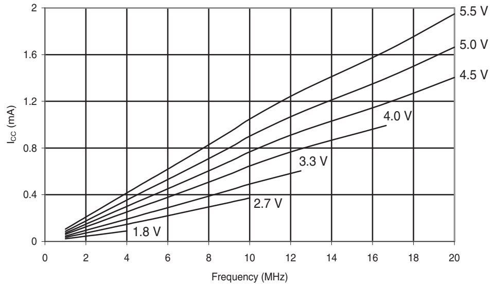
Figure 29-137. ATmega88A: Reset Supply Current vs. Frequency (1 - 20 MHz)
