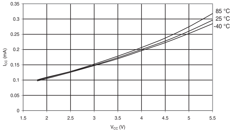
Figure 29-101. ATmega88A: Idle Supply Current vs. V_{CC} (Internal RC Oscillator, 1 MHz)
