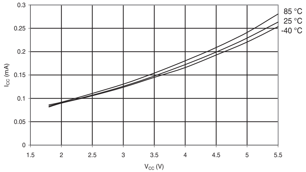
Figure 29-239. ATmega168PA: Idle Supply Current vs. V_{CC} (Internal RC Oscillator, 1 MHz)
