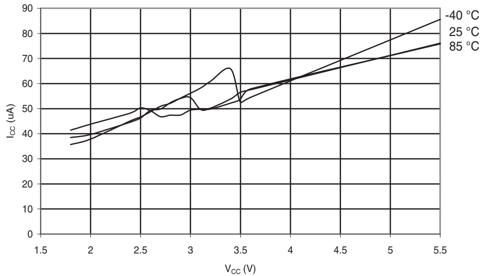
Figure 29-86. ATmega48PA: Analog Comparator Current vs. V_{CC}
