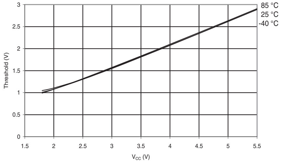
Figure 29-209. ATmega168A: I/O Pin Input Threshold Voltage vs. V_{CC} ( V_{IH} , I/O Pin read as '1')
