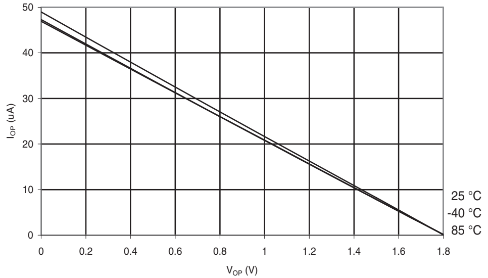
Figure 29-153. ATmega88PA: I/O Pin Pull-up Resistor Current vs. Input Voltage ( V_{CC} = 1.8\text{ V} )
