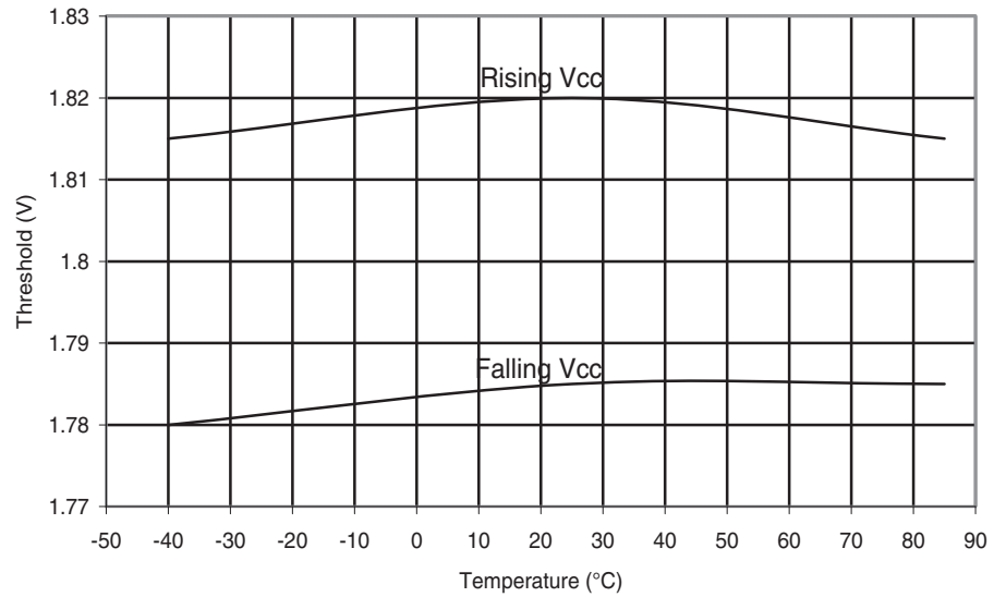
Figure 29-123. ATmega88A: BOD Thresholds vs. Temperature (BODLEVEL is 1.8 V)
