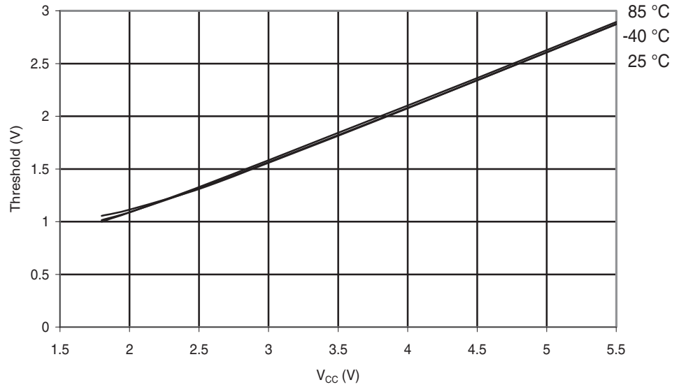
Figure 29-117. ATmega88A: I/O Pin Input Threshold Voltage vs. V_{CC} ( V_{IH} , I/O Pin read as '1')
