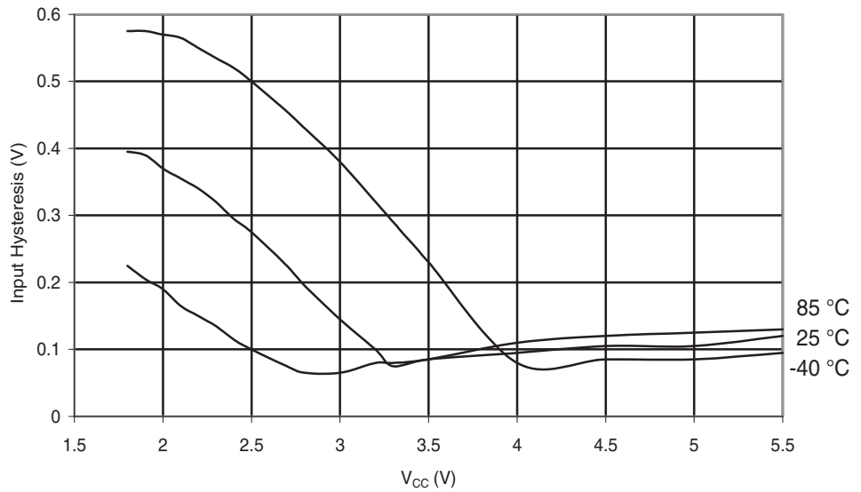
Figure 29-122. ATmega88A: Reset Pin Input Hysteresis vs. V_{CC}
