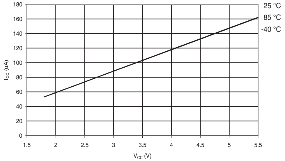
Figure 29-226. ATmega168A: Brownout Detector Current vs. V_{CC}
