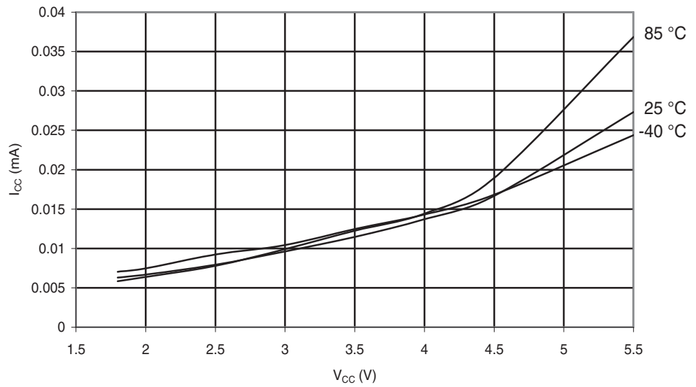
Figure 29-192. ATmega168A: Idle Supply Current vs. V_{CC} (Internal RC Oscillator, 128 kHz)
