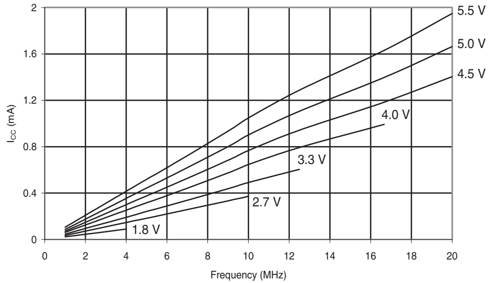
Figure 29-183. ATmega88PA: Reset Supply Current vs. Frequency (1 - 20 MHz)
