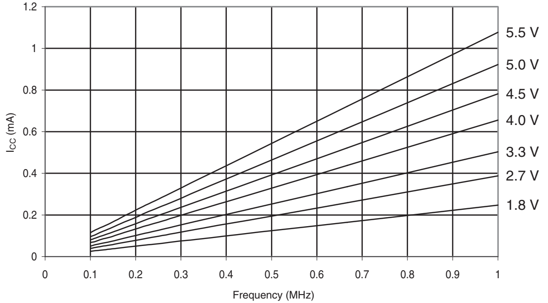
Figure 29-323. ATmega328P: Active Supply Current vs. Low Frequency (0.1-1.0 MHz)
