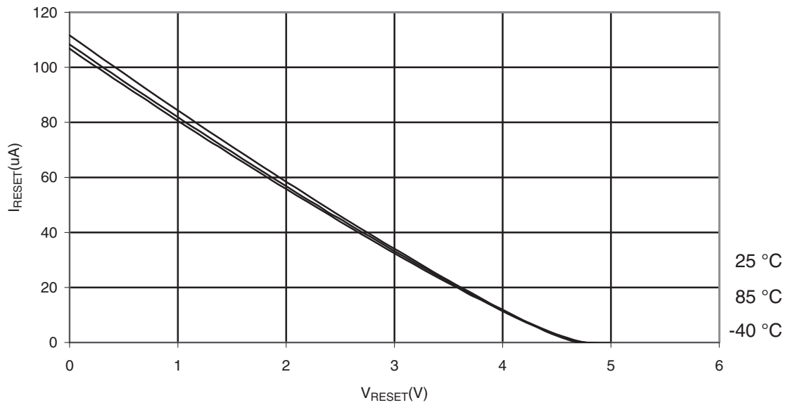
Figure 29-296. ATmega328: Reset Pull-up Resistor Current vs. Reset Pin Voltage ( V_{CC} = 5\text{ V} )
