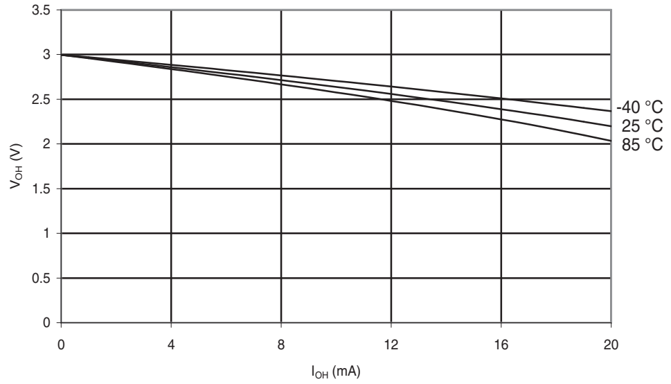
Figure 29-115. ATmega88A: I/O Pin Output Voltage vs. Source Current ( V_{CC} = 3\text{ V} )
