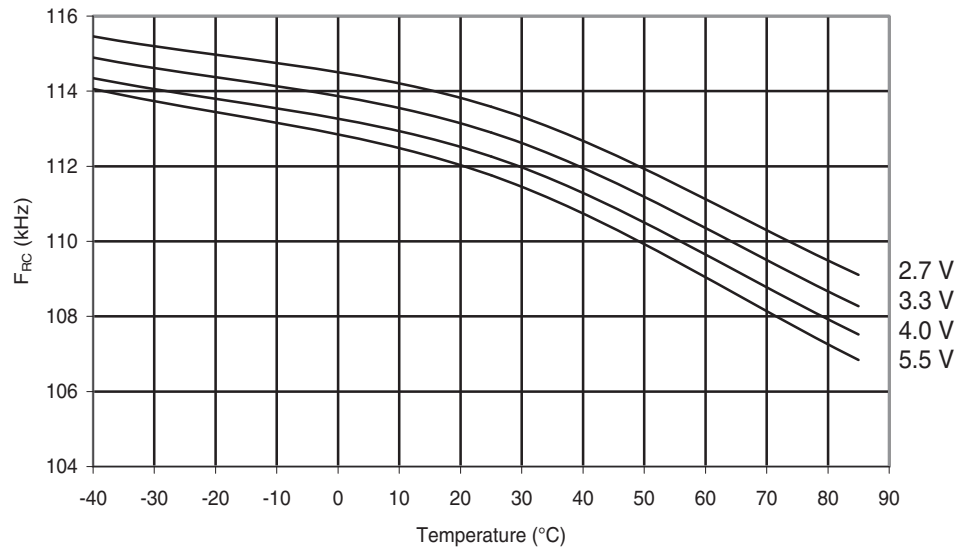
Figure 29-80. ATmega48PA: Watchdog Oscillator Frequency vs. Temperature
