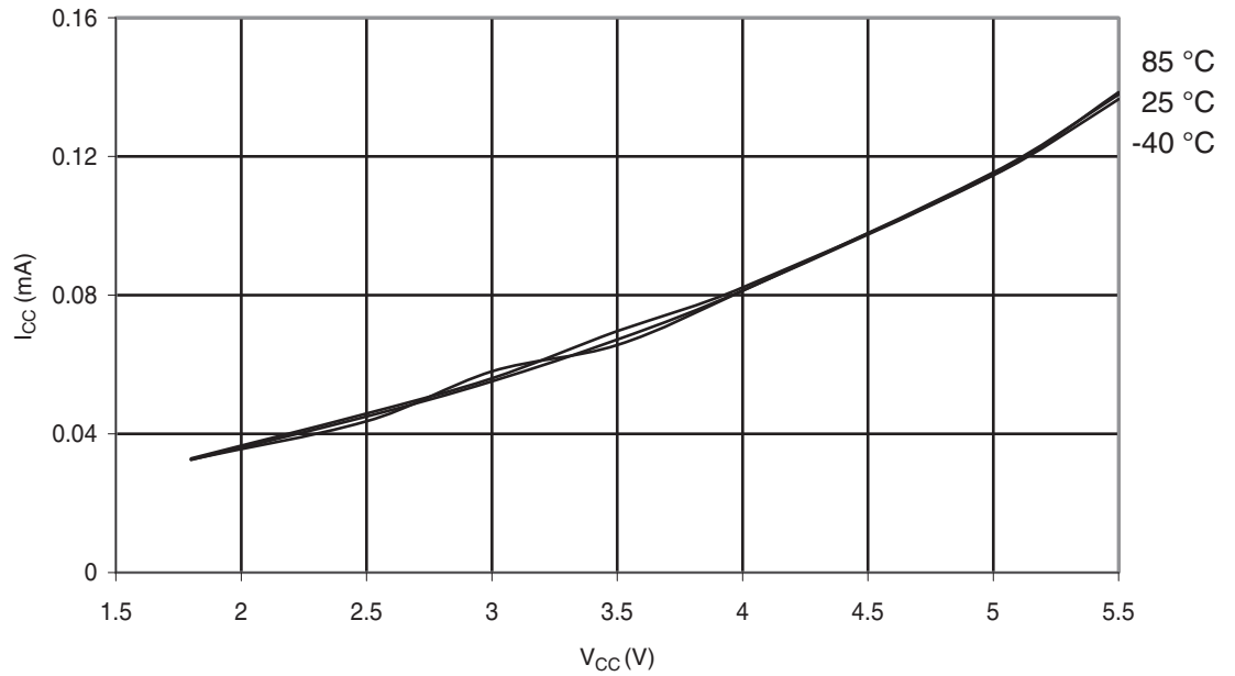
Figure 29-279. ATmega328: Active Supply Current vs. V_{CC} (Internal RC Oscillator, 128 kHz)
