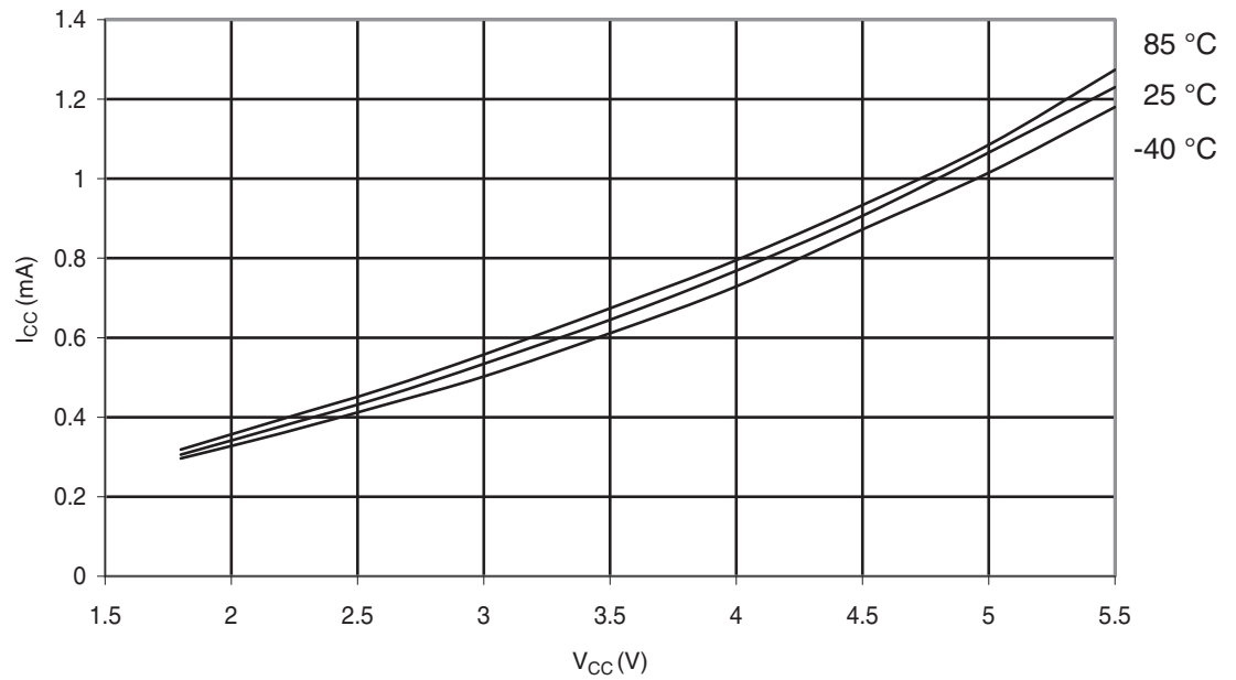
Figure 29-280. ATmega328: Active Supply Current vs. V_{CC} (Internal RC Oscillator, 1 MHz)
