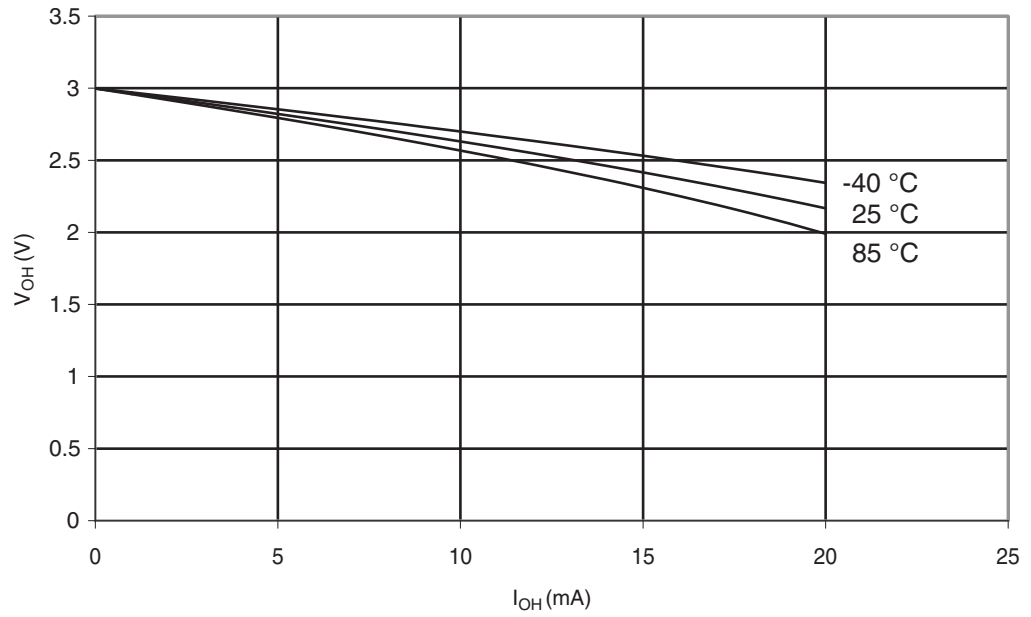
Figure 29-299. ATmega328: I/O Pin Output Voltage vs. Source Current ( V_{CC} = 3\text{ V} )
