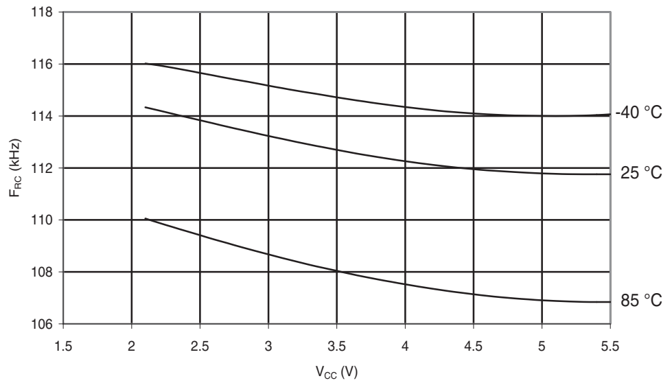
Figure 29-81. ATmega48PA: Watchdog Oscillator Frequency vs. V_{CC}
