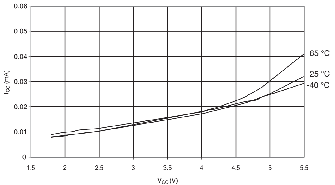
Figure 29-284. ATmega328: Idle Supply Current vs. V_{CC} (Internal RC Oscillator, 128 kHz)
