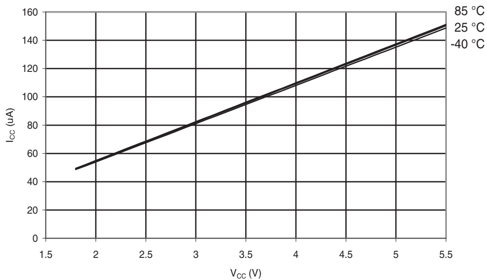
Figure 29-133. ATmega88A: AREF External Reference Current vs. V_{CC}
