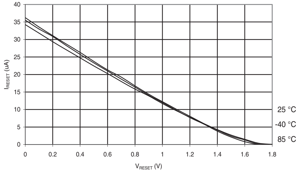
Figure 29-156. ATmega88PA: Reset Pull-up Resistor Current vs. Reset Pin Voltage ( V_{CC} = 1.8\text{ V} )
