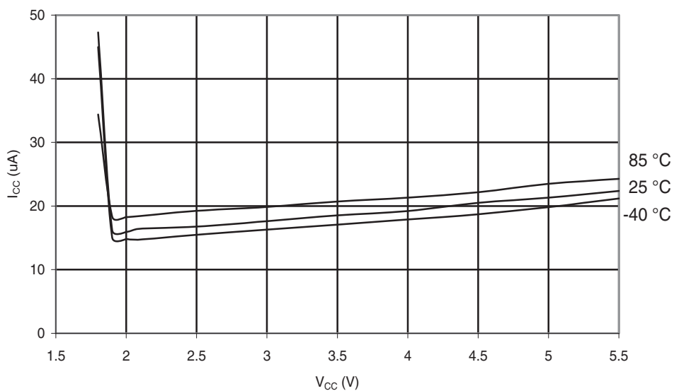
Figure 29-180. ATmega88PA: Brownout Detector Current vs. V_{CC}
