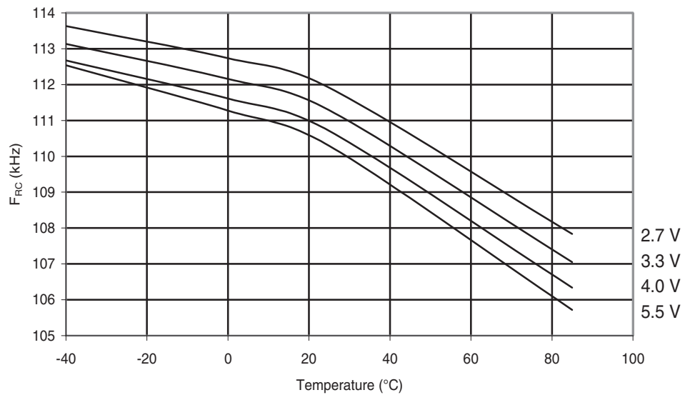
Figure 29-126. ATmega88A: Watchdog Oscillator Frequency vs. Temperature
