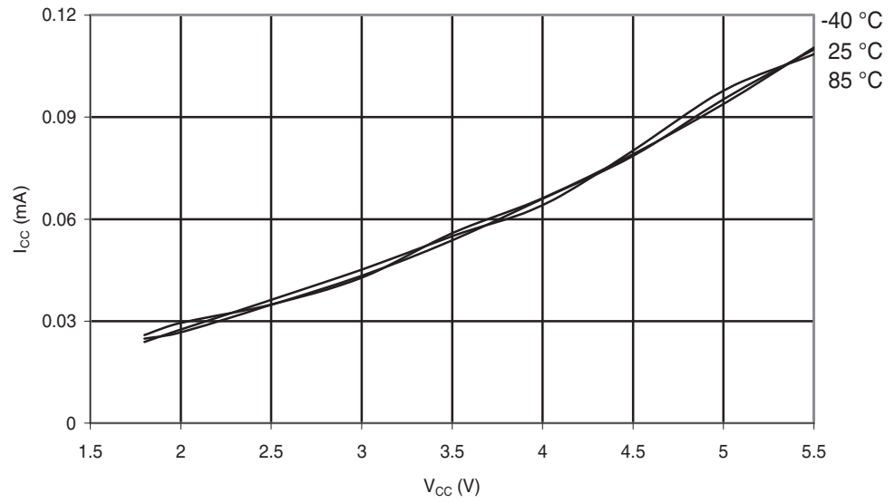
Figure 29-141. ATmega88PA: Active Supply Current vs. V_{CC} (Internal RC Oscillator, 128 kHz)
