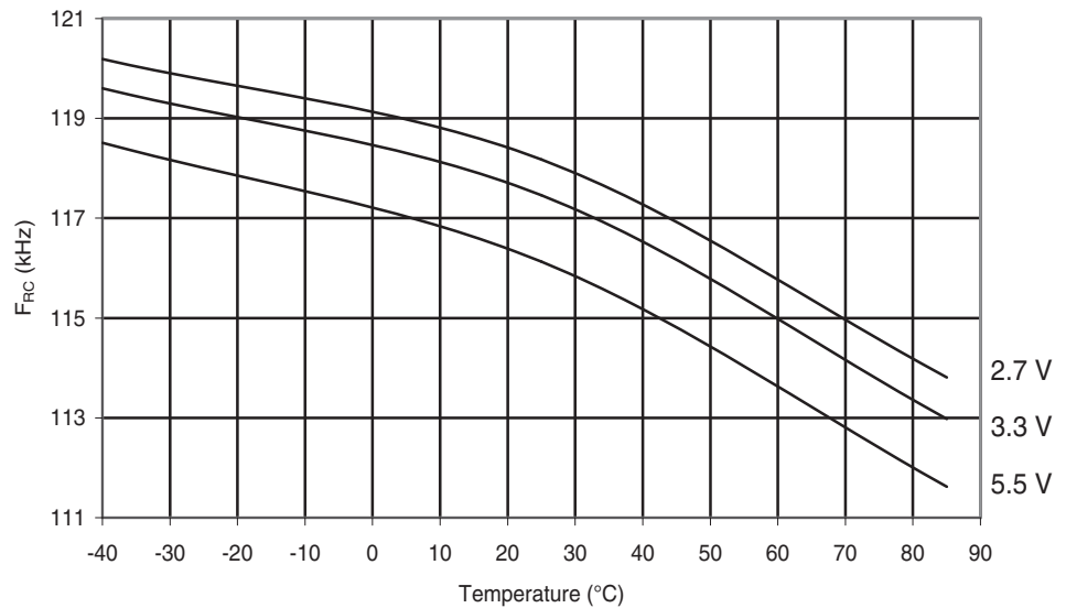
Figure 29-264. ATmega168PA: Watchdog Oscillator Frequency vs. Temperature
