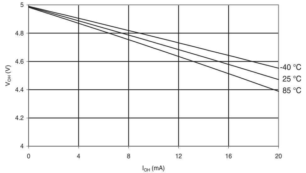
Figure 29-254. ATmega168PA: I/O Pin Output Voltage vs. Source Current ( V_{CC} = 5\text{ V} )
