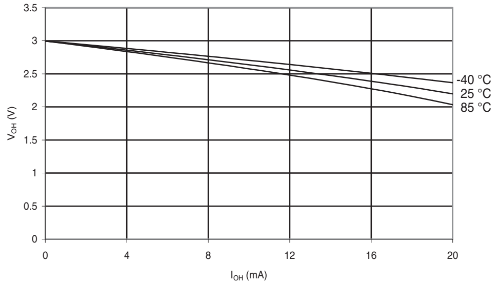
Figure 29-161. ATmega88PA: I/O Pin Output Voltage vs. Source Current ( V_{CC} = 3\text{ V} )
