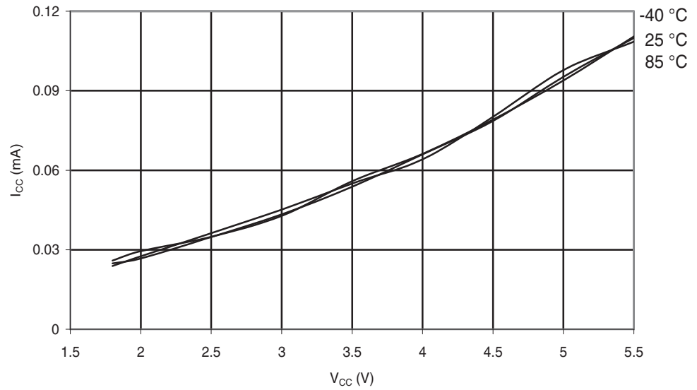
Figure 29-95. ATmega88A: Active Supply Current vs. V_{CC} (Internal RC Oscillator, 128 kHz)
