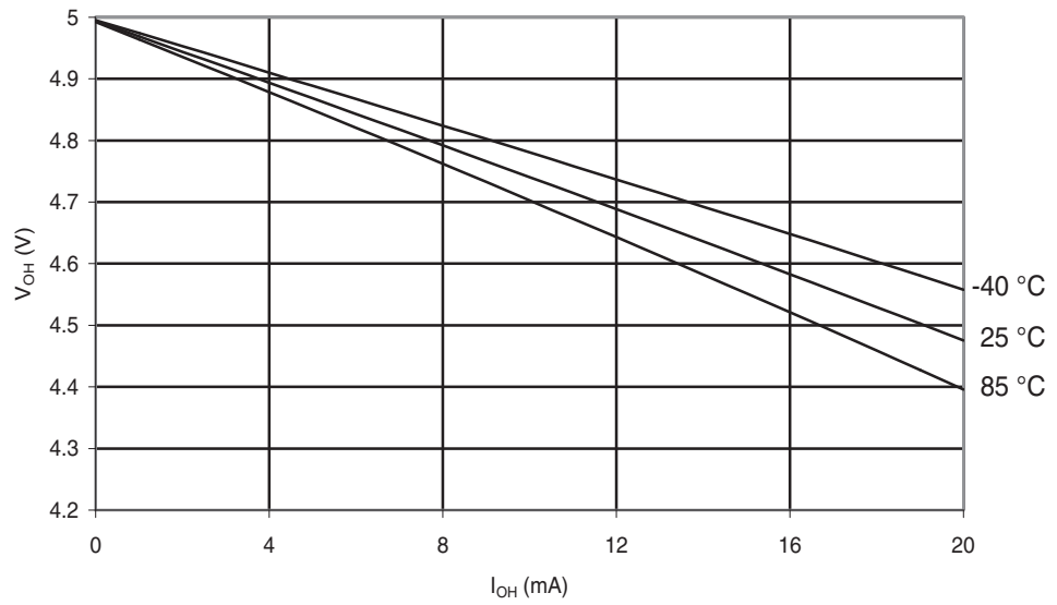
Figure 29-116. ATmega88A: I/O Pin Output Voltage vs. Source Current ( V_{CC} = 5\text{ V} )
