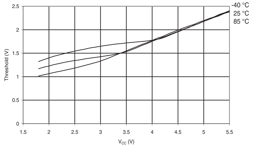
Figure 29-74. ATmega48PA: Reset Input Threshold Voltage vs. V_{CC} ( V_{IH} , I/O Pin read as '1')
