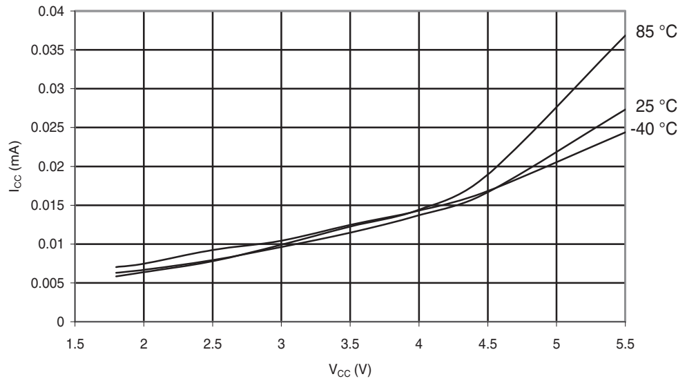
Figure 29-238. ATmega168PA: Idle Supply Current vs. V_{CC} (Internal RC Oscillator, 128 kHz)
