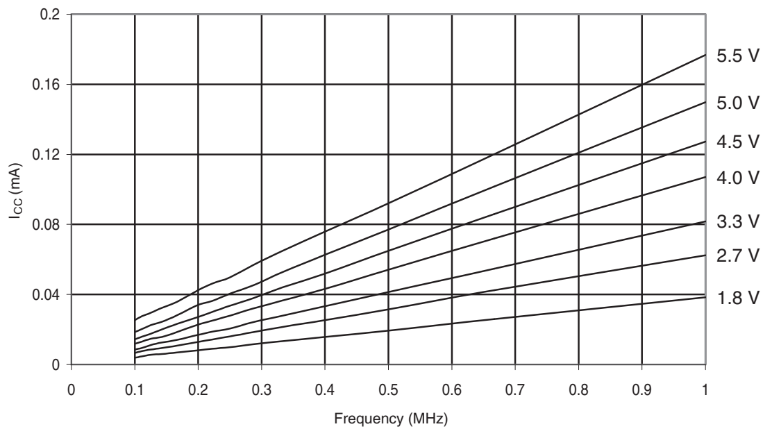
Figure 29-328. ATmega328P: Idle Supply Current vs. Low Frequency (0.1-1.0 MHz)
