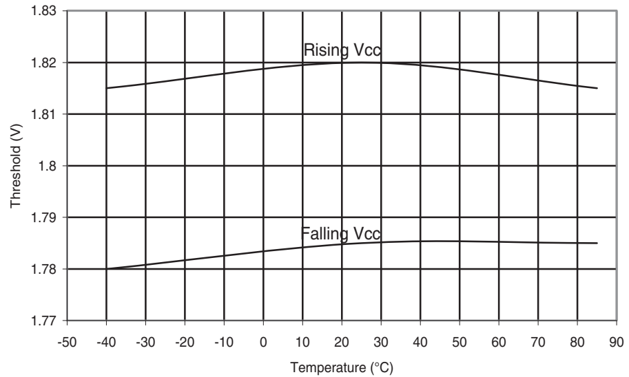
Figure 29-169. ATmega88PA: BOD Thresholds vs. Temperature (BODLEVEL is 1.8 V)
