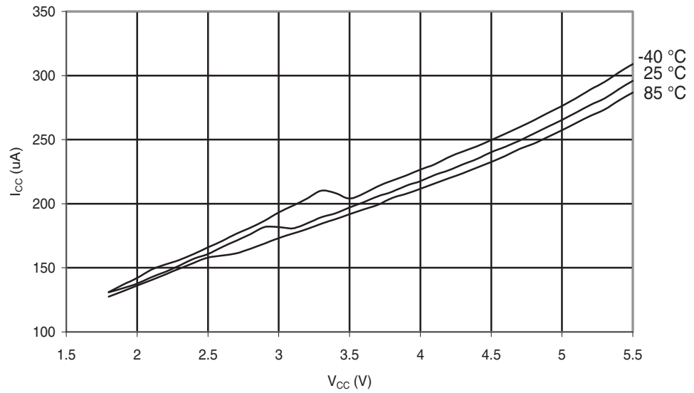
Figure 29-269. ATmega168PA: ADC Current vs. V_{CC} (AREF = AV_{CC} )
