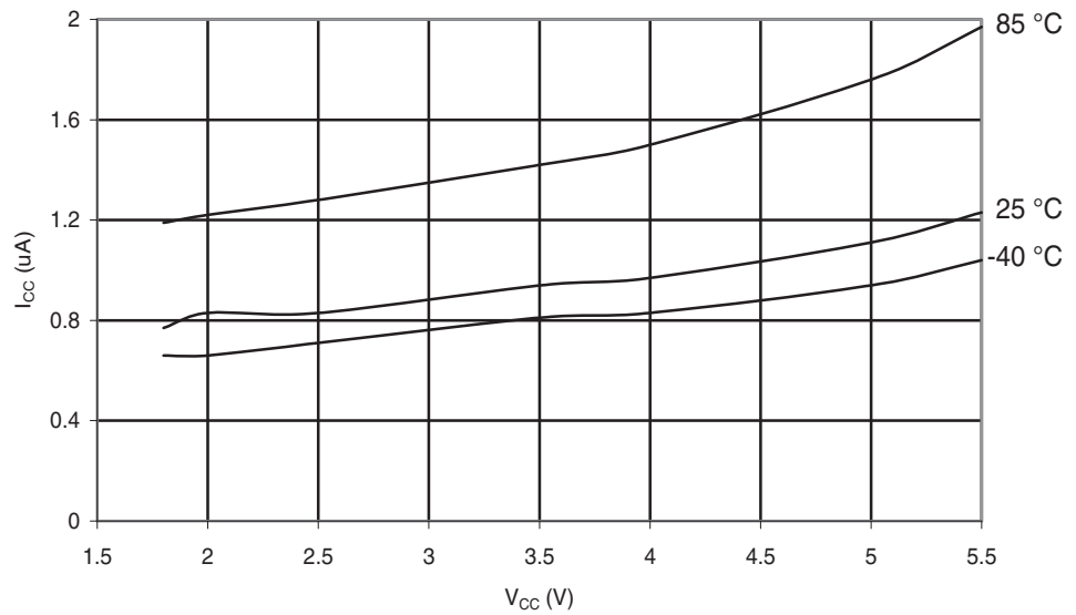
Figure 29-59. ATmega48PA: Power-Save Supply Current vs. V_{CC} (Watchdog Timer Disabled and 32 kHz Crystal Oscillator Running)
