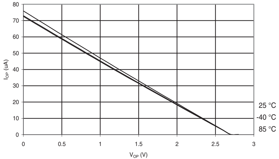
Figure 29-108. ATmega88A: I/O Pin Pull-up Resistor Current vs. Input Voltage ( V_{CC} = 2.7\text{ V} )
