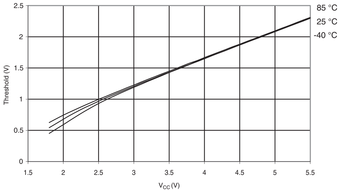
Figure 29-348. ATmega328P: I/O Pin Input Threshold Voltage vs. V_{CC} ( V_{IL} , I/O Pin read as '0')
