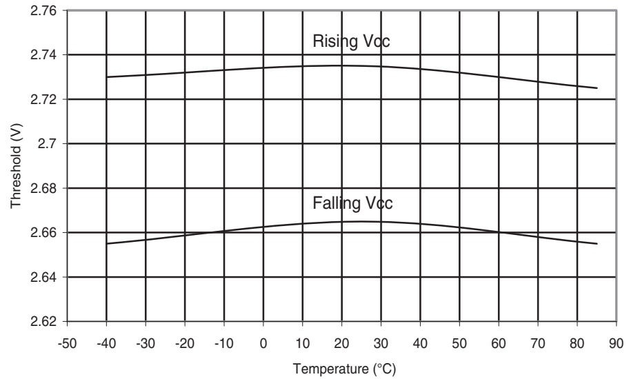
Figure 29-262. ATmega168PA: BOD Thresholds vs. Temperature (BODLEVEL is 2.7 V)
