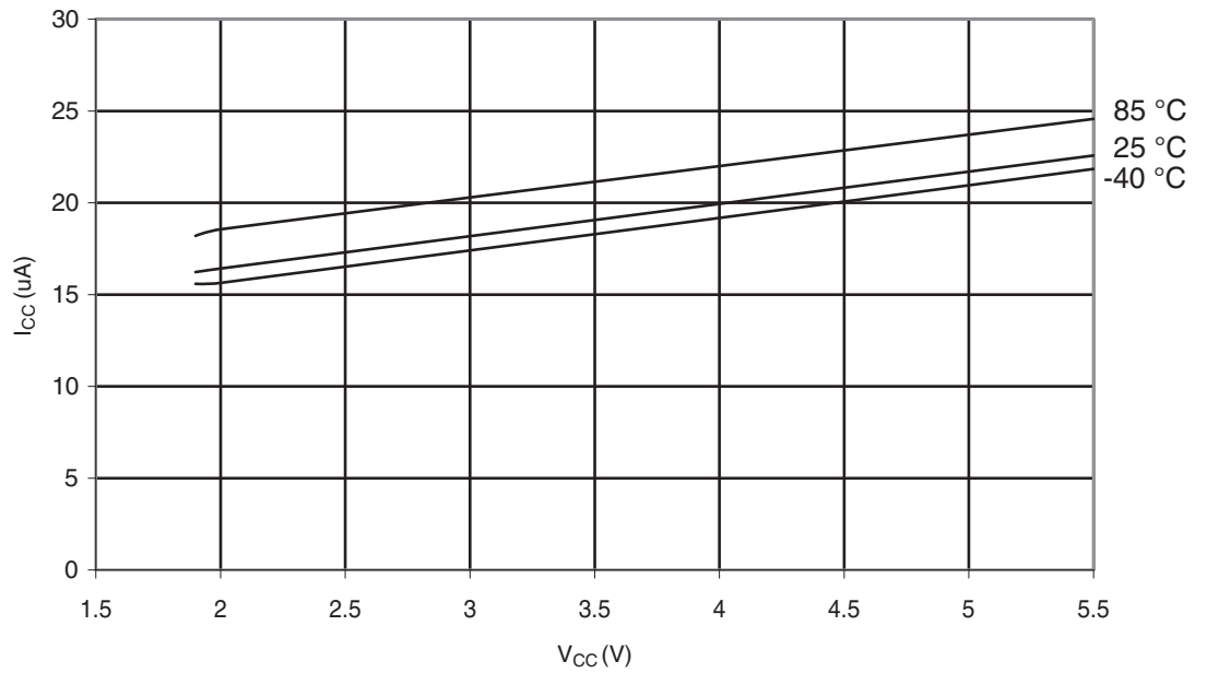
Figure 29-318. ATmega328: Brownout Detector Current vs. V_{CC}
