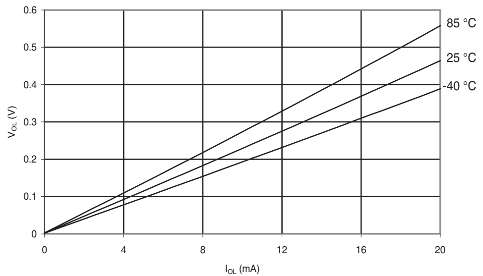
Figure 29-114. ATmega88A: I/O Pin Output Voltage vs. Sink Current ( V_{CC} = 5\text{ V} )
