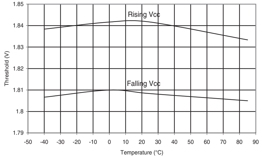
Figure 29-77. ATmega48PA: BOD Thresholds vs. Temperature (BODLEVEL is 1.8 V)
