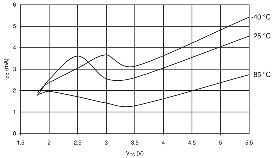
Figure 29-89. ATmega48PA: Programming Current vs. V_{CC}
