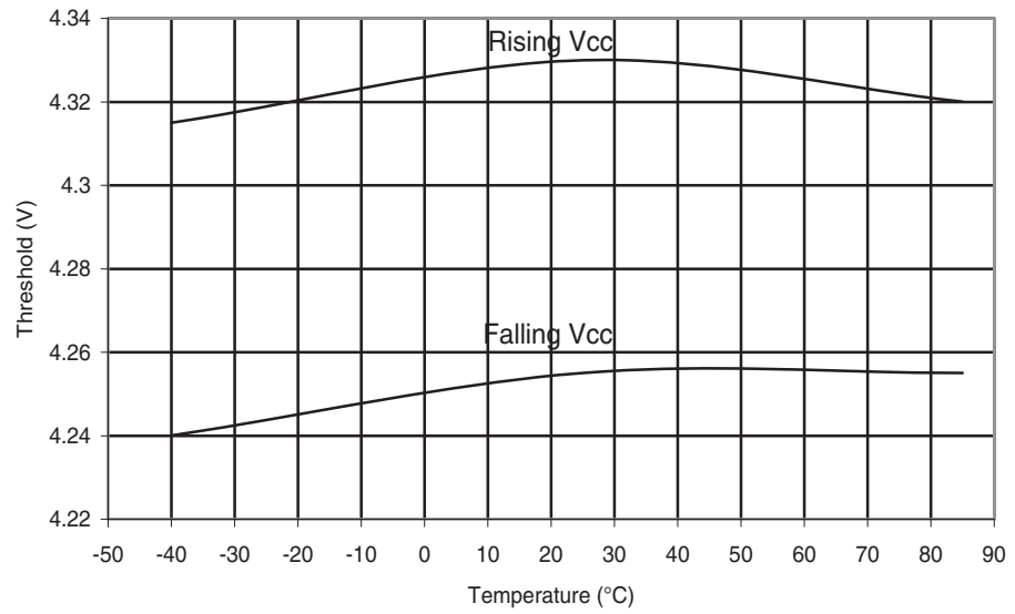
Figure 29-125. ATmega88A: BOD Thresholds vs. Temperature (BODLEVEL is 4.3 V)
