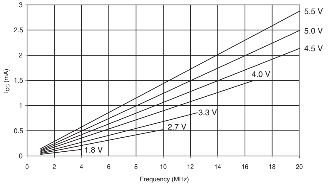
Figure 29-321. ATmega328: Reset Supply Current vs. Frequency (1 - 20 MHz)
