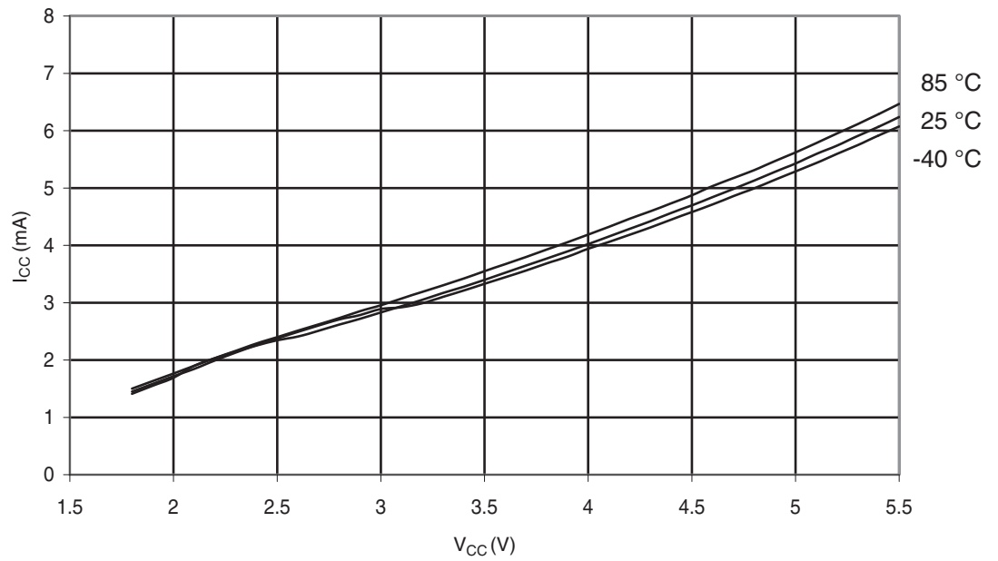
Figure 29-327. ATmega328P: Active Supply Current vs. V_{CC} (Internal RC Oscillator, 8 MHz)
