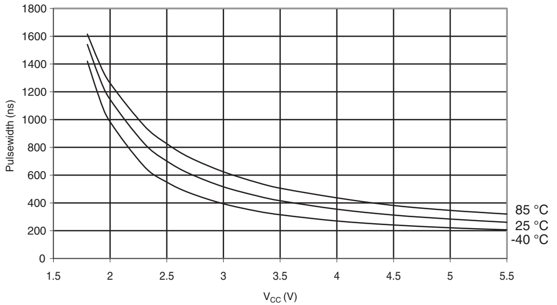
Figure 29-322. ATmega328: Minimum Reset Pulse width vs. V_{CC}
