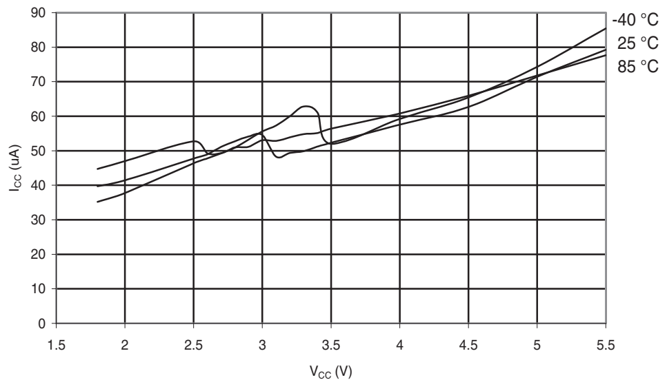
Figure 29-178. ATmega88PA: Analog Comparator Current vs. V_{CC}
