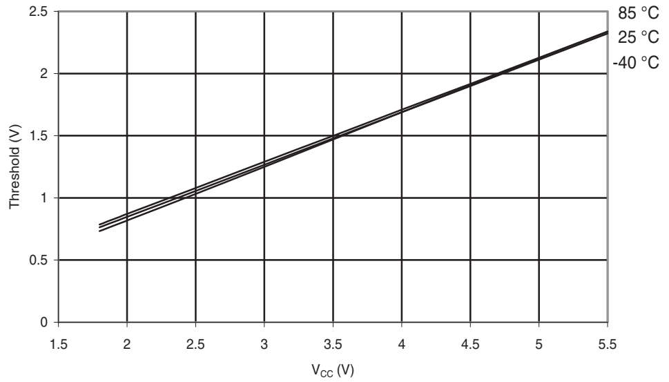
Figure 29-121. ATmega88A: Reset Input Threshold Voltage vs. V_{CC} ( V_{IL} , I/O Pin read as '0')
