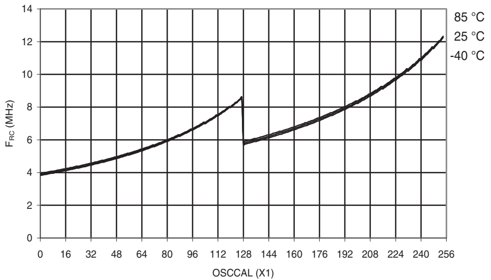
Figure 29-130. ATmega88A: Calibrated 8 MHz RC Oscillator Frequency vs. OSCCAL Value
