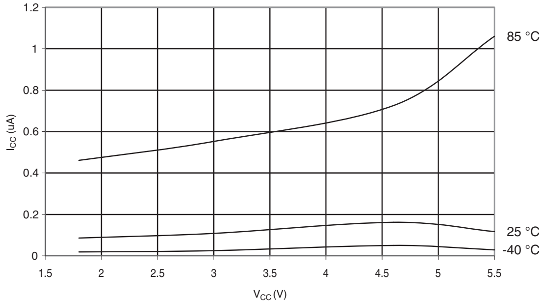
Figure 29-333. ATmega328P: Power-Down Supply Current vs. V_{CC} (Watchdog Timer Disabled)
