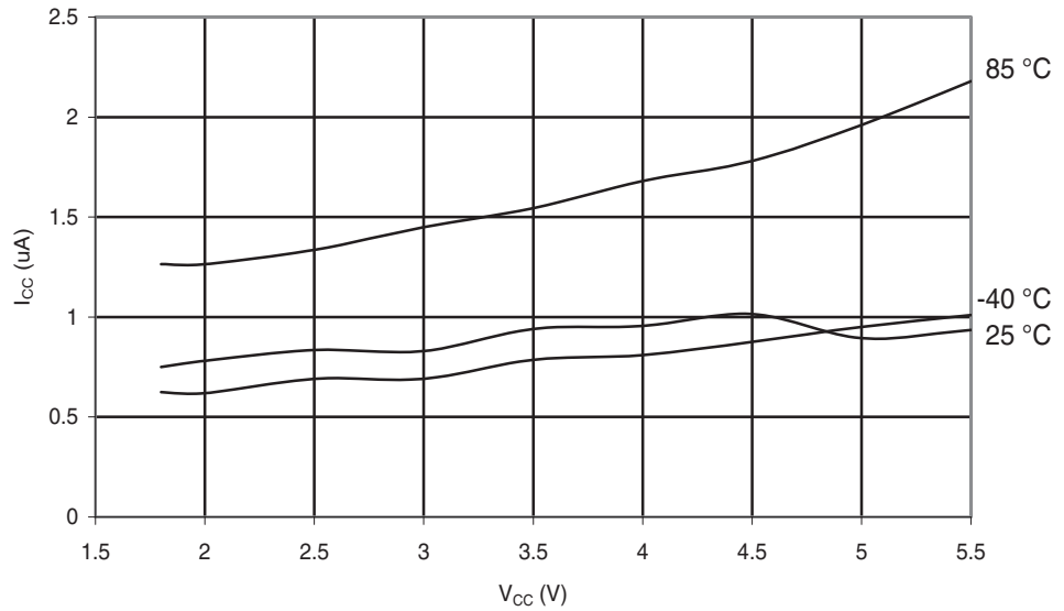
Figure 29-243. ATmega168PA: Power-Save Supply Current vs. V_{CC} (Watchdog Timer Disabled and 32 kHz Crystal Oscillator Running)
