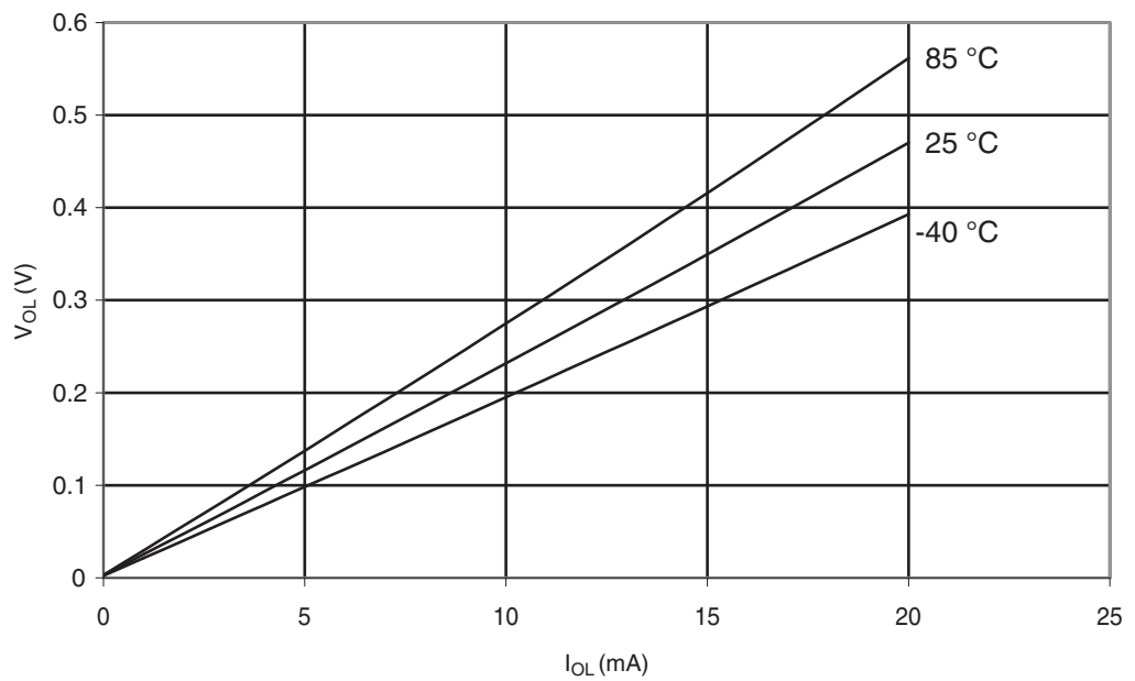
Figure 29-298. ATmega328: I/O Pin Output Voltage vs. Sink Current ( V_{CC} = 5\text{ V} )
