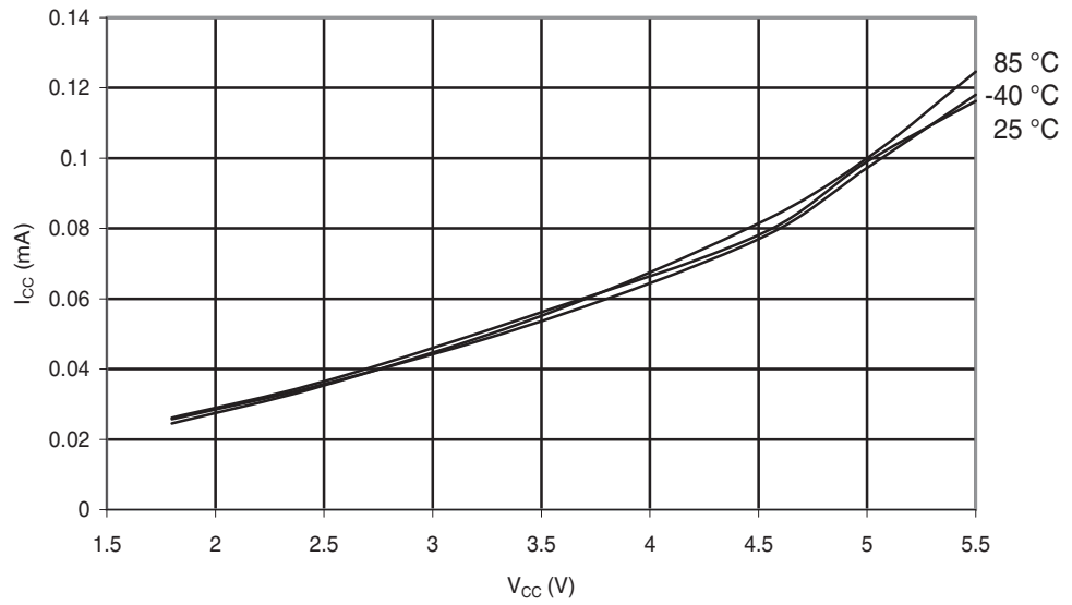
Figure 29-49. ATmega48PA: Active Supply Current vs. V_{CC} (Internal RC Oscillator, 128 kHz)
