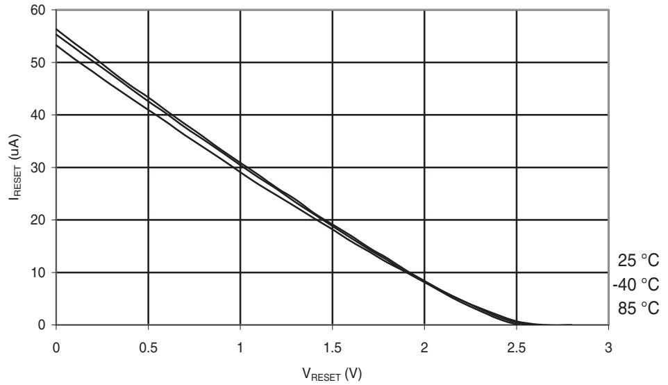
Figure 29-203. ATmega168A: Reset Pull-up Resistor Current vs. Reset Pin Voltage ( V_{CC} = 2.7\text{ V} )
