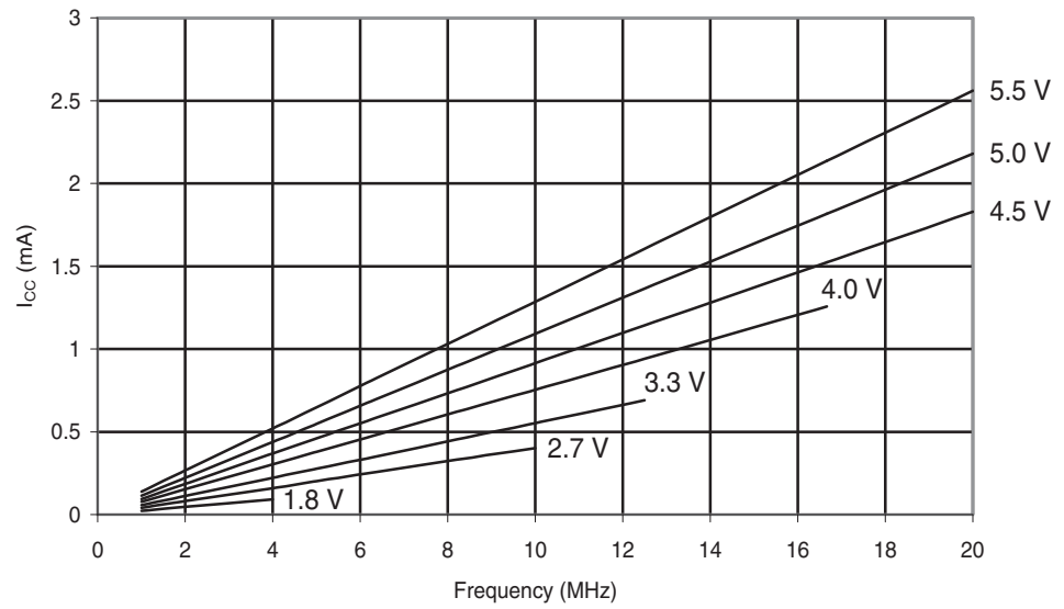
Figure 29-191. ATmega168A: Idle Supply Current vs. Frequency (1-20 MHz)
