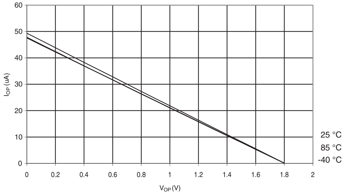
Figure 29-337. ATmega328P: I/O Pin Pull-up Resistor Current vs. Input Voltage ( V_{CC} = 1.8\text{ V} )
