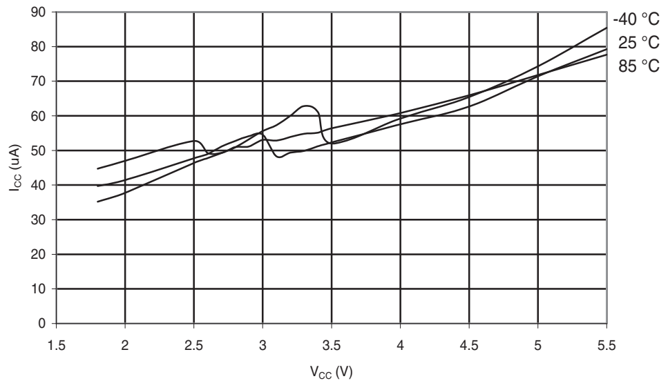
Figure 29-132. ATmega88A: Analog Comparator Current vs. V_{CC}
