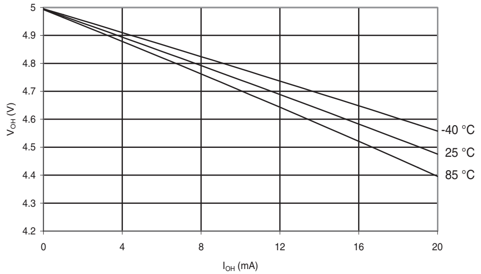
Figure 29-162. ATmega88PA: I/O Pin Output Voltage vs. Source Current ( V_{CC} = 5\text{ V} )
