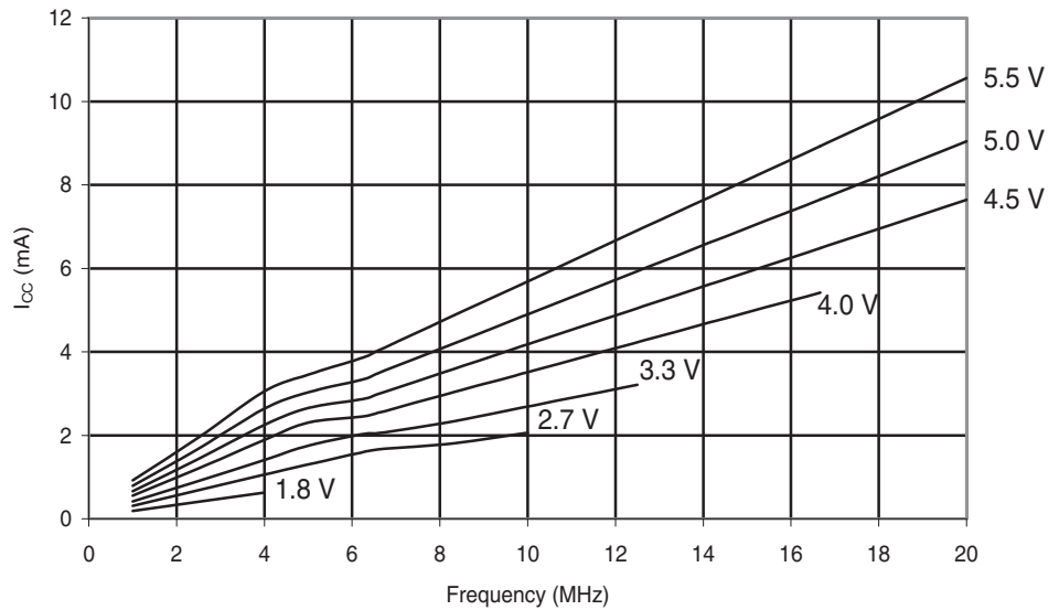
Figure 29-186. ATmega168A: Active Supply Current vs. Frequency (1-20 MHz)
