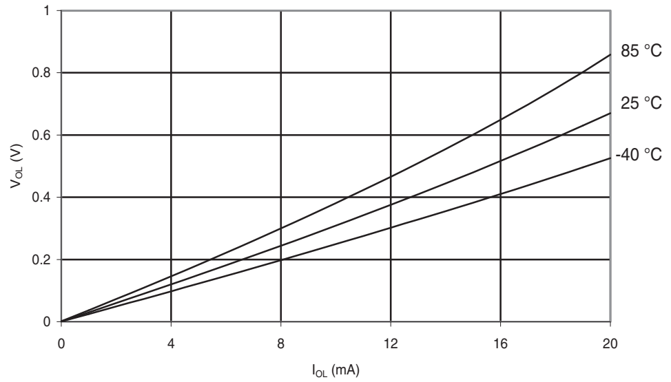
Figure 29-113. ATmega88A: I/O Pin Output Voltage vs. Sink Current ( V_{CC} = 3\text{ V} )
