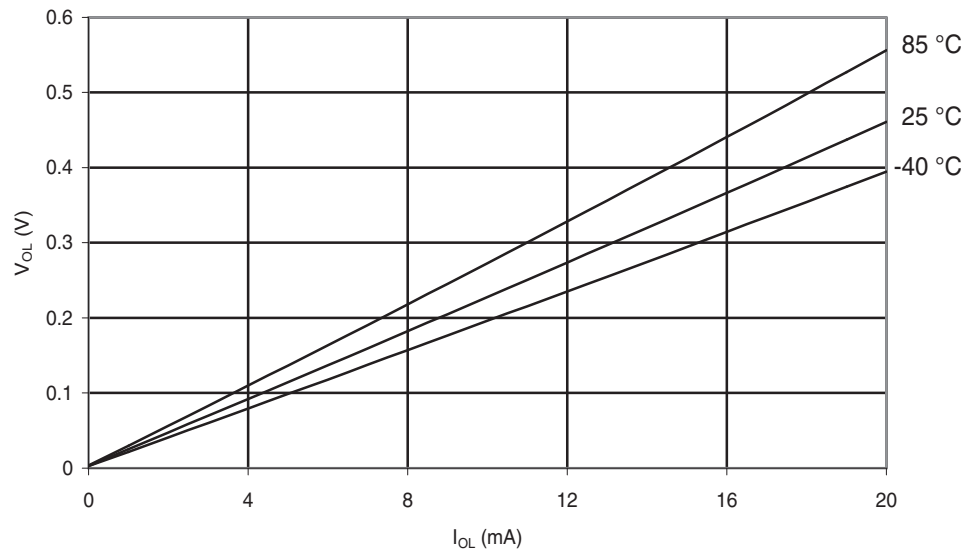
Figure 29-252. ATmega168PA: I/O Pin Output Voltage vs. Sink Current ( V_{CC} = 5\text{ V} )
