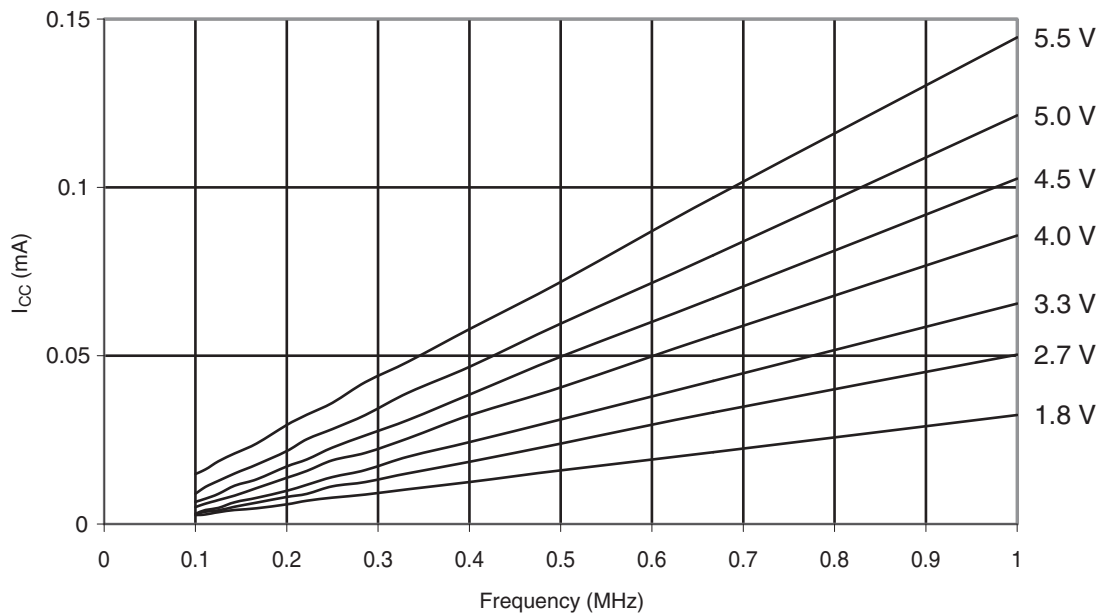
Figure 29-320. ATmega328: Reset Supply Current vs. Low Frequency (0.1 - 1.0 MHz)
