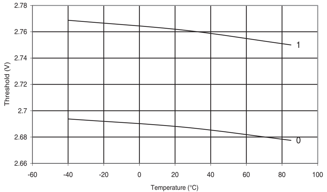
Figure 29-308. ATmega328: BOD Thresholds vs. Temperature (BODLEVEL is 2.7 V)
