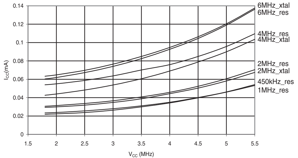
Figure 29-198. ATmega168A: Standby Supply Current vs. V_{CC} (Watchdog Timer Disabled)
