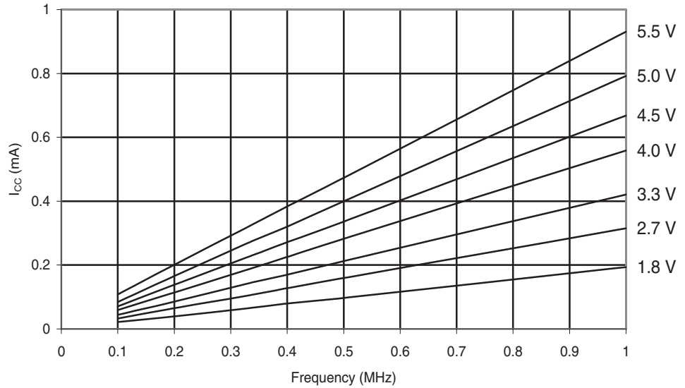
Figure 29-93. ATmega88A: Active Supply Current vs. Low Frequency (0.1-1.0 MHz)
