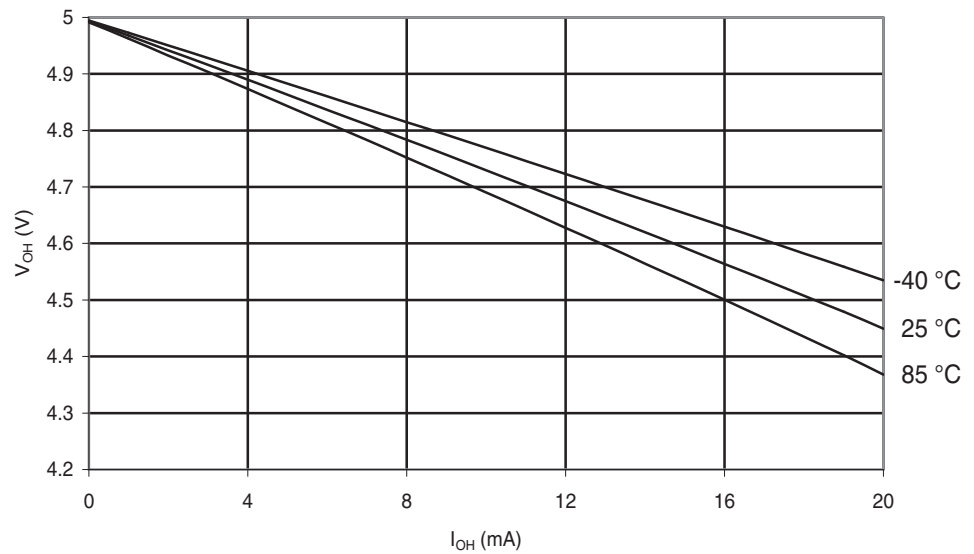
Figure 29-70. ATmega48PA: I/O Pin Output Voltage vs. Source Current ( V_{CC} = 5\text{ V} )
