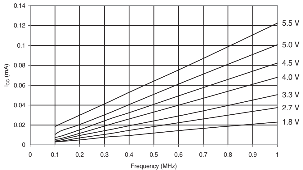
Figure 29-90. ATmega48PA: Reset Supply Current vs. Low Frequency (0.1 - 1.0 MHz)
