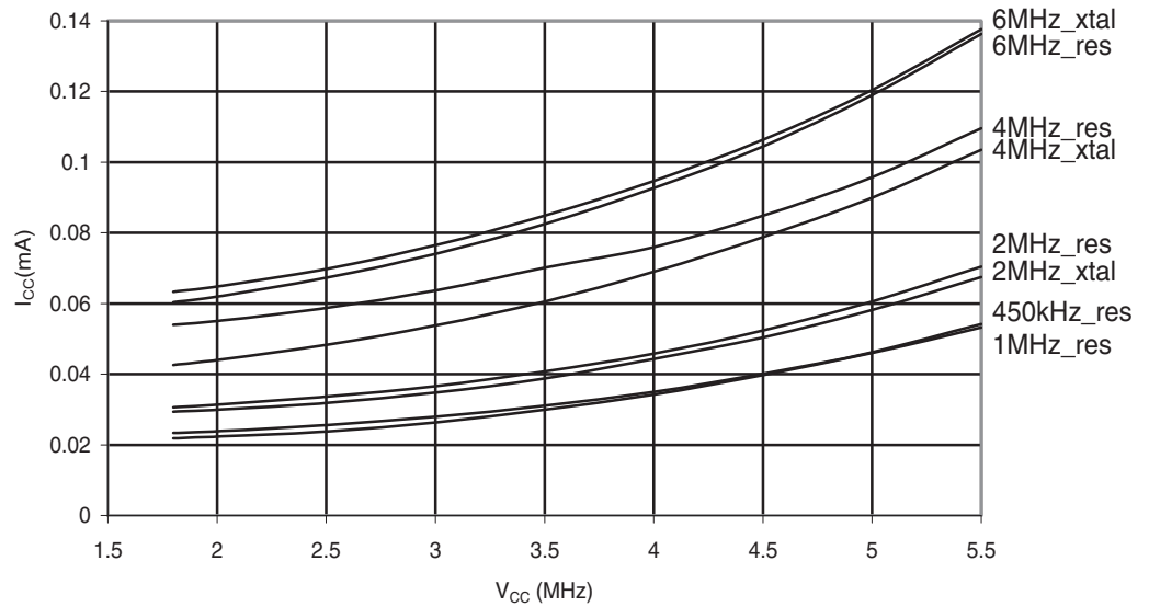
Figure 29-244. ATmega168PA: Standby Supply Current vs. V_{CC} (Watchdog Timer Disabled)
