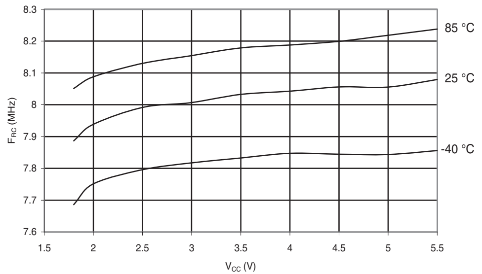
Figure 29-174. ATmega88PA: Calibrated 8 MHz RC Oscillator Frequency vs. V_{CC}
