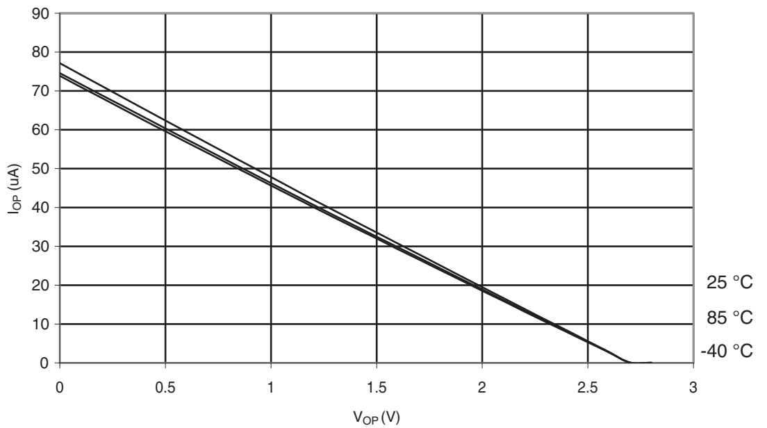
Figure 29-292. ATmega328: I/O Pin Pull-up Resistor Current vs. Input Voltage ( V_{CC} = 2.7\text{ V} )
