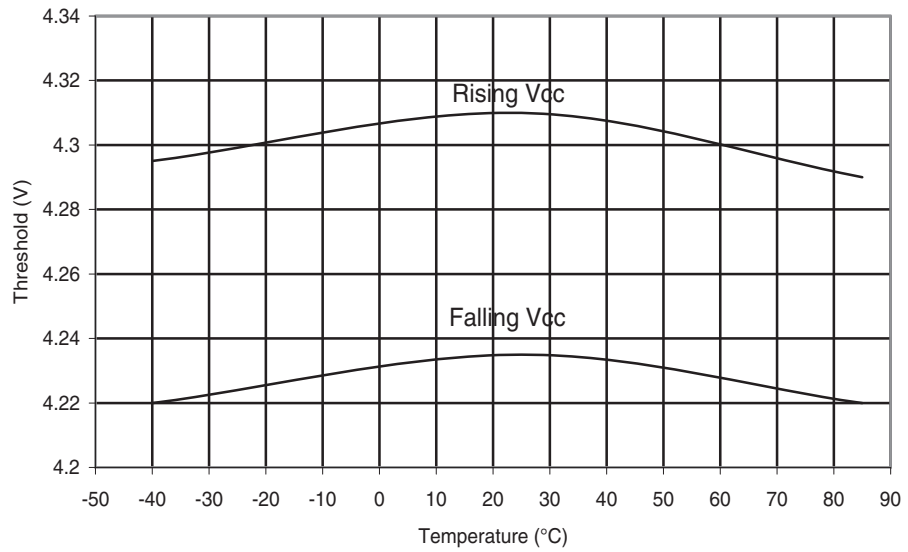
Figure 29-217. ATmega168A: BOD Thresholds vs. Temperature (BODLEVEL is 4.3 V)
