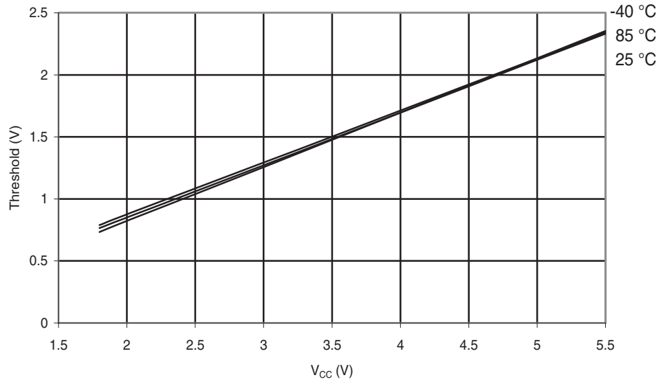
Figure 29-213. ATmega168A: Reset Input Threshold Voltage vs. V_{CC} ( V_{IL} , I/O Pin read as '0')
