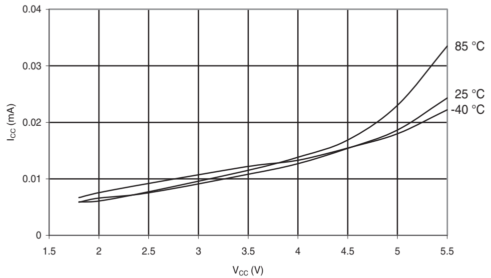
Figure 29-100. ATmega88A: Idle Supply Current vs. V_{CC} (Internal RC Oscillator, 128 kHz)
