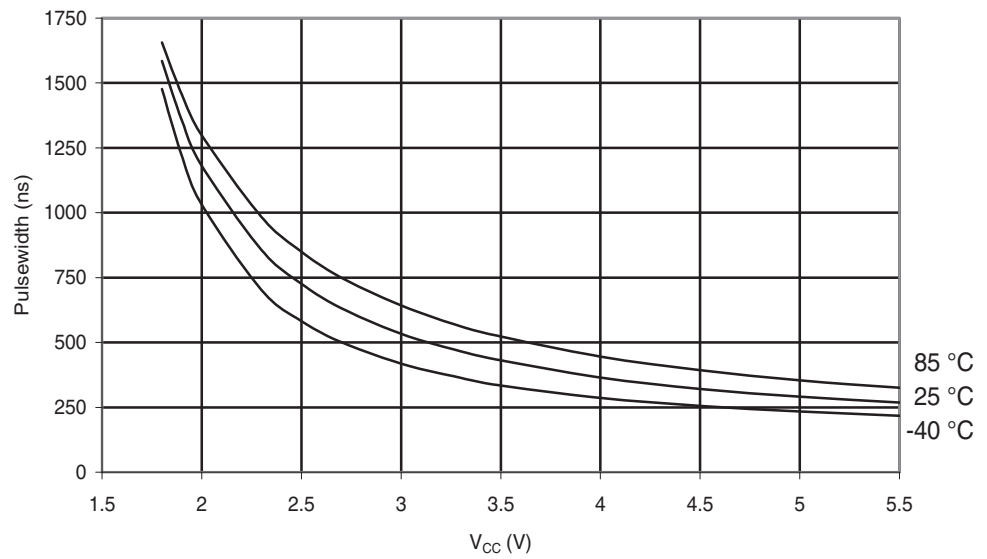
Figure 29-276. ATmega168PA: Minimum Reset Pulse width vs. V_{CC}
