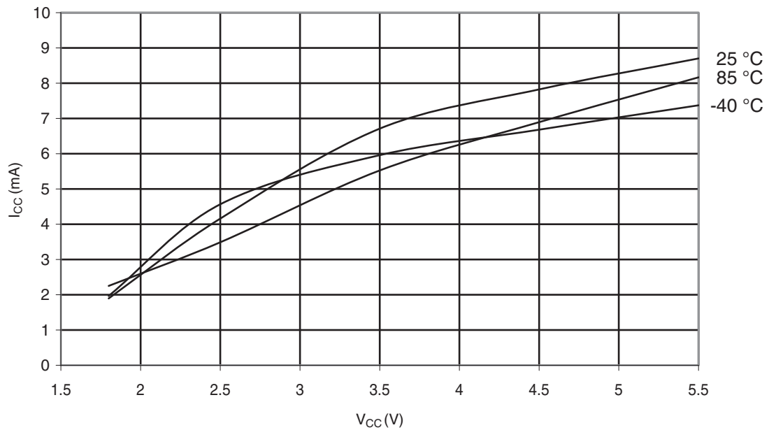
Figure 29-319. ATmega328: Programming Current vs. V_{CC}
