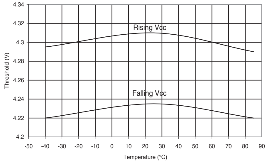
Figure 29-263. ATmega168PA: BOD Thresholds vs. Temperature (BODLEVEL is 4.3 V)
