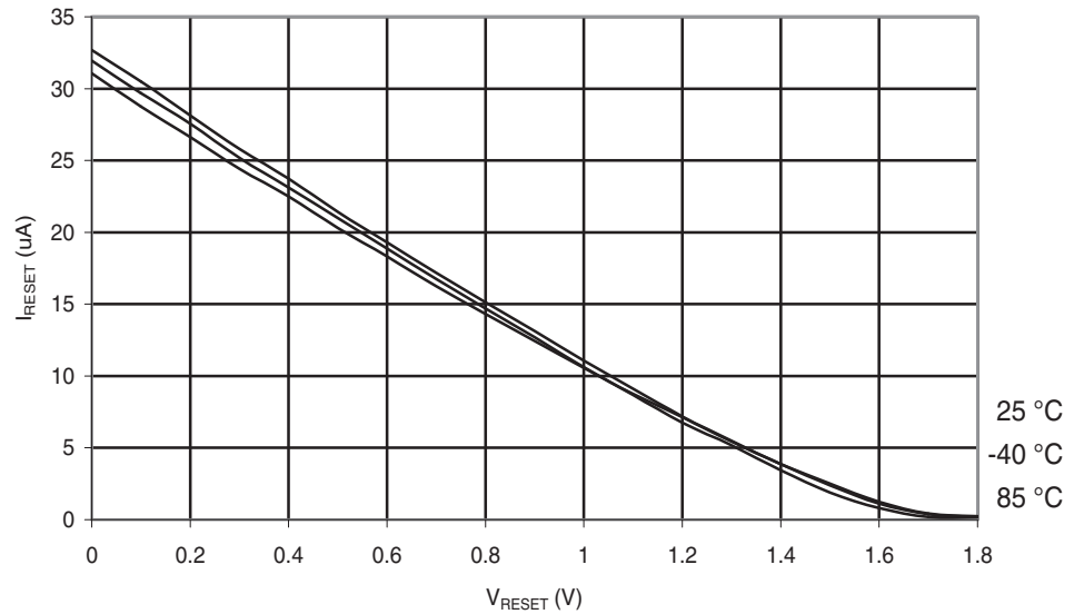
Figure 29-64. ATmega48PA: Reset Pull-up Resistor Current vs. Reset Pin Voltage ( V_{CC} = 1.8\text{ V} )
