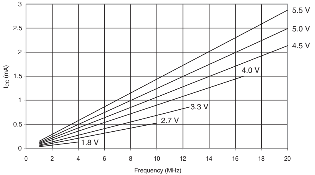
Figure 29-367. ATmega328P: Reset Supply Current vs. Frequency (1 - 20 MHz)
