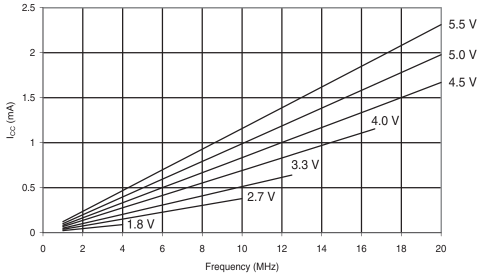
Figure 29-91. ATmega48PA: Reset Supply Current vs. Frequency (1 - 20 MHz)
