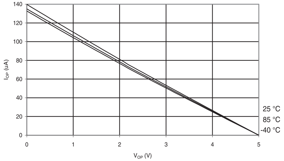
Figure 29-109. ATmega88A: I/O Pin Pull-up Resistor Current vs. Input Voltage ( V_{CC} = 5\text{ V} )
