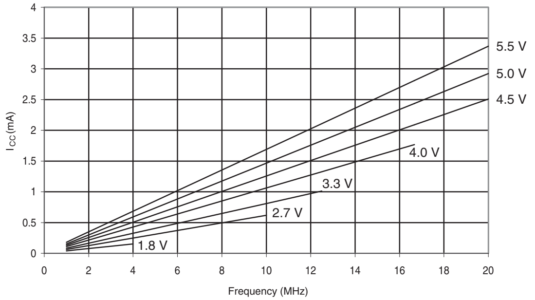
Figure 29-329. ATmega328P: Idle Supply Current vs. Frequency (1-20 MHz)
