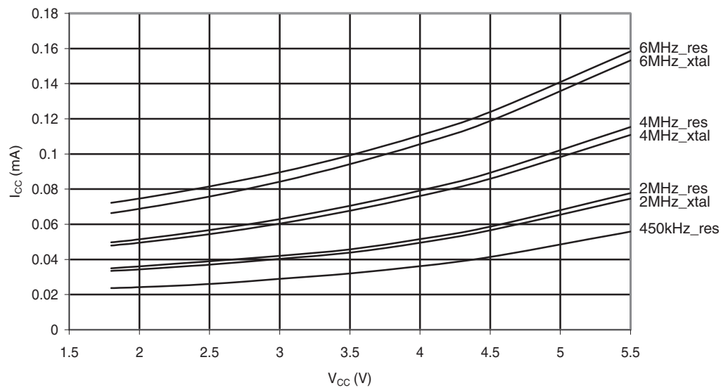
Figure 29-152. ATmega88PA: Standby Supply Current vs. V_{CC} (Watchdog Timer Disabled)
