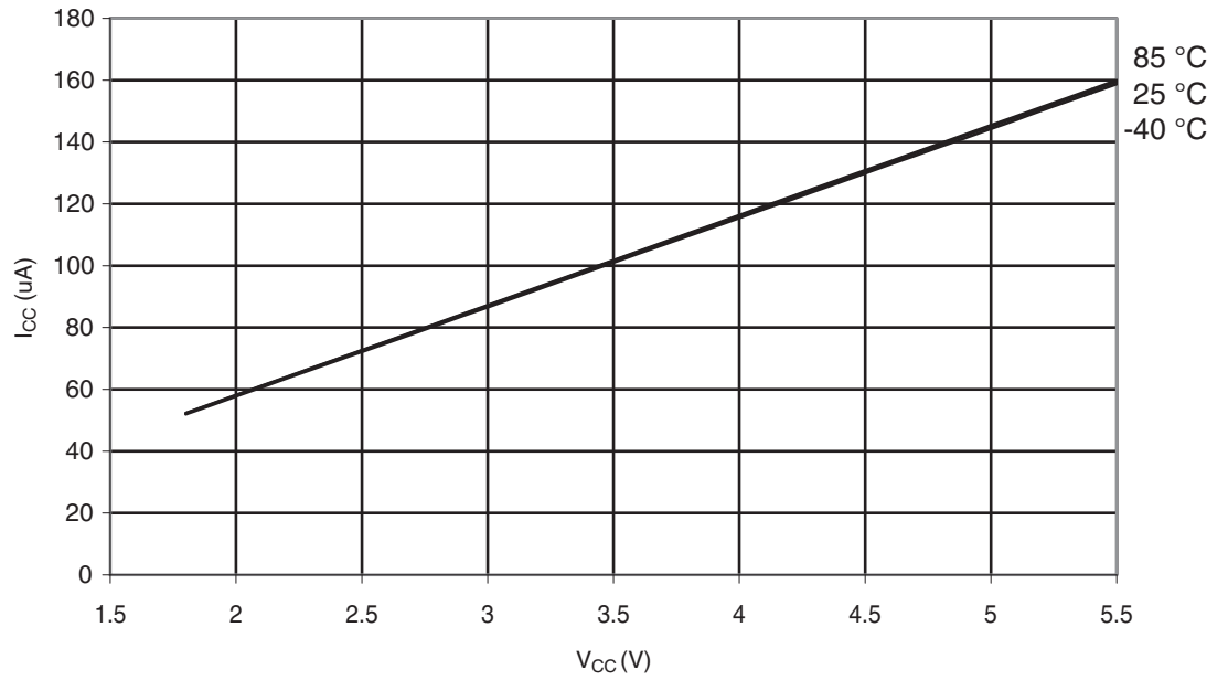
Figure 29-317. ATmega328: AREF External Reference Current vs. V_{CC}
