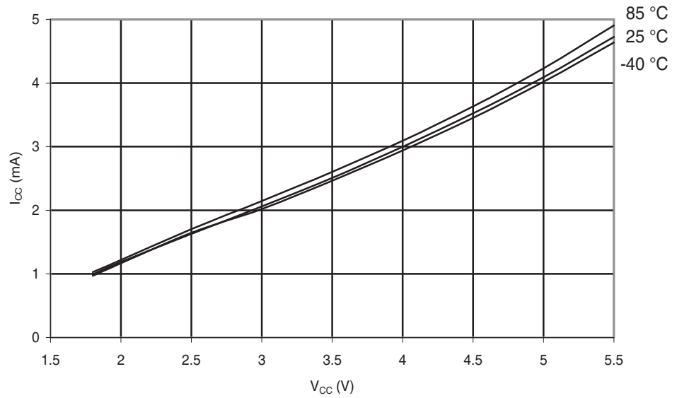
Figure 29-143. ATmega88PA: Active Supply Current vs. V_{CC} (Internal RC Oscillator, 8 MHz)
