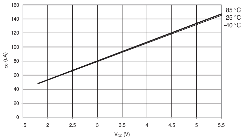
Figure 29-87. ATmega48PA: AREF External Reference Current vs. V_{CC}
