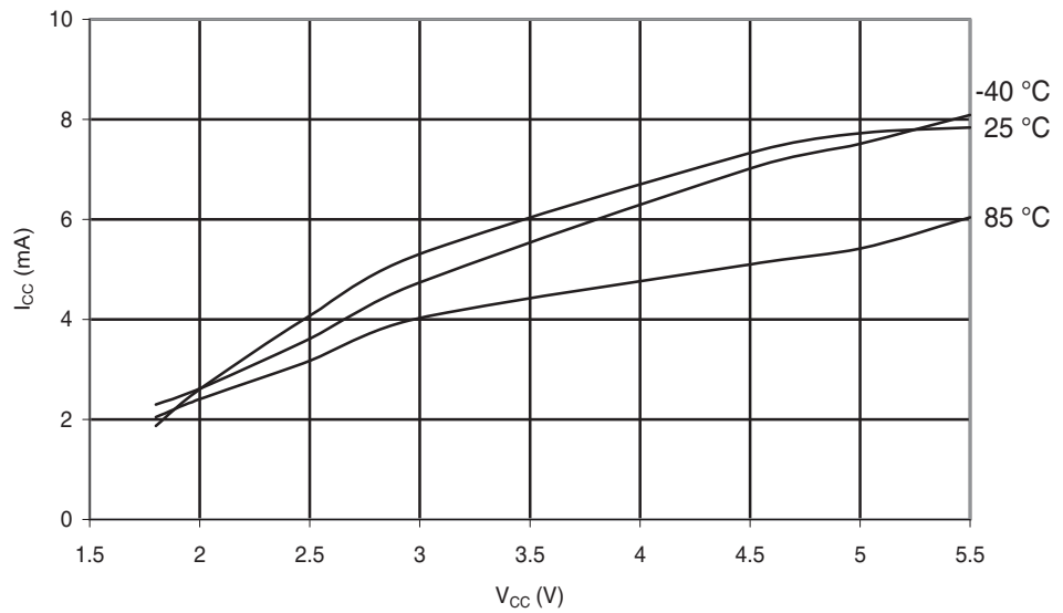
Figure 29-273. ATmega168PA: Programming Current vs. V_{CC}
