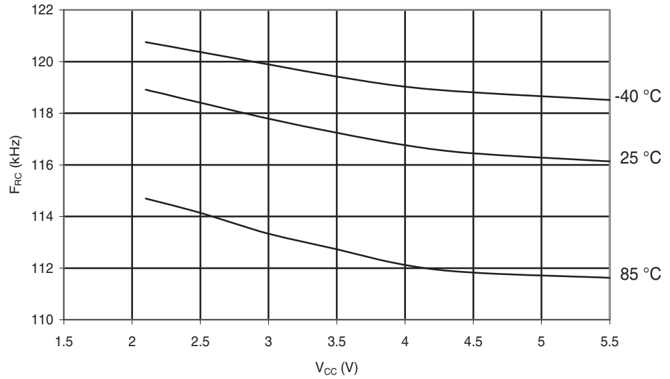
Figure 29-219. ATmega168A: Watchdog Oscillator Frequency vs. V_{CC}
