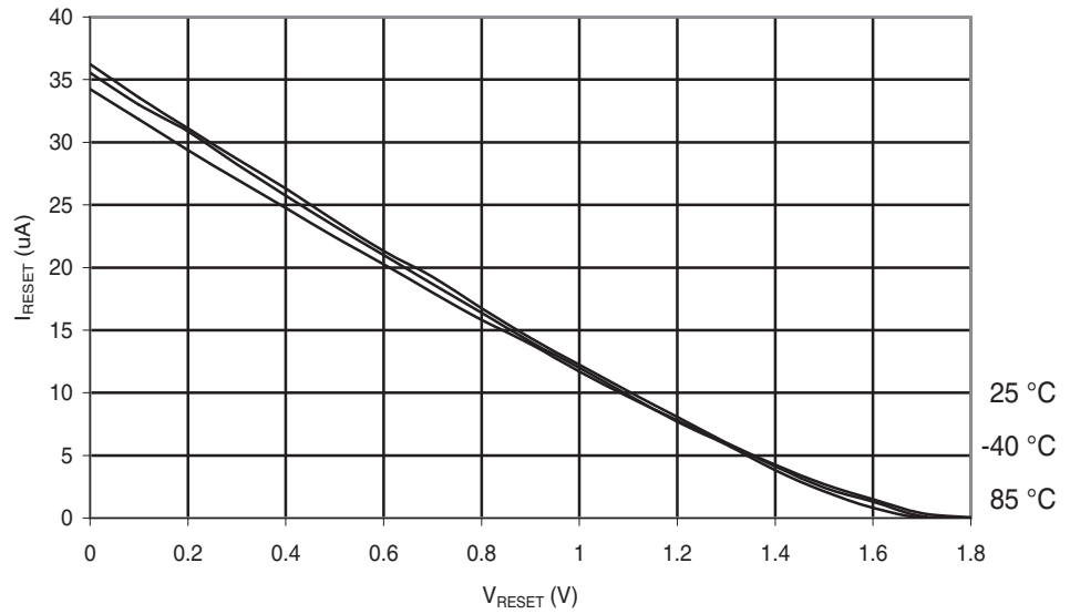
Figure 29-110. ATmega88A: Reset Pull-up Resistor Current vs. Reset Pin Voltage ( V_{CC} = 1.8\text{ V} )
