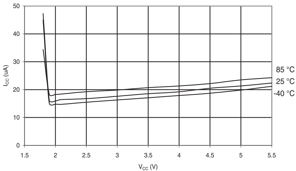
Figure 29-134. ATmega88A: Brownout Detector Current vs. V_{CC}
