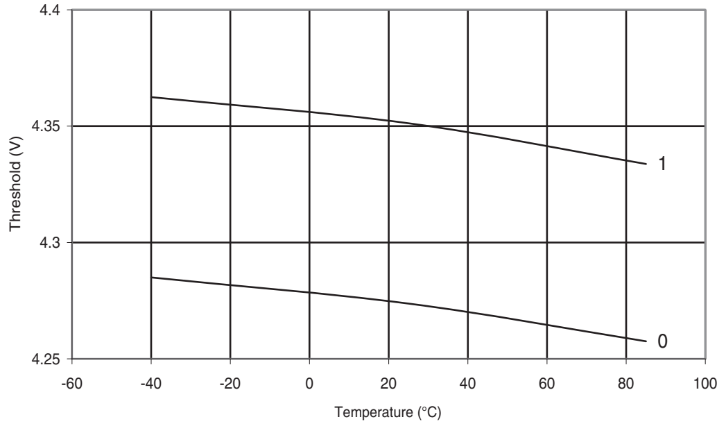
Figure 29-355. ATmega328P: BOD Thresholds vs. Temperature (BODLEVEL is 4.3 V)
