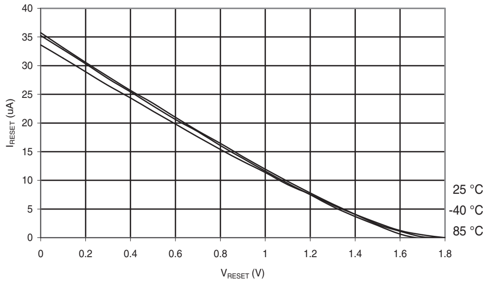
Figure 29-248. ATmega168PA: Reset Pull-up Resistor Current vs. Reset Pin Voltage ( V_{CC} = 1.8\text{ V} )
