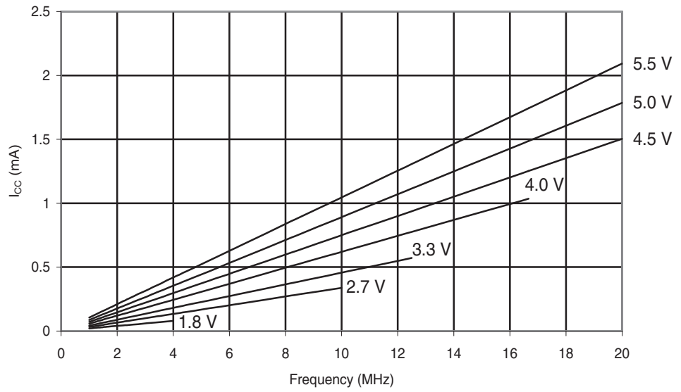
Figure 29-229. ATmega168A: Reset Supply Current vs. Frequency (1 - 20 MHz)
