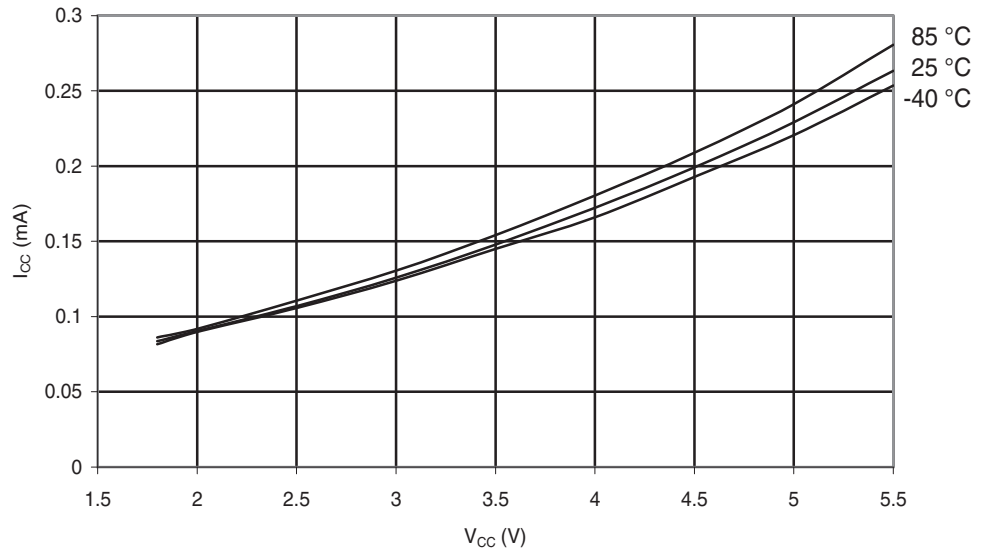
Figure 29-193. ATmega168A: Idle Supply Current vs. V_{CC} (Internal RC Oscillator, 1 MHz)
