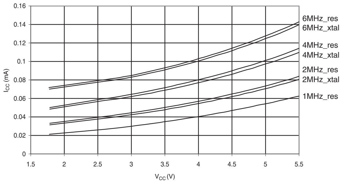
Figure 29-336. ATmega328P: Standby Supply Current vs. V_{CC} (Watchdog Timer Disabled)
