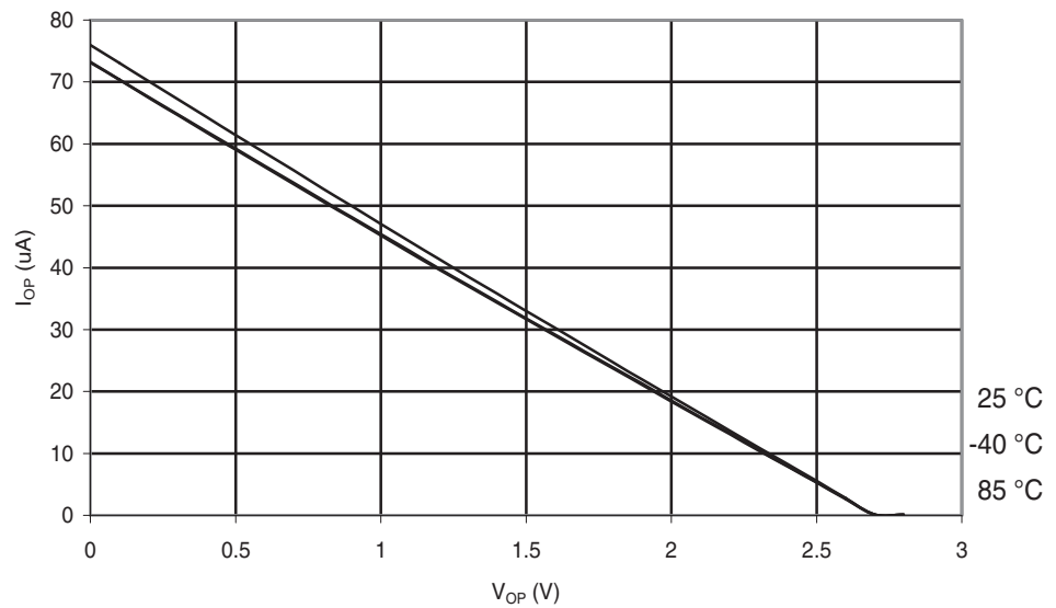
Figure 29-200. ATmega168A: I/O Pin Pull-up Resistor Current vs. Input Voltage ( V_{CC} = 2.7\text{ V} )
