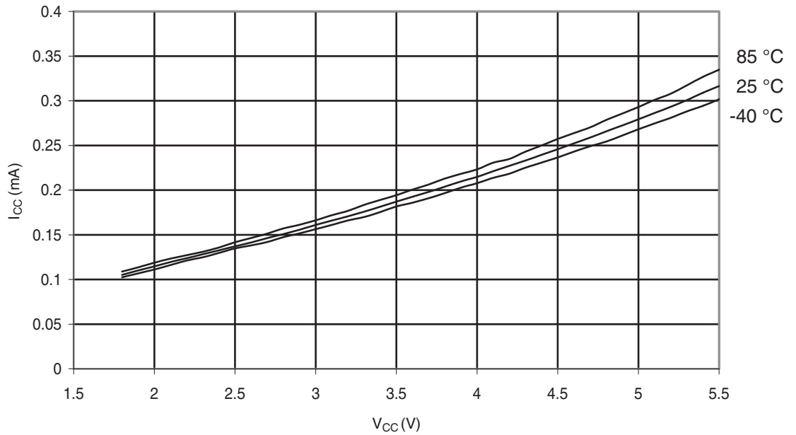
Figure 29-285. ATmega328: Idle Supply Current vs. V_{CC} (Internal RC Oscillator, 1 MHz)
