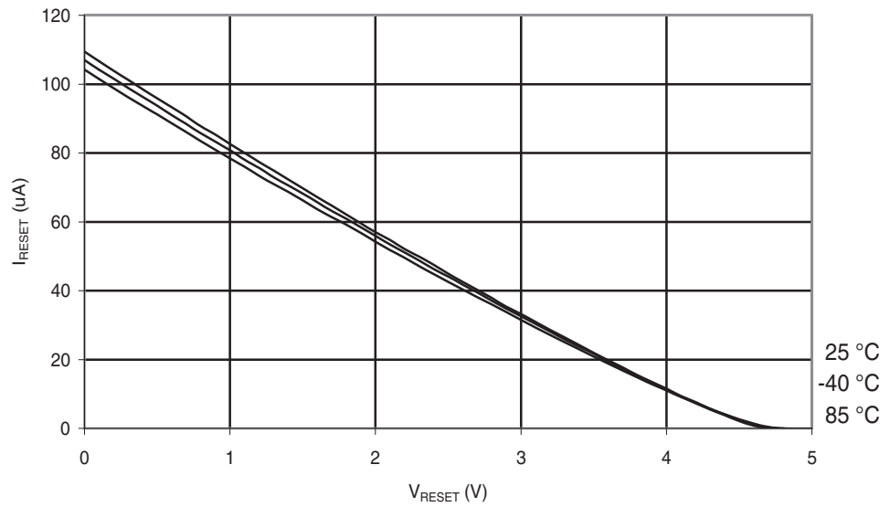
Figure 29-250. ATmega168PA: Reset Pull-up Resistor Current vs. Reset Pin Voltage ( V_{CC} = 5\text{V} )
