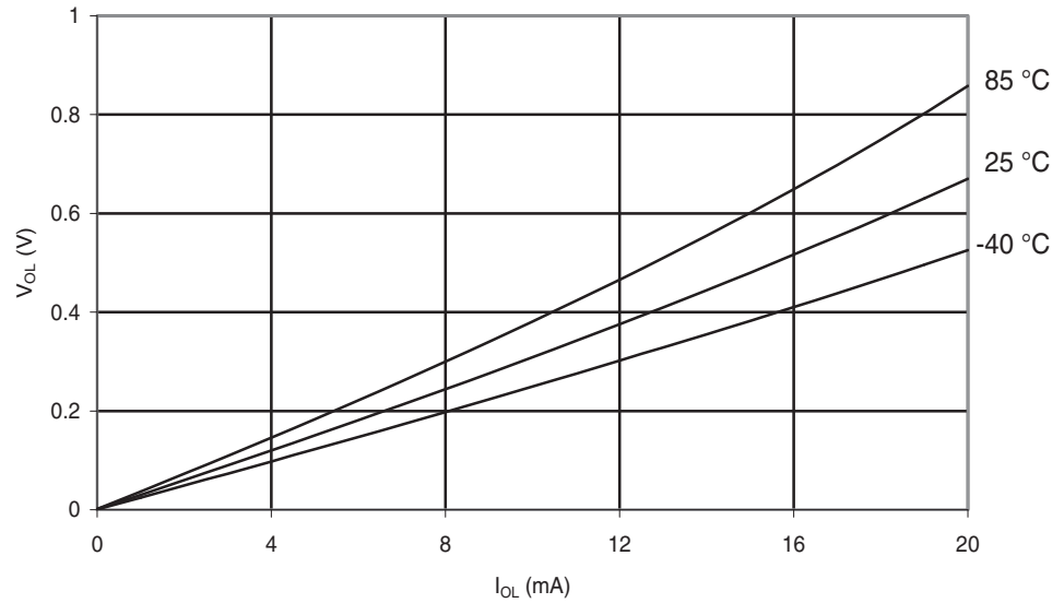
Figure 29-159. ATmega88PA: I/O Pin Output Voltage vs. Sink Current ( V_{CC} = 3\text{ V} )
