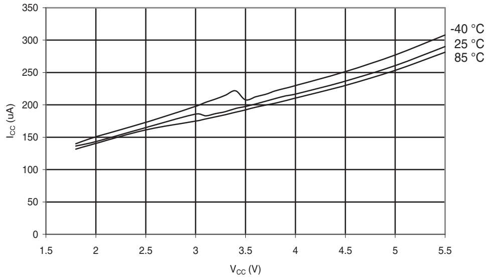
Figure 29-39. ATmega48A: ADC Current vs. V_{CC} (AREF = AV_{CC} )
