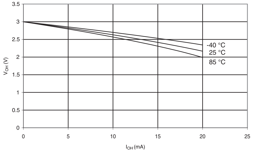
Figure 29-345. ATmega328P: I/O Pin Output Voltage vs. Source Current ( V_{CC} = 3\text{ V} )
