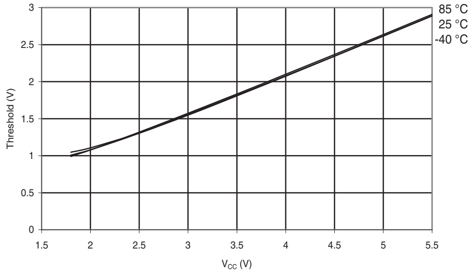
Figure 29-255. ATmega168PA: I/O Pin Input Threshold Voltage vs. V_{CC} ( V_{IH} , I/O Pin read as '1')
