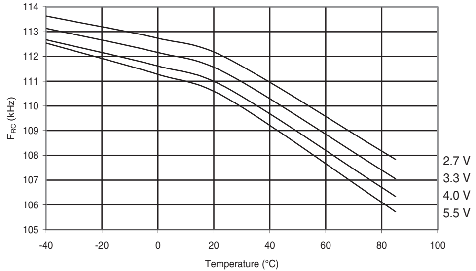
Figure 29-172. ATmega88PA: Watchdog Oscillator Frequency vs. Temperature
