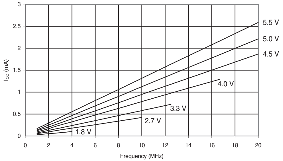
Figure 29-53. ATmega48PA: Idle Supply Current vs. Frequency (1-20 MHz)
