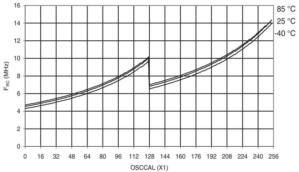
Figure 29-268. ATmega168PA: Calibrated 8 MHz RC Oscillator Frequency vs. OSCCAL Value
