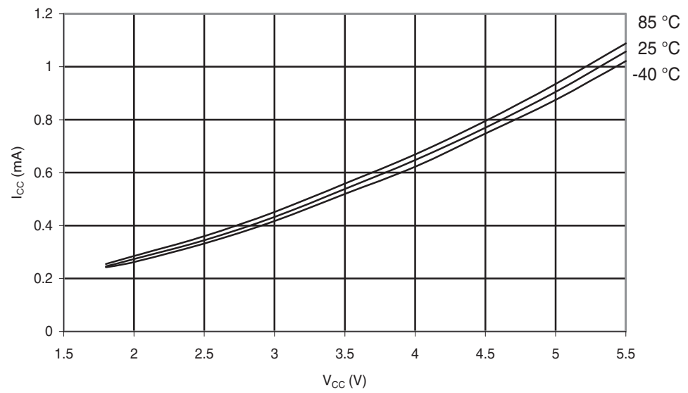
Figure 29-188. ATmega168A: Active Supply Current vs. V_{CC} (Internal RC Oscillator, 1 MHz)
