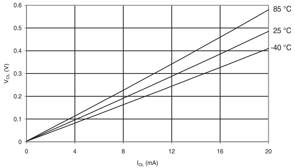
Figure 29-68. ATmega48PA: I/O Pin Output Voltage vs. Sink Current ( V_{CC} = 5\text{ V} )
