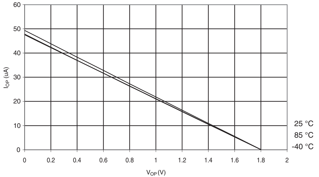
Figure 29-291. ATmega328: I/O Pin Pull-up Resistor Current vs. Input Voltage ( V_{CC} = 1.8\text{ V} )
