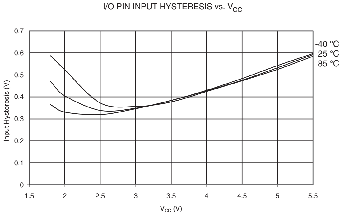
Figure 29-303. ATmega328: I/O Pin Input Hysteresis vs. V_{CC}
