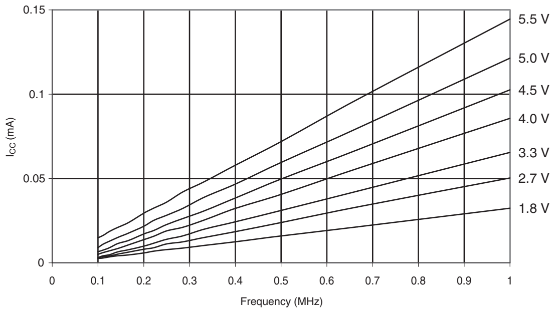
Figure 29-366. ATmega328P: Reset Supply Current vs. Low Frequency (0.1 - 1.0 MHz)
