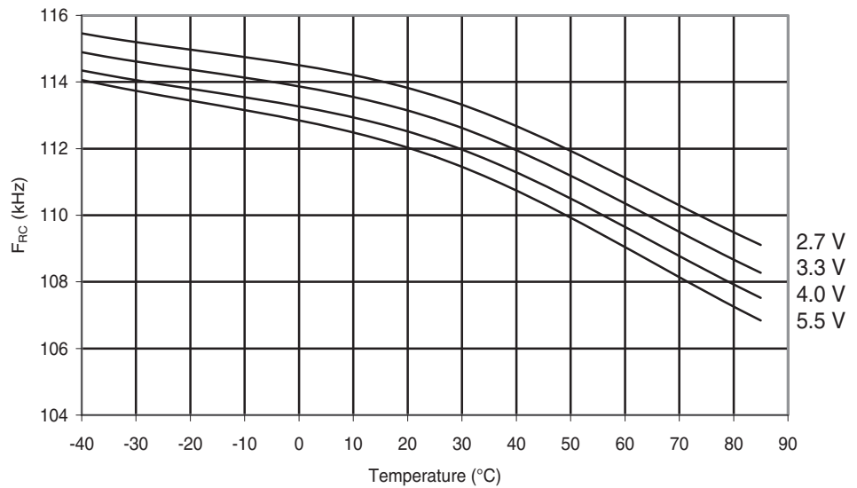
Figure 29-34. ATmega48A: Watchdog Oscillator Frequency vs. Temperature
