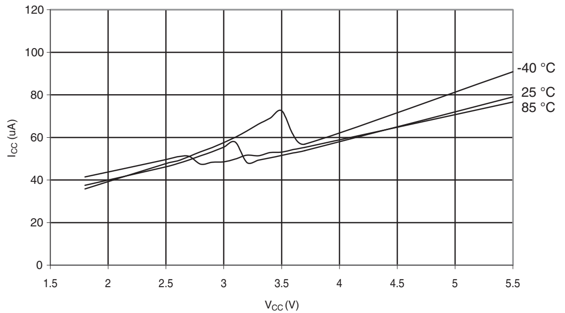
Figure 29-362. ATmega328P: Analog Comparator Current vs. V_{CC}
