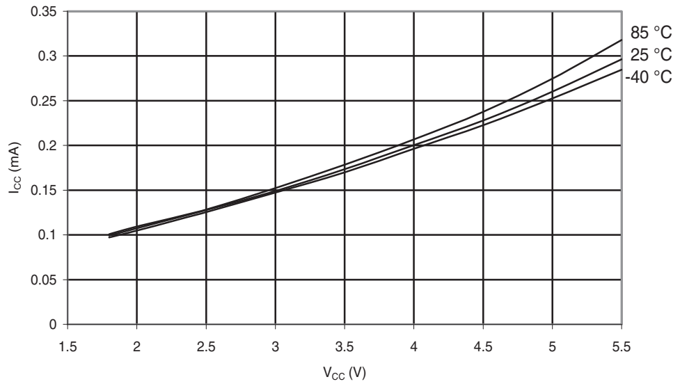
Figure 29-147. ATmega88PA: Idle Supply Current vs. V_{CC} (Internal RC Oscillator, 1 MHz)
