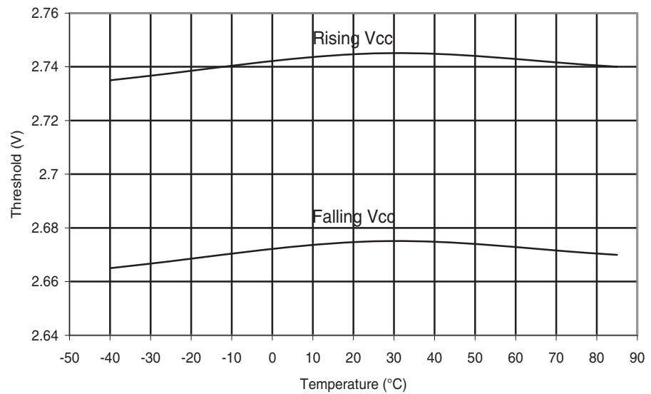
Figure 29-170. ATmega88PA: BOD Thresholds vs. Temperature (BODLEVEL is 2.7 V)
