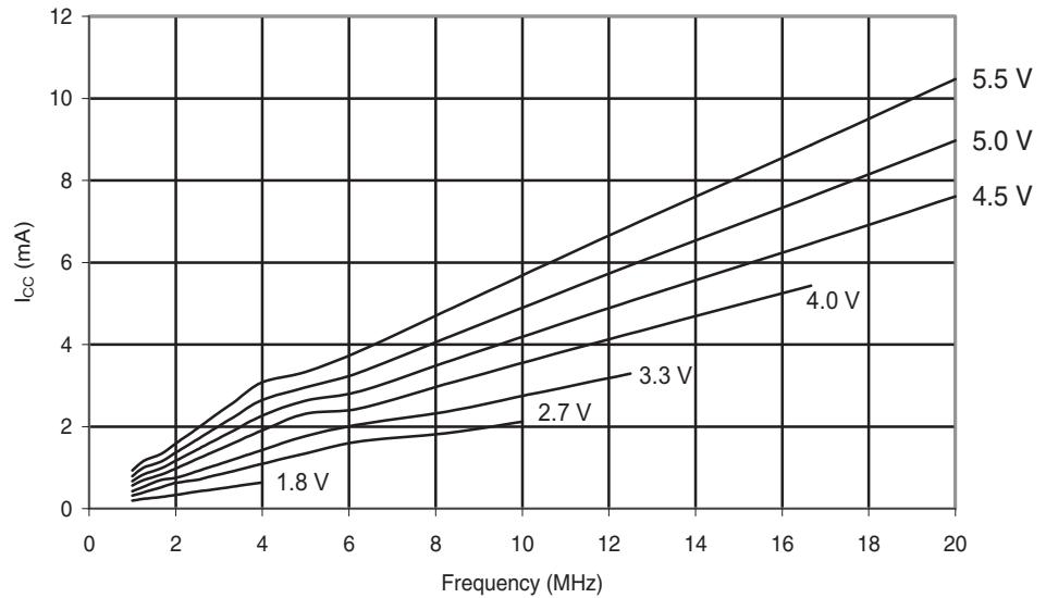
Figure 29-140. ATmega88PA: Active Supply Current vs. Frequency (1 - 20 MHz)
