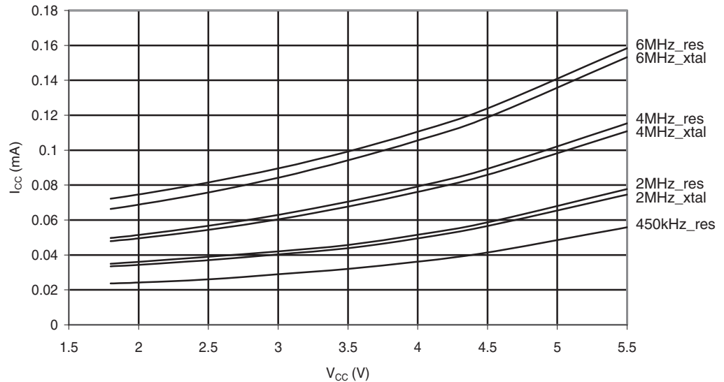
Figure 29-106. ATmega88A: Standby Supply Current vs. V_{CC} (Watchdog Timer Disabled)
