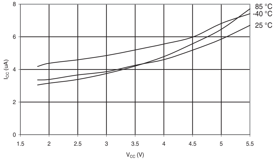
Figure 29-104. ATmega88A: Power-Down Supply Current vs. V_{CC} (Watchdog Timer Enabled)
