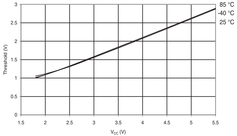
Figure 29-163. ATmega88PA: I/O Pin Input Threshold Voltage vs. V_{CC} ( V_{IH} , I/O Pin read as '1')
