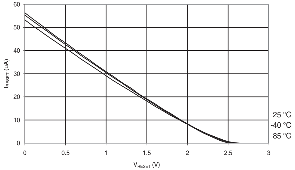
Figure 29-249. ATmega168PA: Reset Pull-up Resistor Current vs. Reset Pin Voltage ( V_{CC} = 2.7\text{ V} )
