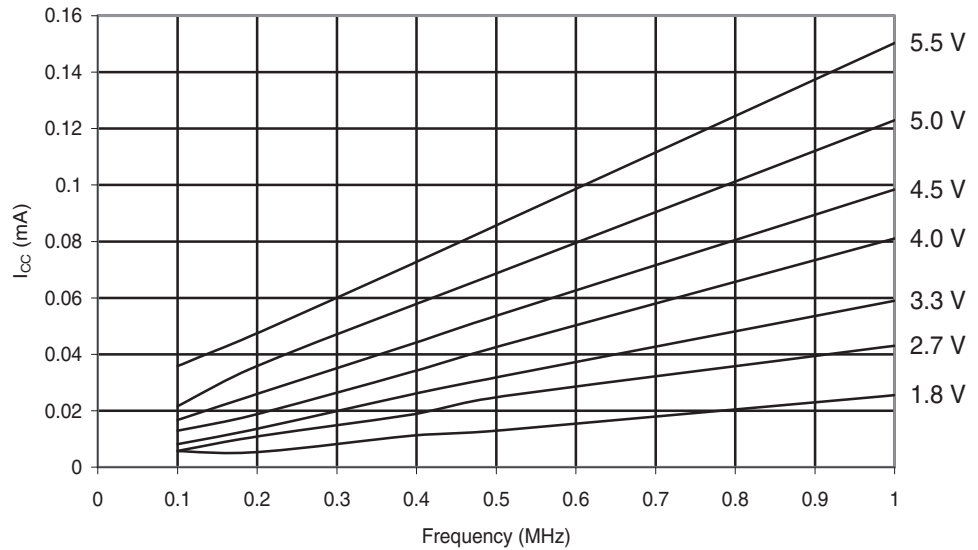
Figure 29-52. ATmega48PA: Idle Supply Current vs. Low Frequency (0.1-1.0 MHz)
