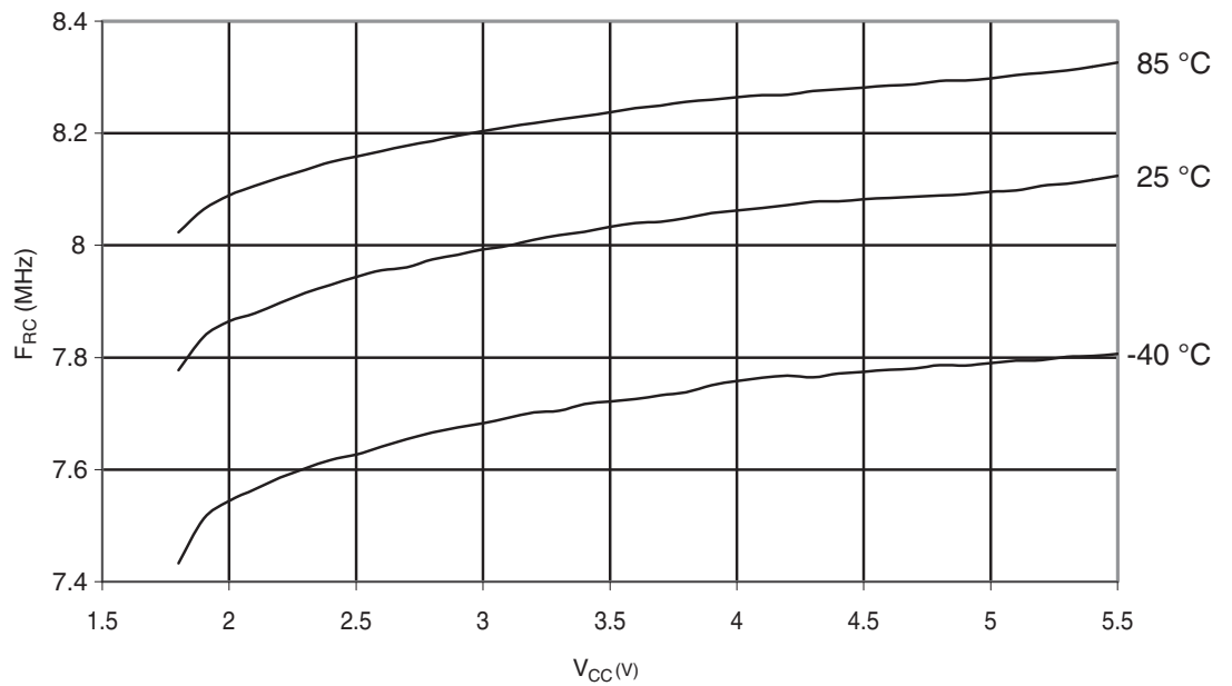
Figure 29-358. ATmega328P: Calibrated 8 MHz RC Oscillator Frequency vs. V_{CC}
