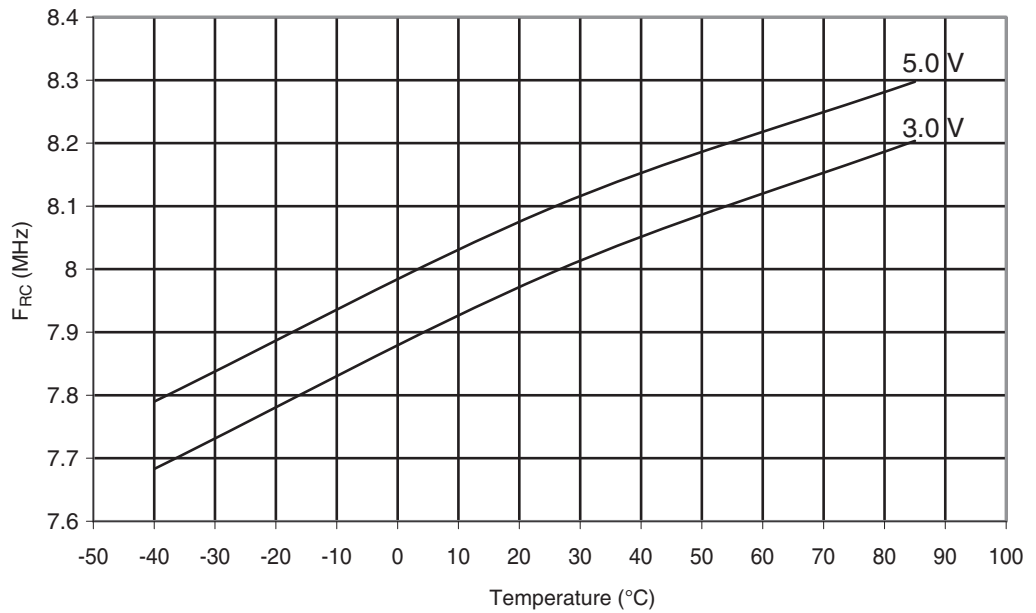
Figure 29-313. ATmega328: Calibrated 8 MHz RC Oscillator Frequency vs. Temperature
