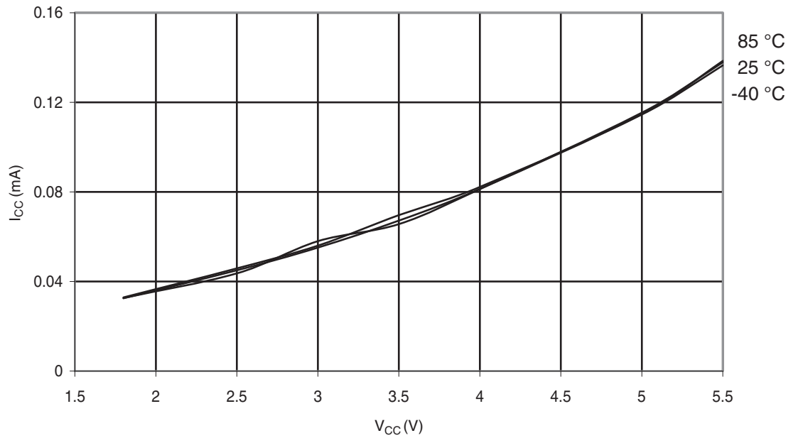
Figure 29-325. ATmega328P: Active Supply Current vs. V_{CC} (Internal RC Oscillator, 128 kHz)
