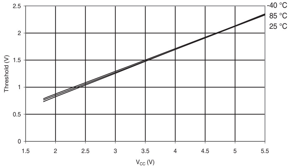
Figure 29-259. ATmega168PA: Reset Input Threshold Voltage vs. V_{CC} ( V_{IL} , I/O Pin read as '0')
