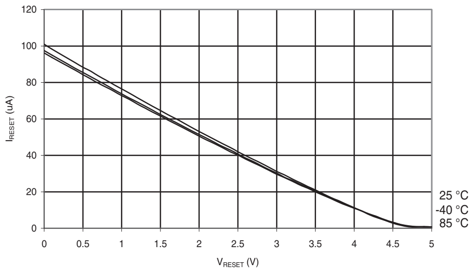
Figure 29-66. ATmega48PA: Reset Pull-up Resistor Current vs. Reset Pin Voltage ( V_{CC} = 5\text{ V} )
