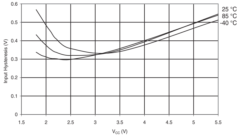
Figure 29-73. ATmega48PA: I/O Pin Input Hysteresis vs. V_{CC}
