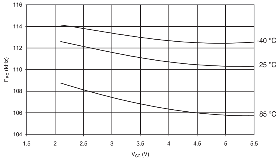
Figure 29-127. ATmega88A: Watchdog Oscillator Frequency vs. V_{CC}
