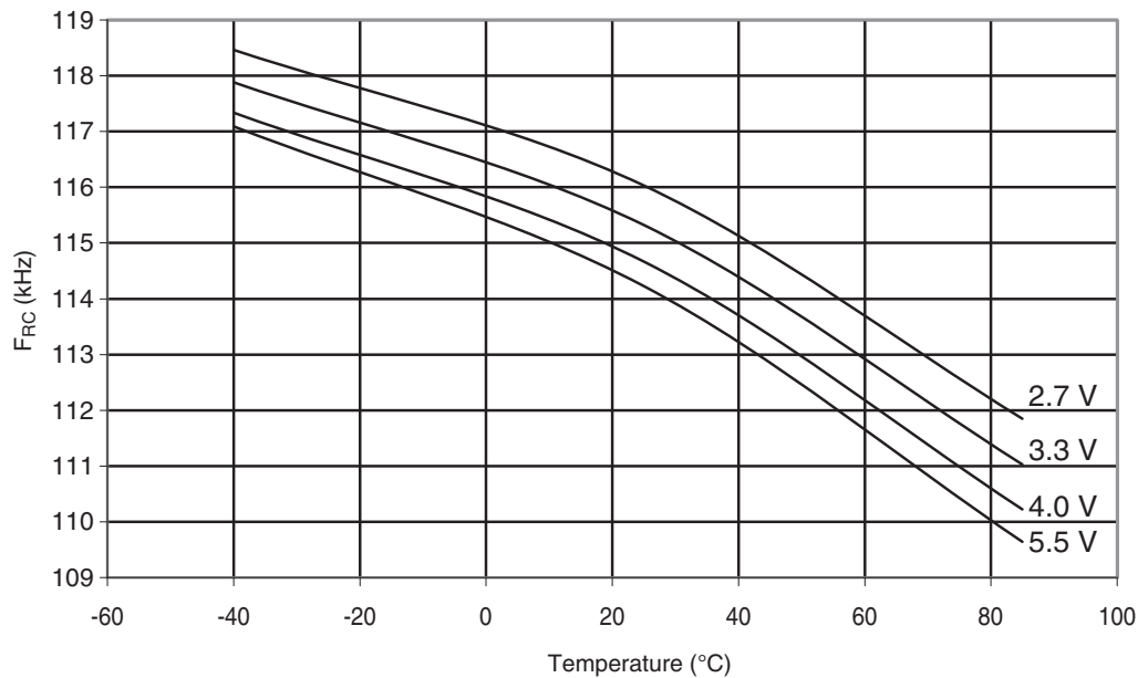
Figure 29-310. ATmega328: Watchdog Oscillator Frequency vs. Temperature
