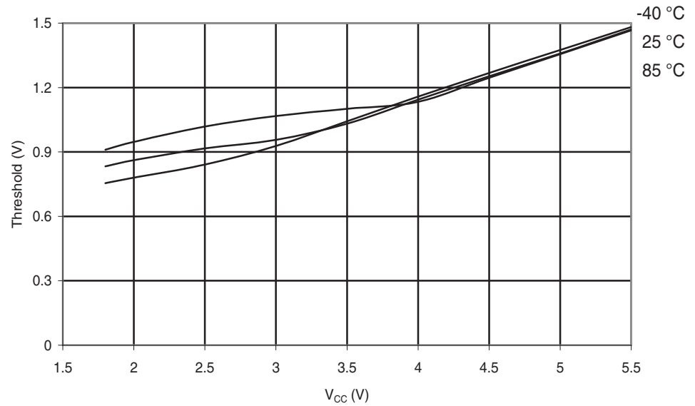
Figure 29-166. ATmega88PA: Reset Input Threshold Voltage vs. V_{CC} ( V_{IH} , I/O Pin read as '1')
