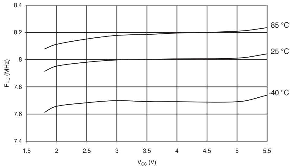
Figure 29-220. ATmega168A: Calibrated 8 MHz RC Oscillator Frequency vs. V_{CC}
