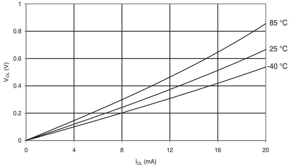
Figure 29-251. ATmega168PA: I/O Pin Output Voltage vs. Sink Current ( V_{CC} = 3\text{ V} )
