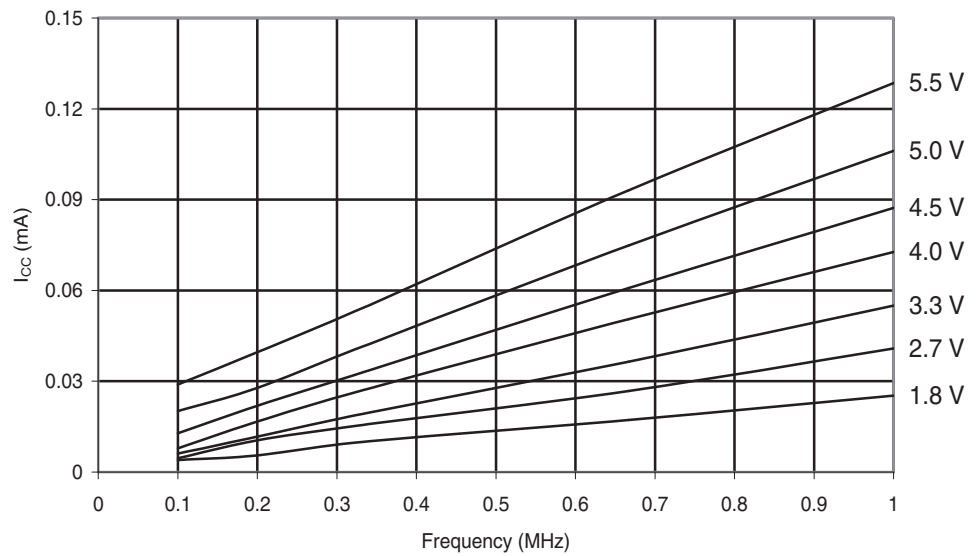
Figure 29-144. ATmega88PA: Idle Supply Current vs. Low Frequency (0.1-1.0 MHz)
