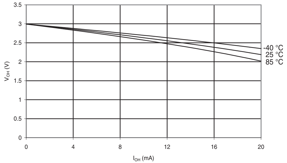
Figure 29-253. ATmega168PA: I/O Pin Output Voltage vs. Source Current ( V_{CC} = 3\text{ V} )
