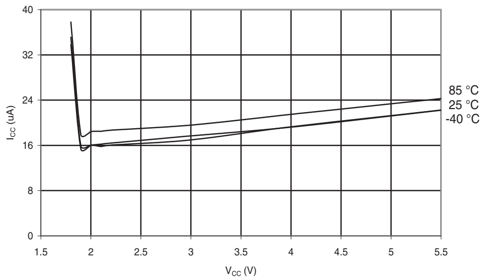
Figure 29-42. ATmega48A Brownout Detector Current vs. V_{CC}
