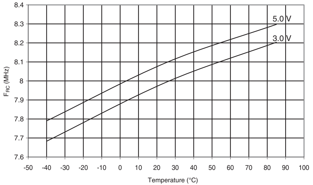
Figure 29-359. ATmega328P: Calibrated 8 MHz RC Oscillator Frequency vs. Temperature
