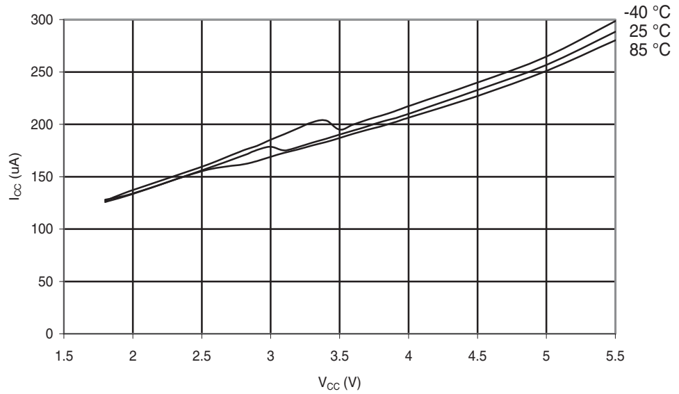
Figure 29-177. ATmega88PA: ADC Current vs. V_{CC} (AREF = AV_{CC} )
