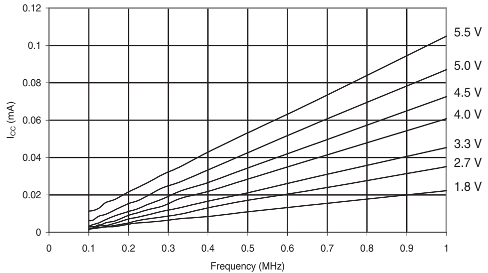
Figure 29-136. ATmega88A: Reset Supply Current vs. Low Frequency (0.1 - 1.0 MHz)
