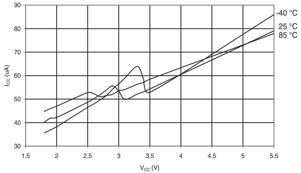
Figure 29-224. ATmega168A: Analog Comparator Current vs. V_{CC}
