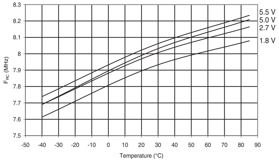
Figure 29-267. ATmega168PA: Calibrated 8 MHz RC Oscillator Frequency vs. Temperature
