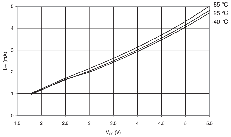
Figure 29-235. ATmega168PA: Active Supply Current vs. V_{CC} (Internal RC Oscillator, 8 MHz)
