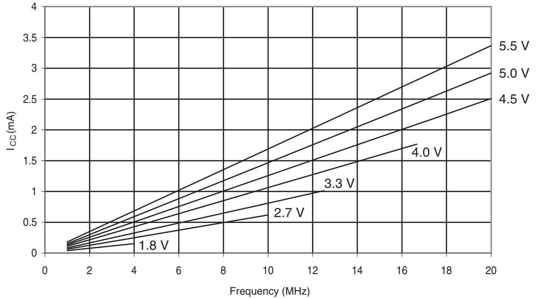
Figure 29-283. ATmega328: Idle Supply Current vs. Frequency (1-20 MHz)
