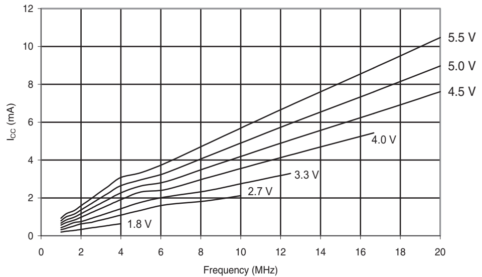
Figure 29-94. ATmega88A: Active Supply Current vs. Frequency (1 - 20 MHz)
