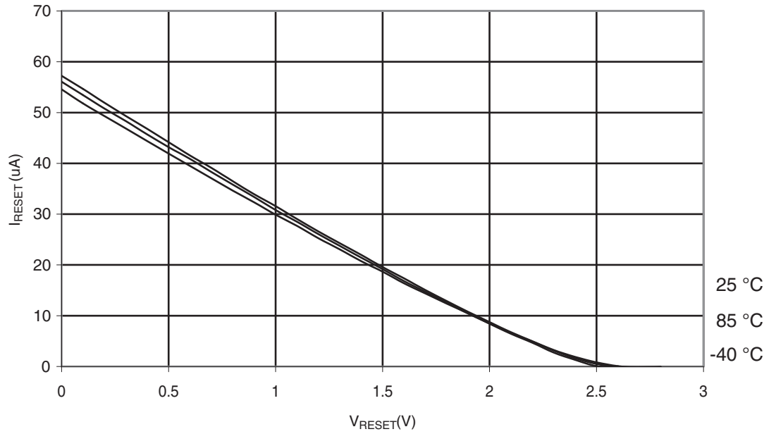
Figure 29-341. ATmega328P: Reset Pull-up Resistor Current vs. Reset Pin Voltage ( V_{CC} = 2.7\text{ V} )
