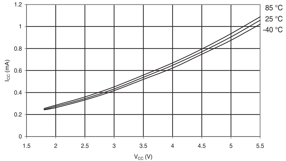
Figure 29-234. ATmega168PA: Active Supply Current vs. V_{CC} (Internal RC Oscillator, 1 MHz)
