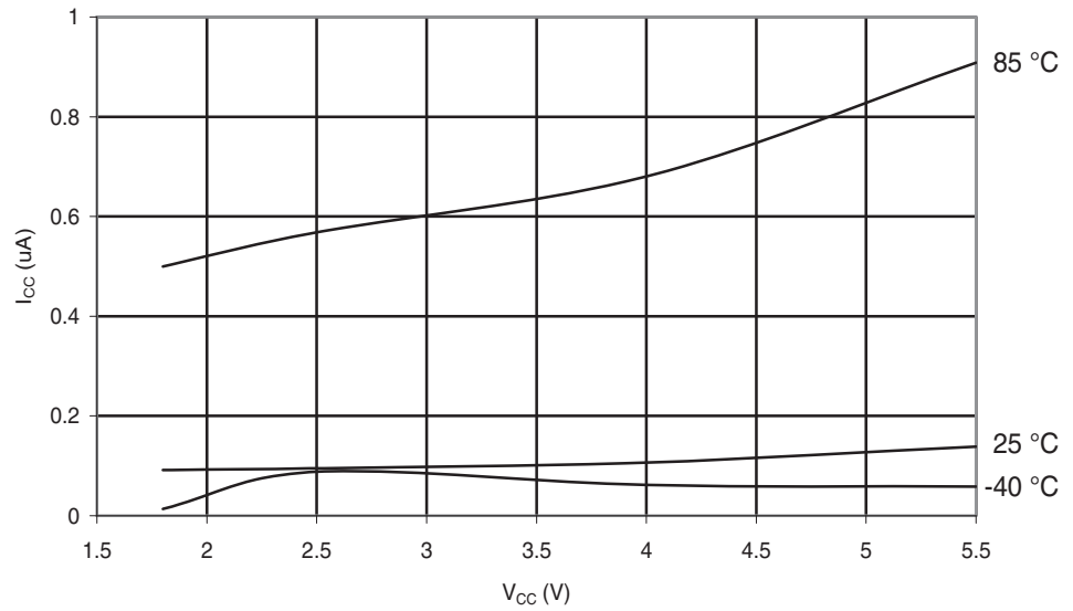
Figure 29-241. ATmega168PA: Power-Down Supply Current vs. V_{CC} (Watchdog Timer Disabled)
