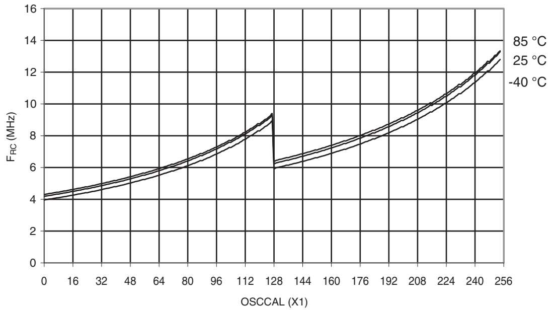
Figure 29-314. ATmega328: Calibrated 8 MHz RC Oscillator Frequency vs. OSCCAL Value
