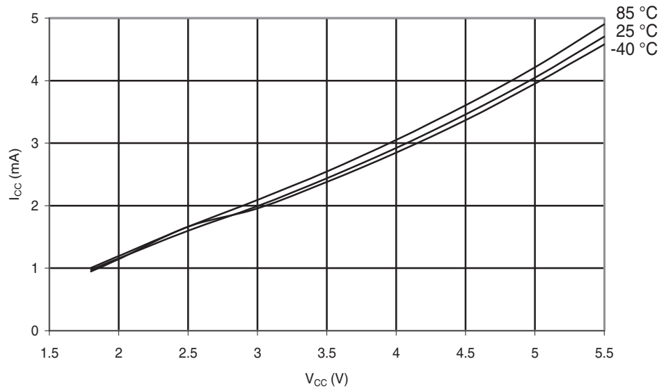
Figure 29-51. ATmega48PA: Active Supply Current vs. V_{CC} (Internal RC Oscillator, 8 MHz)
