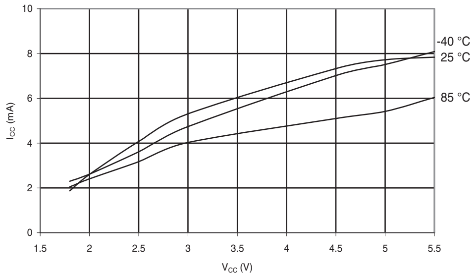
Figure 29-227. ATmega168A: Programming Current vs. V_{CC}
