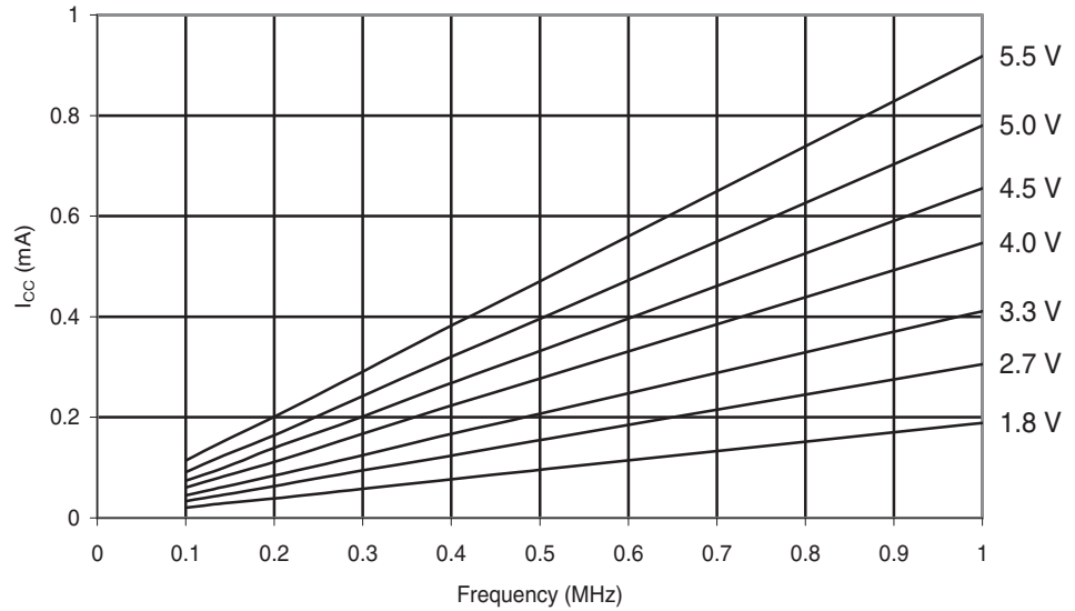
Figure 29-47. ATmega48PA: Active Supply Current vs. Low Frequency (0.1-1.0 MHz)
