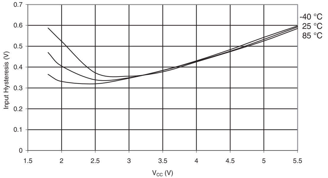
Figure 29-349. ATmega328P: I/O Pin Input Hysteresis vs. V_{CC}
