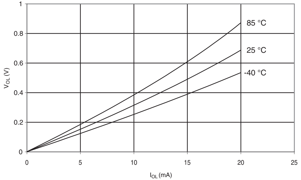
Figure 29-297. ATmega328: I/O Pin Output Voltage vs. Sink Current ( V_{CC} = 3\text{ V} )
