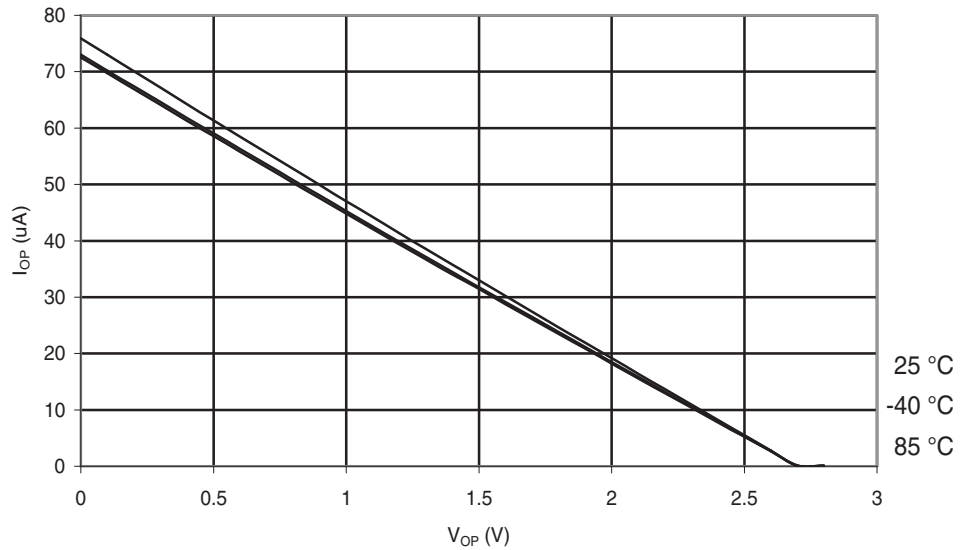
Figure 29-154. ATmega88PA: I/O Pin Pull-up Resistor Current vs. Input Voltage ( V_{CC} = 2.7\text{ V} )
