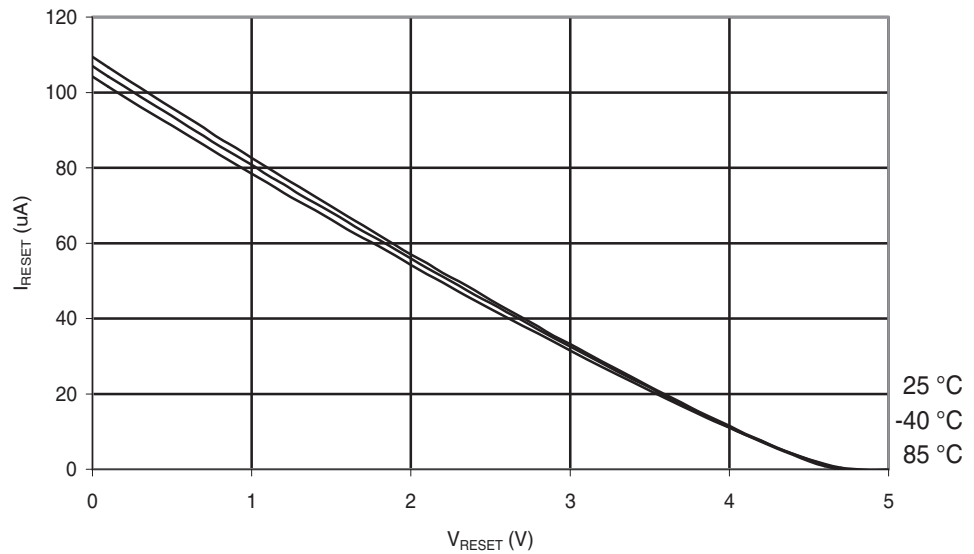
Figure 29-204. ATmega168A: Reset Pull-up Resistor Current vs. Reset Pin Voltage ( V_{CC} = 5\text{ V} )
