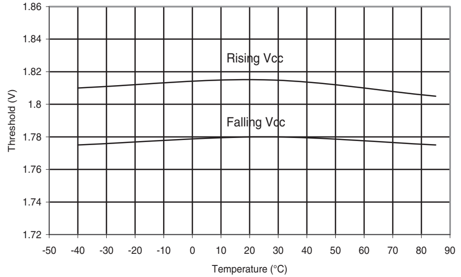
Figure 29-261. ATmega168PA: BOD Thresholds vs. Temperature (BODLEVEL is 1.8 V)
