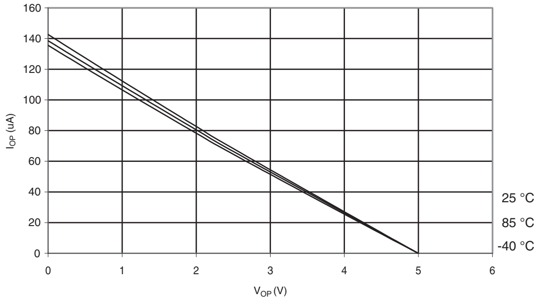
Figure 29-293. ATmega328: I/O Pin Pull-up Resistor Current vs. Input Voltage ( V_{CC} = 5\text{ V} )
