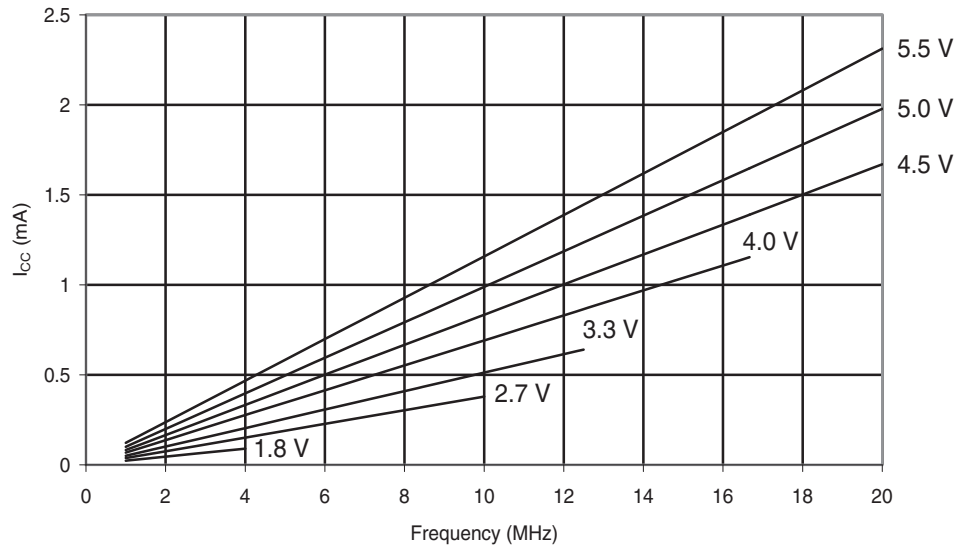
Figure 29-45. ATmega48A: Reset Supply Current vs. Frequency (1 - 20 MHz)
