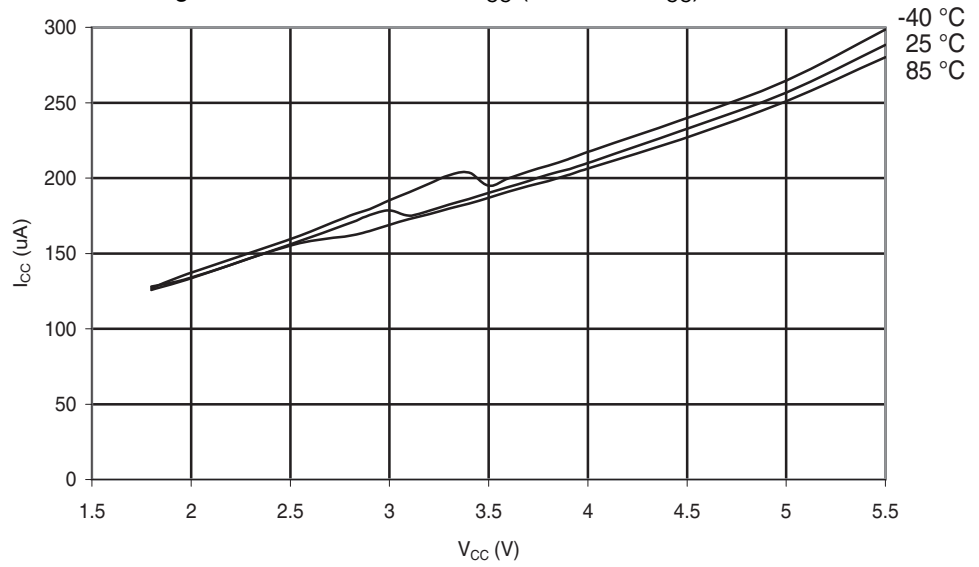
Figure 29-131. ATmega88A: ADC Current vs. V_{CC} (AREF = AV_{CC} )
