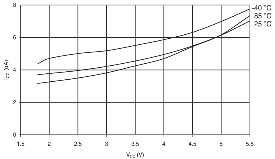
Figure 29-242. ATmega168PA: Power-Down Supply Current vs. V_{CC} (Watchdog Timer Enabled)
