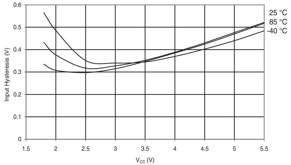
Figure 29-119. ATmega88A: I/O Pin Input Hysteresis vs. V_{CC}
