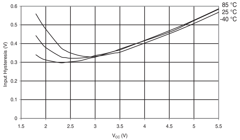
Figure 29-257. ATmega168PA: I/O Pin Input Hysteresis vs. V_{CC}
