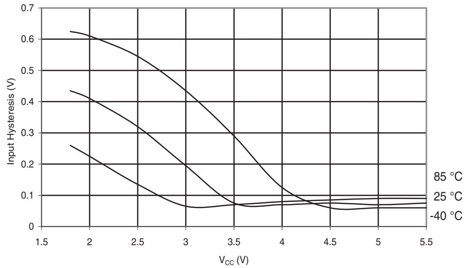
Figure 29-214. ATmega168A: Reset Pin Input Hysteresis vs. V_{CC} RESET PIN INPUT HYSTERESIS vs. V_{CC}
