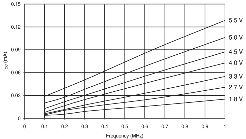
Figure 29-98. ATmega88A: Idle Supply Current vs. Low Frequency (0.1-1.0 MHz)
