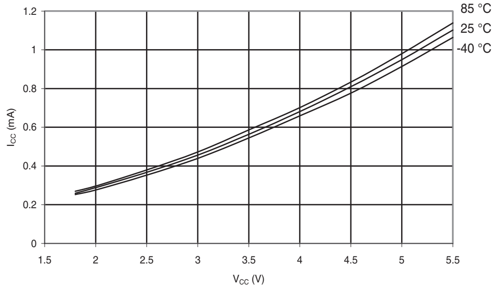
Figure 29-142. ATmega88PA: Active Supply Current vs. V_{CC} (Internal RC Oscillator, 1 MHz)
