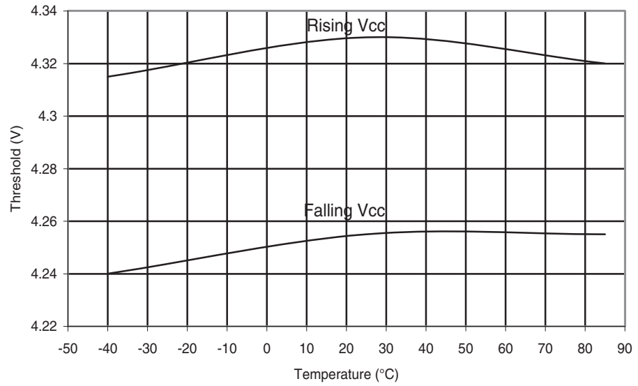
Figure 29-171. ATmega88PA: BOD Thresholds vs. Temperature (BODLEVEL is 4.3 V)
