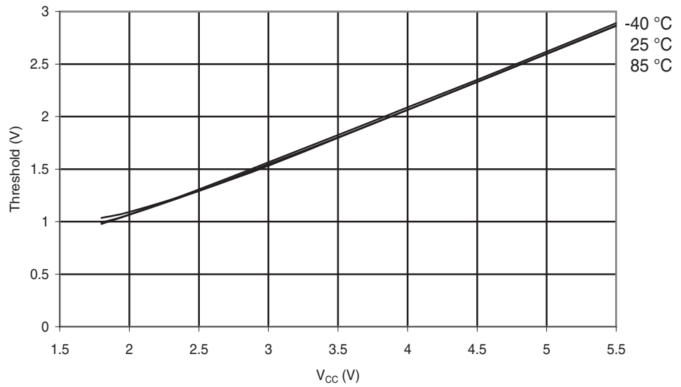
Figure 29-71. ATmega48PA: I/O Pin Input Threshold Voltage vs. V_{CC} ( V_{IH} , I/O Pin read as '1')
