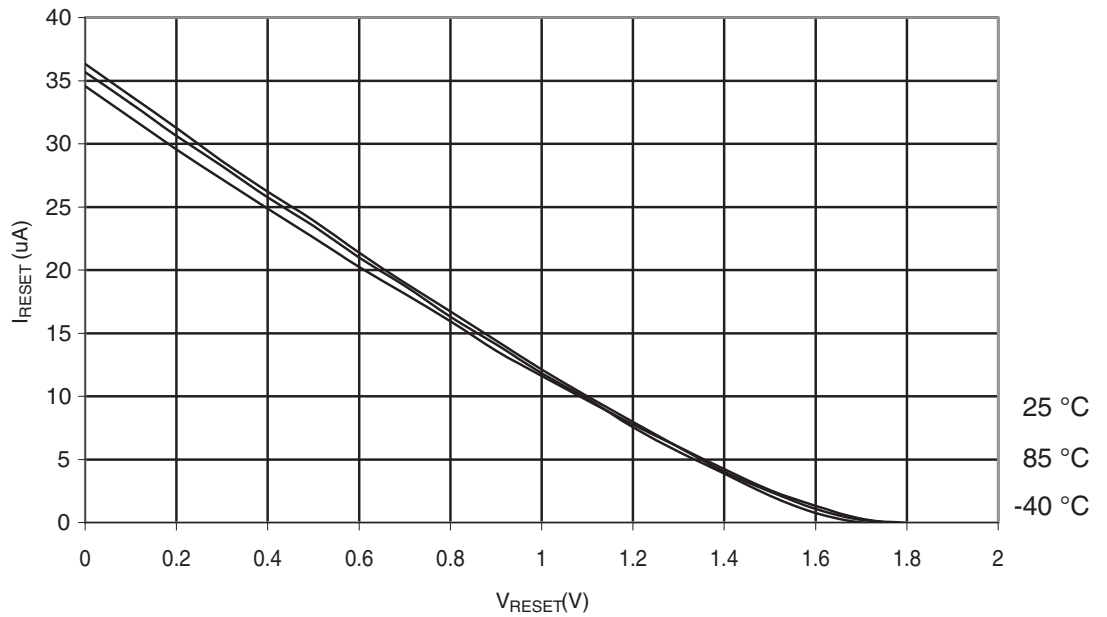
Figure 29-294. ATmega328: Reset Pull-up Resistor Current vs. Reset Pin Voltage ( V_{CC} = 1.8\text{ V} )
