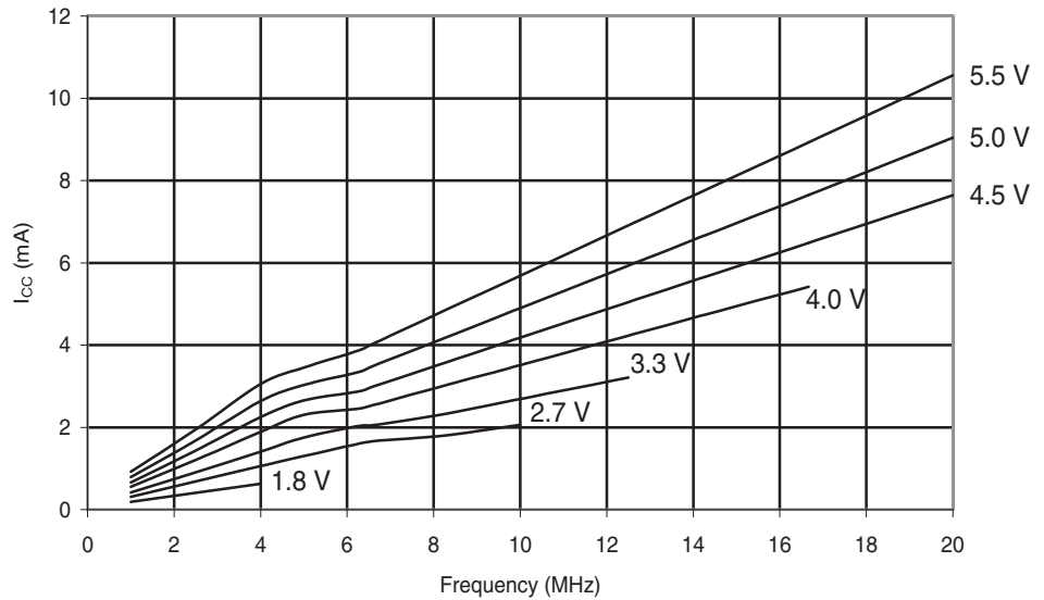
Figure 29-232. ATmega168PA: Active Supply Current vs. Frequency (1-20 MHz)
