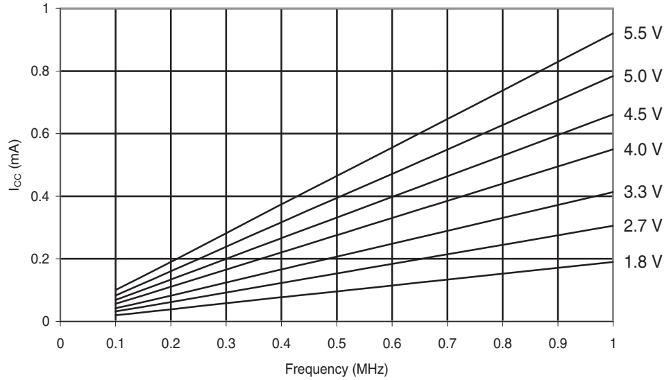
Figure 29-231. ATmega168PA: Active Supply Current vs. Low Frequency (0.1-1.0 MHz)
