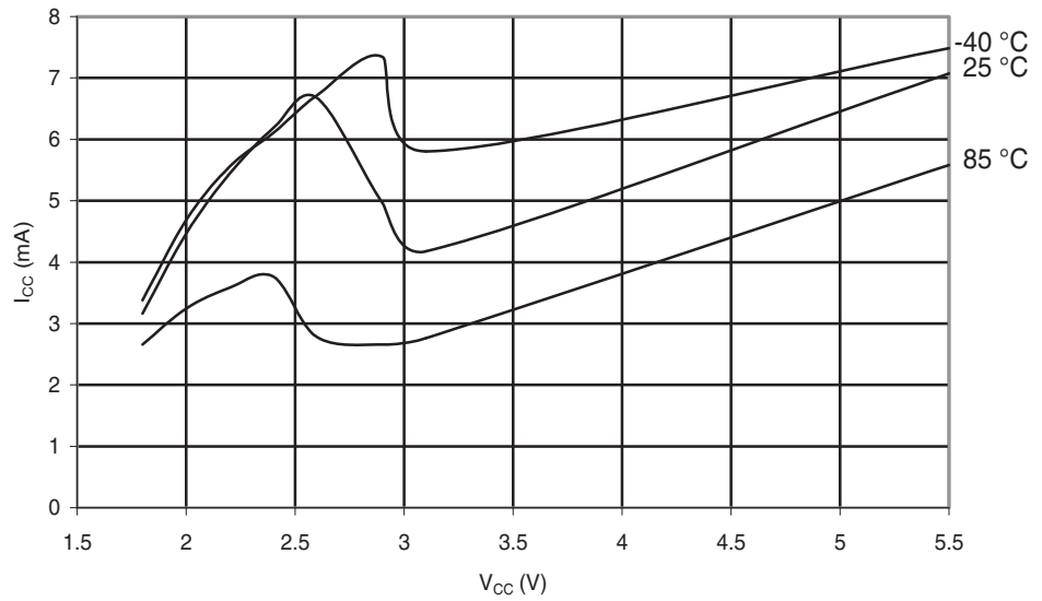
Figure 29-181. ATmega88PA: Programming Current vs. V_{CC}
