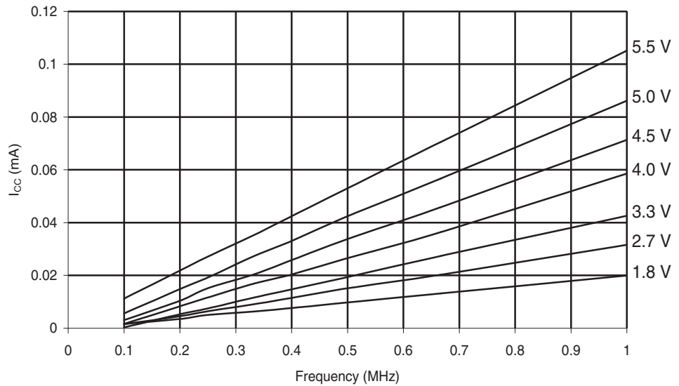
Figure 29-228. ATmega168A: Reset Supply Current vs. Low Frequency (0.1 - 1.0 MHz)
