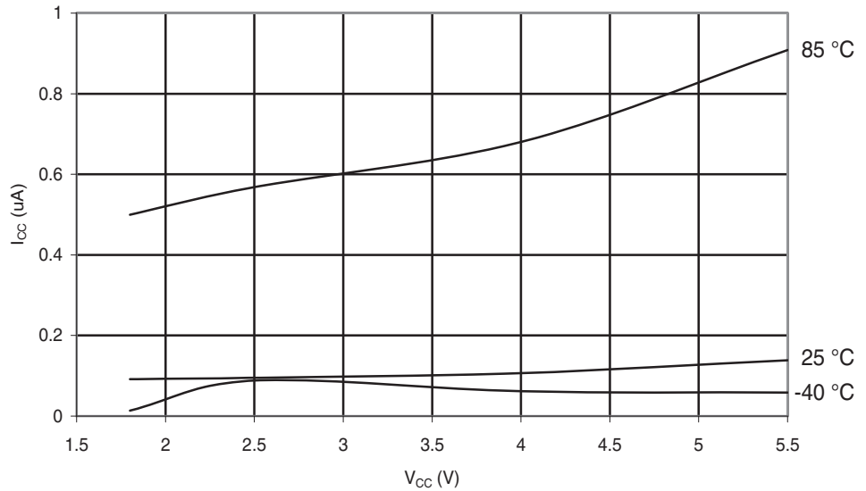
Figure 29-195. ATmega168A: Power-Down Supply Current vs. V_{CC} (Watchdog Timer Disabled)
