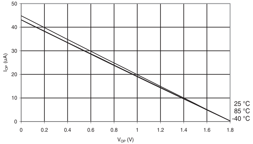
Figure 29-61. ATmega48PA: I/O Pin Pull-up Resistor Current vs. Input Voltage ( V_{CC} = 1.8\text{ V} )
