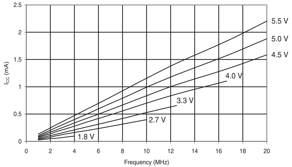
Figure 29-99. ATmega88A: Idle Supply Current vs. Frequency (1-20 MHz)
