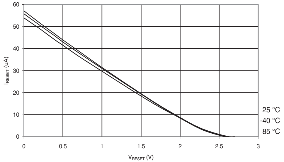
Figure 29-157. ATmega88PA: Reset Pull-up Resistor Current vs. Reset Pin Voltage ( V_{CC} = 2.7\text{ V} )
