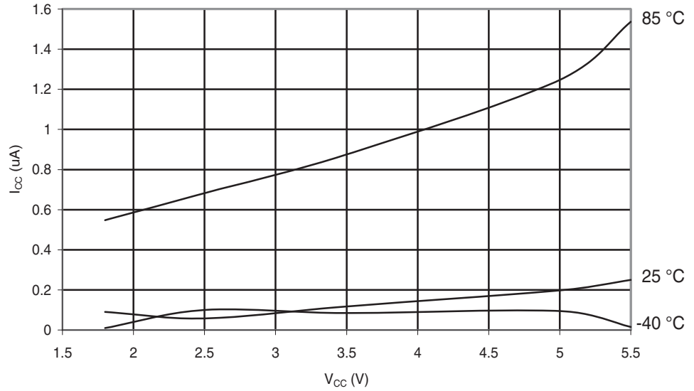
Figure 29-149. ATmega88PA: Power-Down Supply Current vs. V_{CC} (Watchdog Timer Disabled)
