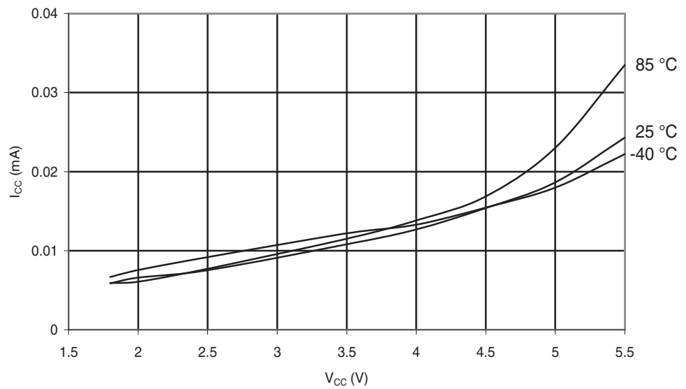
Figure 29-146. ATmega88PA: Idle Supply Current vs. V_{CC} (Internal RC Oscillator, 128 kHz)
