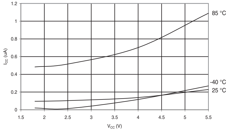
Figure 29-57. ATmega48PA: Power-Down Supply Current vs. V_{CC} (Watchdog Timer Disabled)
