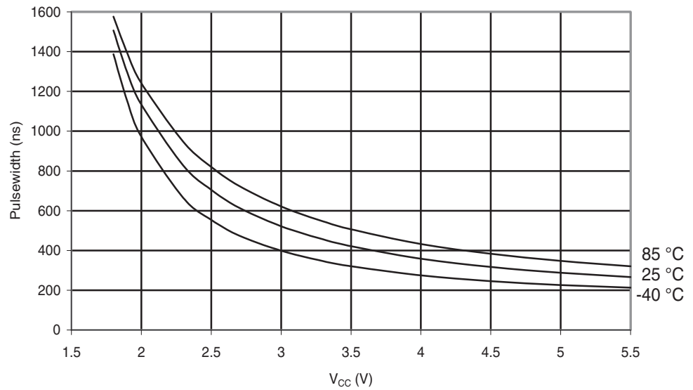
Figure 29-138. ATmega88A: Minimum Reset Pulse width vs. V_{CC}
