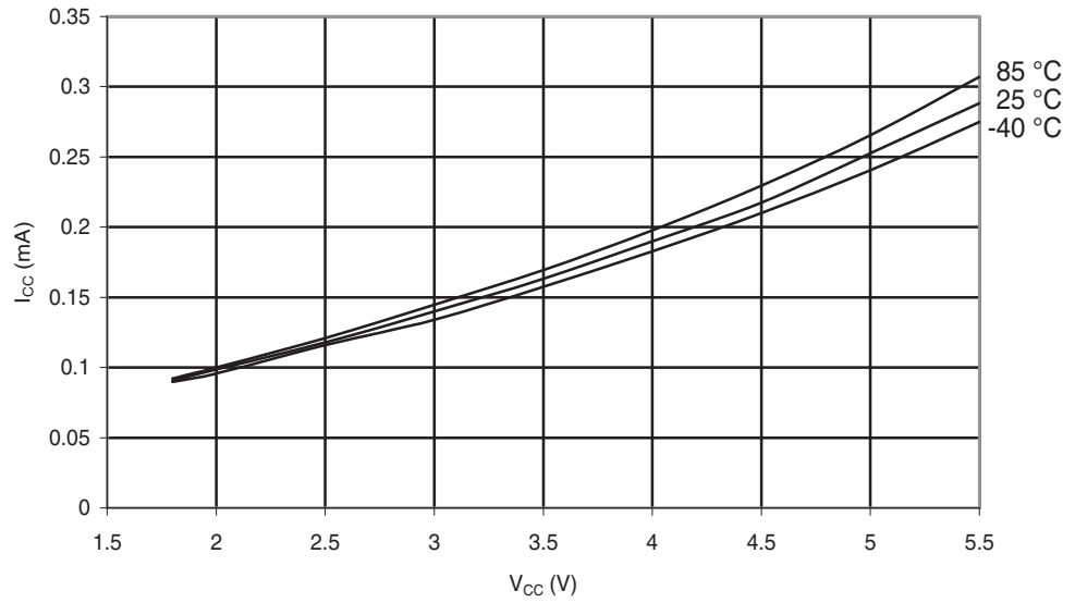
Figure 29-55. ATmega48PA: Idle Supply Current vs. V_{CC} (Internal RC Oscillator, 1 MHz)
