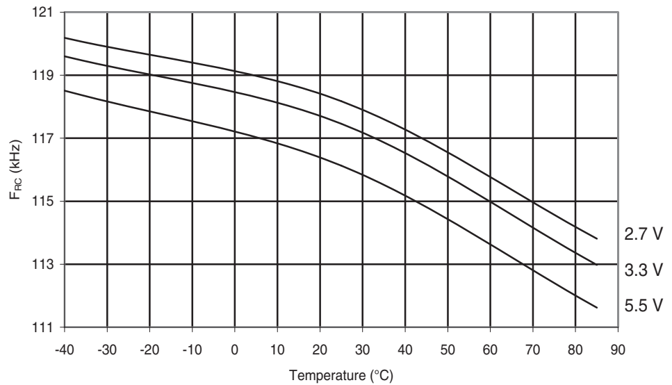
Figure 29-218. ATmega168A: Watchdog Oscillator Frequency vs. Temperature
