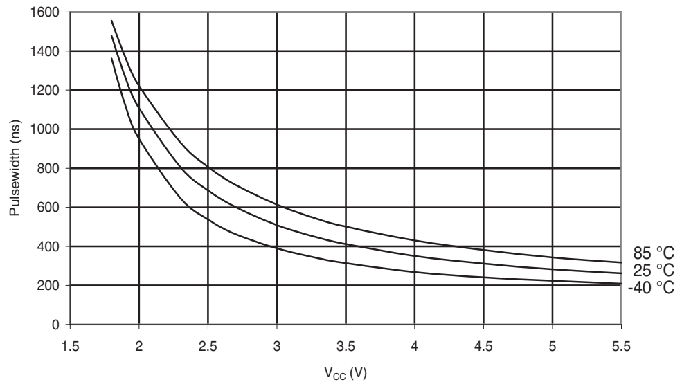
Figure 29-92. ATmega48PA: Minimum Reset Pulse width vs. V_{CC}
