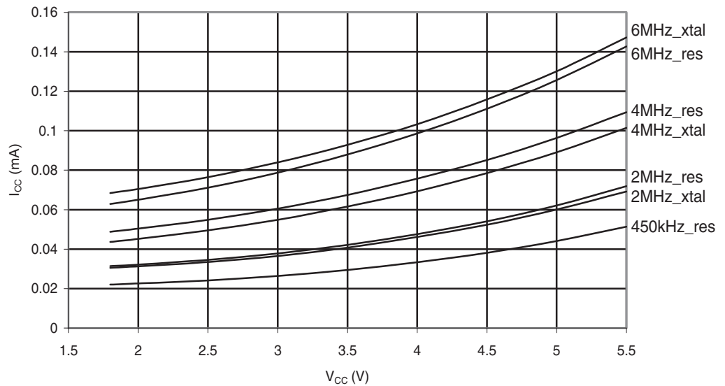
Figure 29-60. ATmega48PA: Standby Supply Current vs. V_{CC} (Watchdog Timer Disabled)
