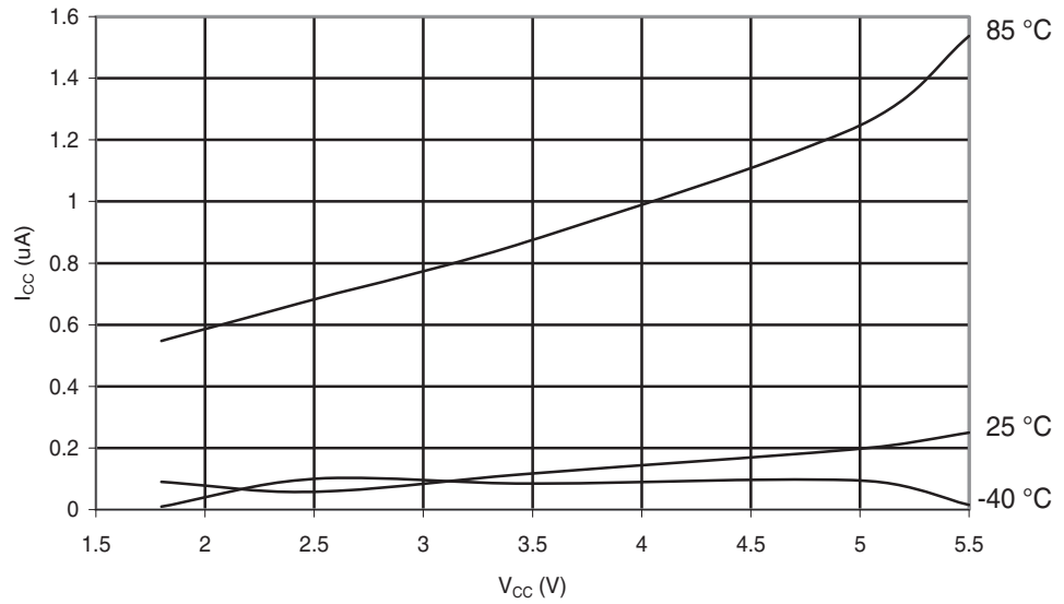
Figure 29-103. ATmega88A: Power-Down Supply Current vs. V_{CC} (Watchdog Timer Disabled)
