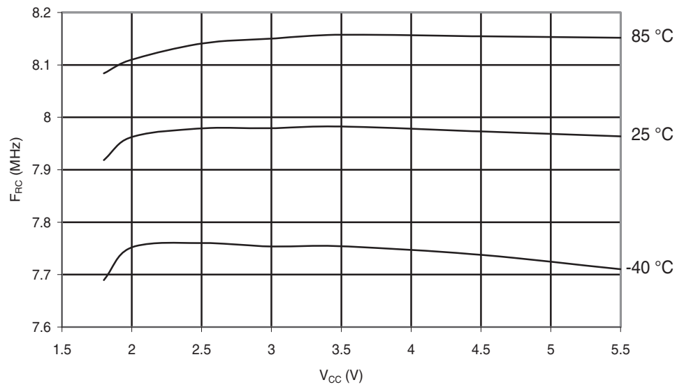
Figure 29-82. ATmega48PA: Calibrated 8 MHz RC Oscillator Frequency vs. V_{CC}
