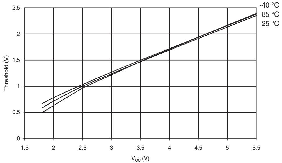
Figure 29-164. ATmega88PA: I/O Pin Input Threshold Voltage vs. V_{CC} ( V_{IL} , I/O Pin read as '0')
