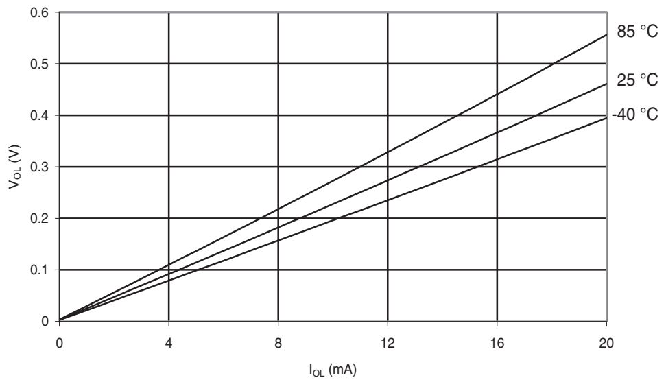
Figure 29-206. ATmega168A: I/O Pin Output Voltage vs. Sink Current ( V_{CC} = 5\text{ V} )
