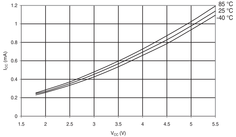
Figure 29-56. ATmega48PA: Idle Supply Current vs. V_{CC} (Internal RC Oscillator, 8 MHz)
