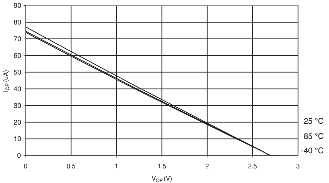
Figure 29-338. ATmega328P: I/O Pin Pull-up Resistor Current vs. Input Voltage ( V_{CC} = 2.7\text{ V} )
