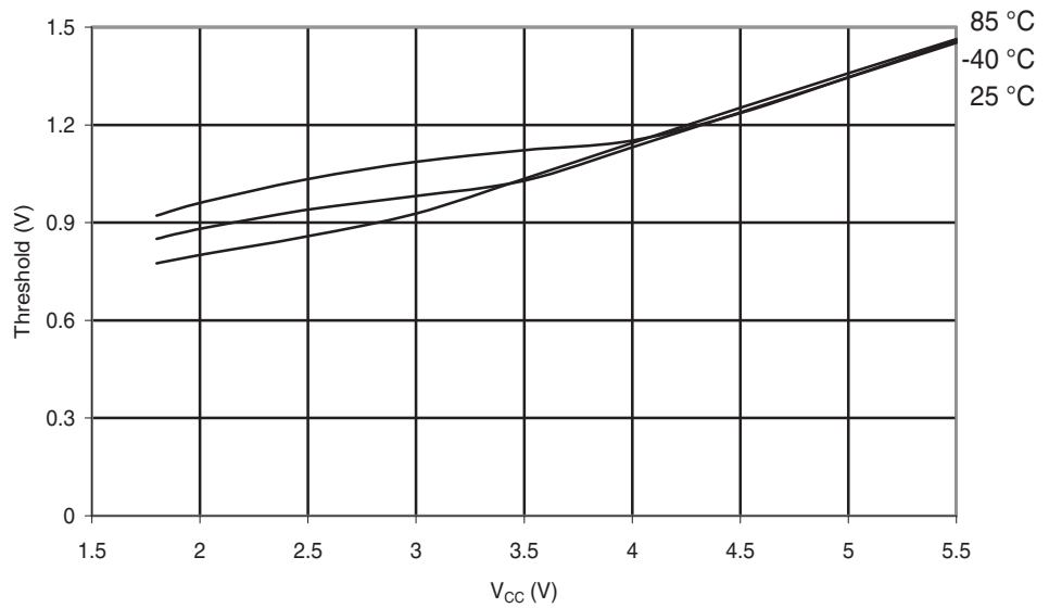
Figure 29-258. ATmega168PA: Reset Input Threshold Voltage vs. V_{CC} ( V_{IH} , I/O Pin read as '1')
