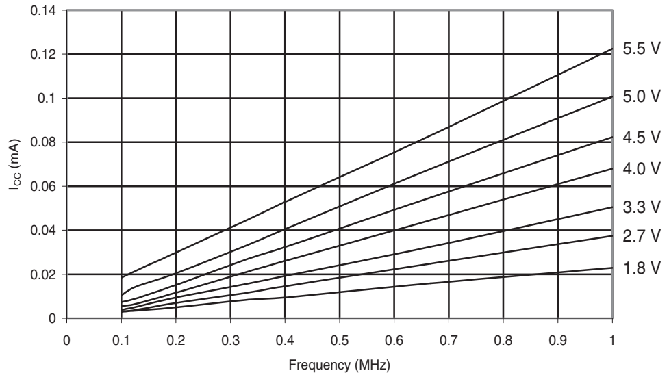
Figure 29-44. ATmega48A: Reset Supply Current vs. Low Frequency (0.1 - 1.0 MHz)
