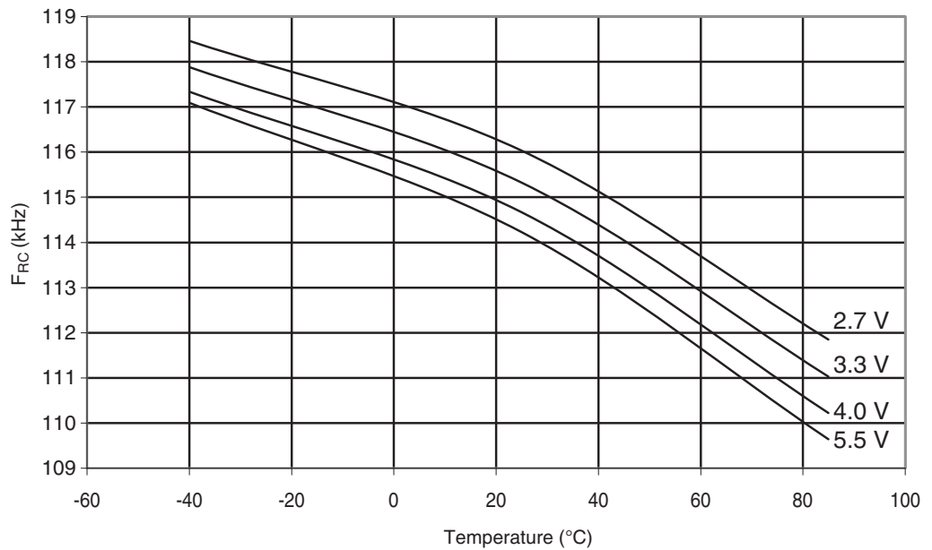
Figure 29-356. ATmega328P: Watchdog Oscillator Frequency vs. Temperature
