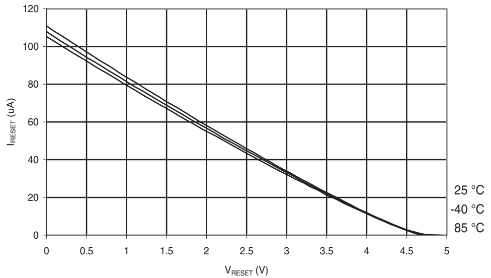
Figure 29-158. ATmega88PA: Reset Pull-up Resistor Current vs. Reset Pin Voltage ( V_{CC} = 5\text{ V} )
