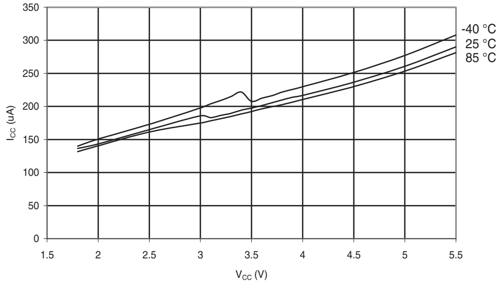
Figure 29-85. ATmega48PA: ADC Current vs. V_{CC} (AREF = AV_{CC} )
