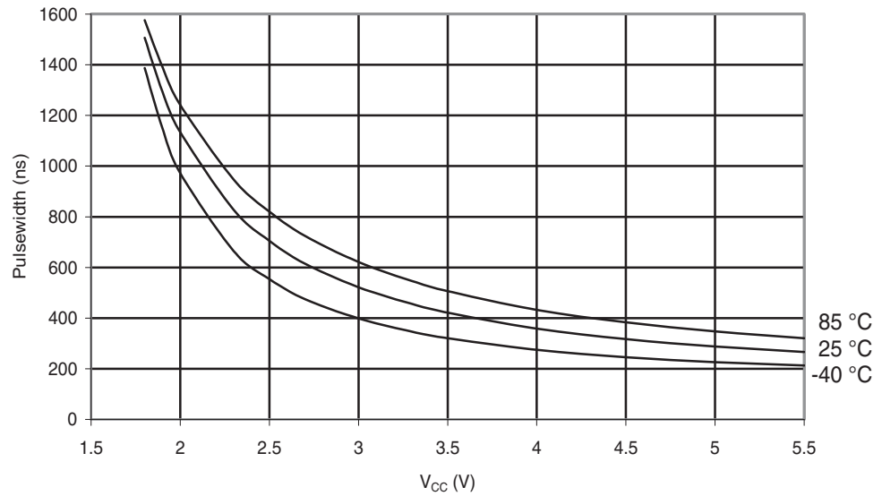
Figure 29-184. ATmega88PA: Minimum Reset Pulse width vs. V_{CC}
