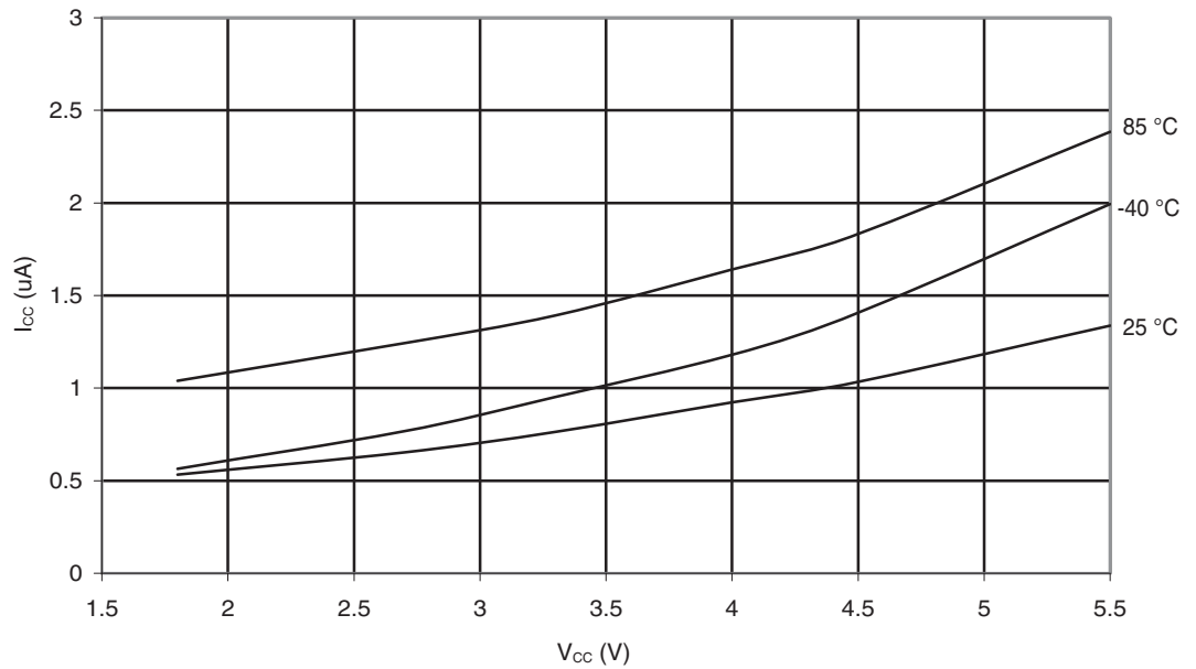
Figure 29-105. ATmega88A: Power-Save Supply Current vs. V_{CC} (Watchdog Timer Disabled and 32 kHz Crystal Oscillator Running)
