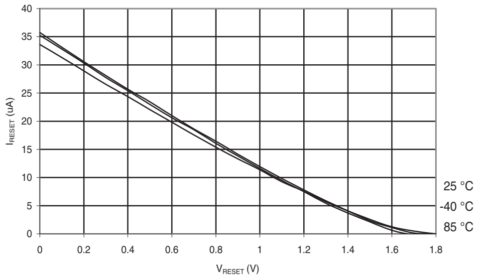
Figure 29-202. ATmega168A: Reset Pull-up Resistor Current vs. Reset Pin Voltage ( V_{CC} = 1.8\text{ V} )
