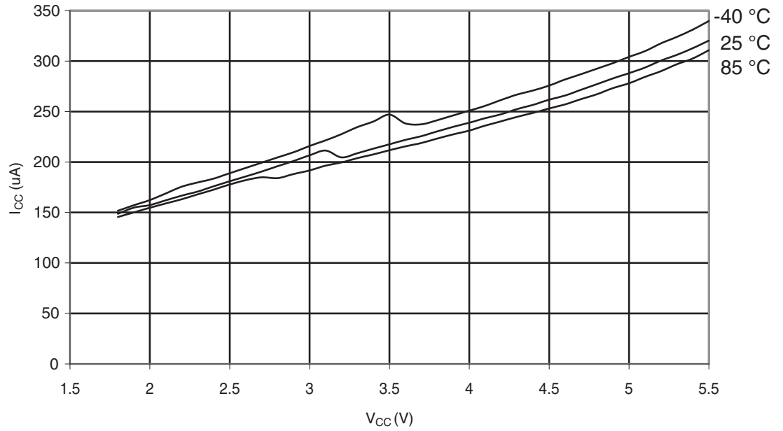
Figure 29-361. ATmega328P: ADC Current vs. V_{CC} (AREF = AV_{CC} )
