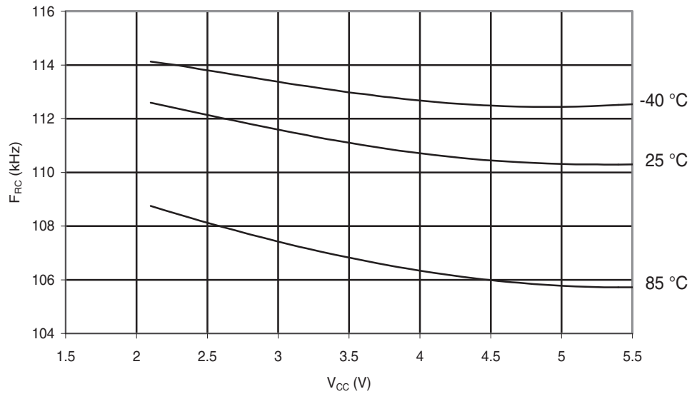
Figure 29-173. ATmega88PA: Watchdog Oscillator Frequency vs. V_{CC}
