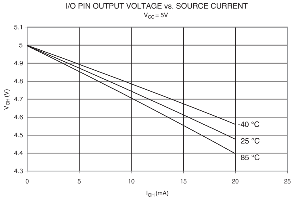
Figure 29-300. ATmega328: I/O Pin Output Voltage vs. Source Current ( V_{CC} = 5\text{ V} )
