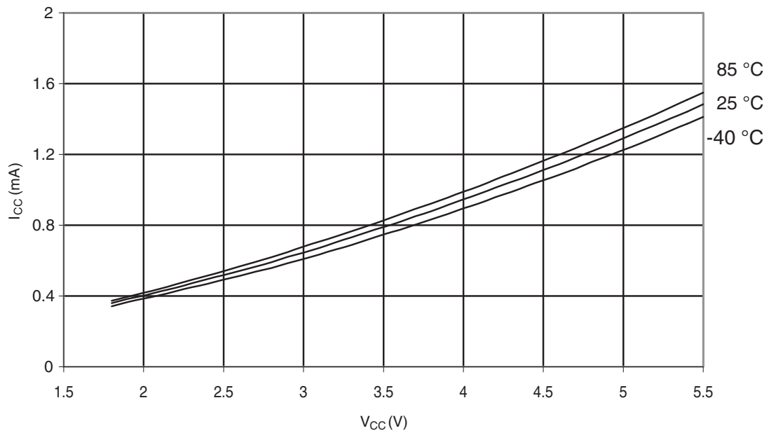
Figure 29-286. ATmega328: Idle Supply Current vs. V_{CC} (Internal RC Oscillator, 8 MHz)
