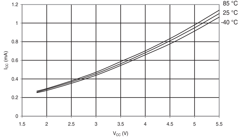
Figure 29-96. ATmega88A: Active Supply Current vs. V_{CC} (Internal RC Oscillator, 1 MHz)
