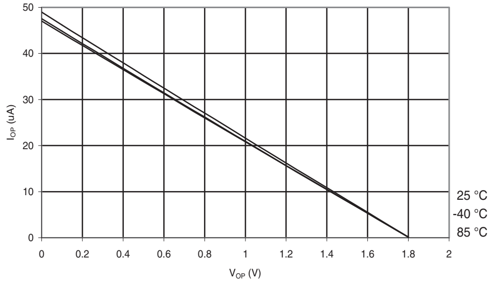
Figure 29-245. ATmega168PA: I/O Pin Pull-up Resistor Current vs. Input Voltage ( V_{CC} = 1.8\text{ V} )
