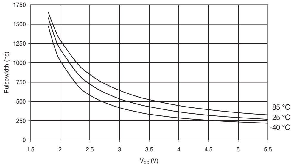
Figure 29-230. ATmega168A: Minimum Reset Pulse width vs. V_{CC}
