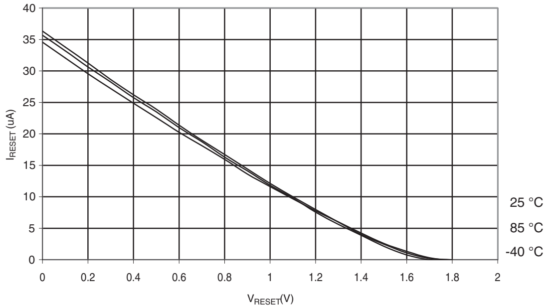
Figure 29-340. ATmega328P: Reset Pull-up Resistor Current vs. Reset Pin Voltage ( V_{CC} = 1.8\text{ V} )
