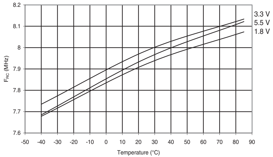
Figure 29-83. ATmega48PA: Calibrated 8 MHz RC Oscillator Frequency vs. Temperature
