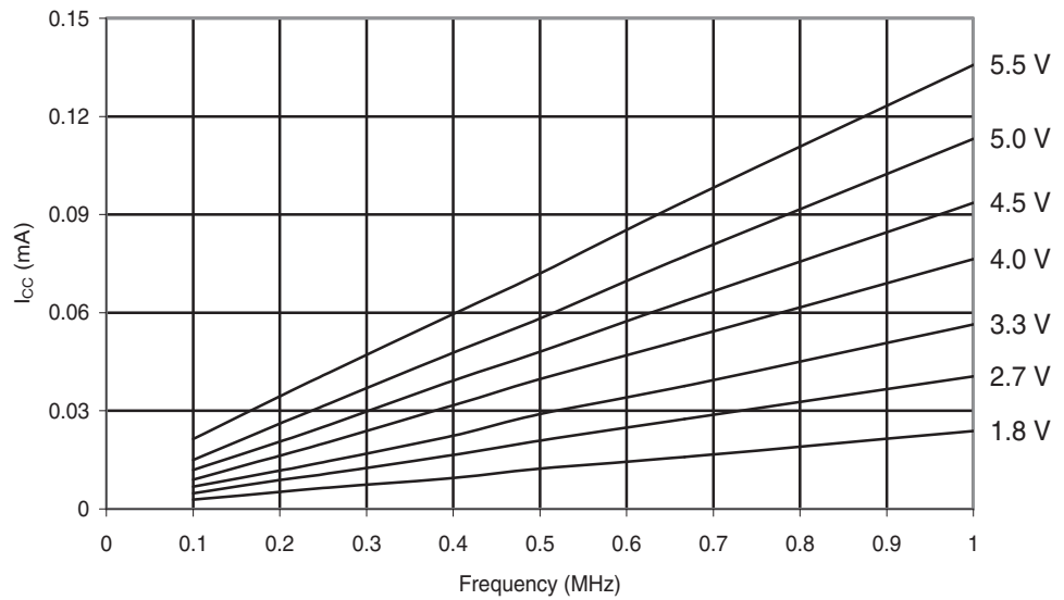
Figure 29-236. ATmega168PA: Idle Supply Current vs. Low Frequency (0.1-1.0 MHz)
