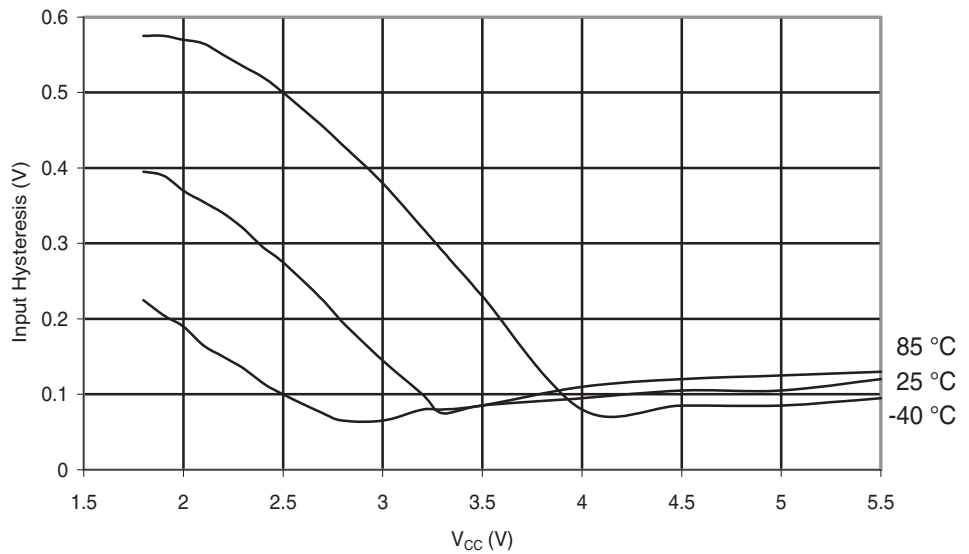
Figure 29-168. ATmega88PA: Reset Pin Input Hysteresis vs. V_{CC}
