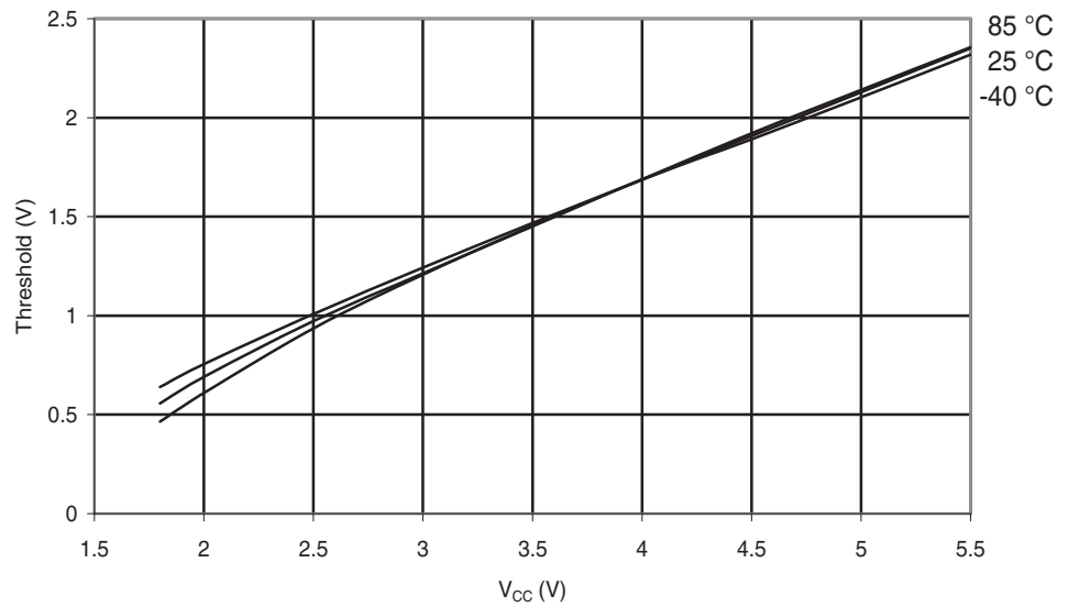
Figure 29-72. ATmega48PA: I/O Pin Input Threshold Voltage vs. V_{CC} ( V_{IL} , I/O Pin read as '0')
