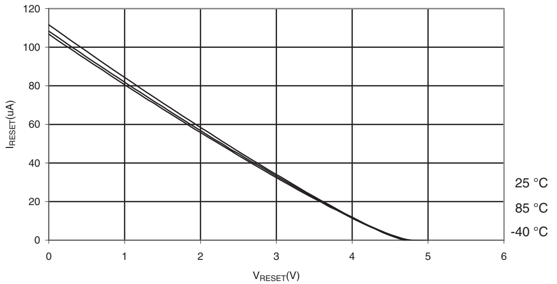
Figure 29-342. ATmega328P: Reset Pull-up Resistor Current vs. Reset Pin Voltage ( V_{CC} = 5\text{ V} )
