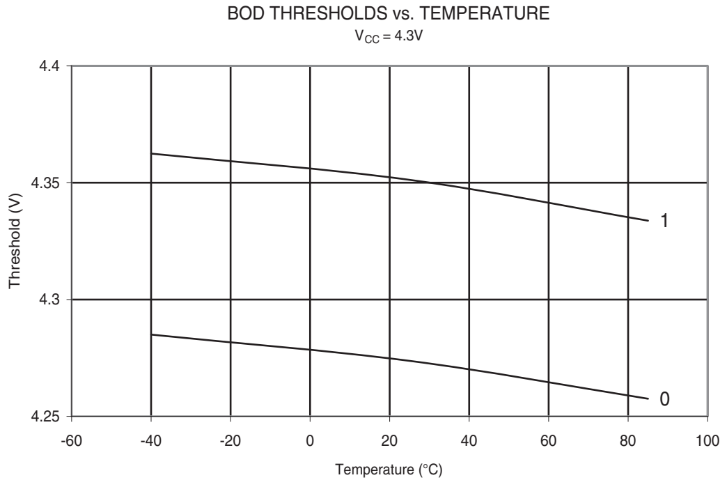
Figure 29-309. ATmega328: BOD Thresholds vs. Temperature (BODLEVEL is 4.3 V)
