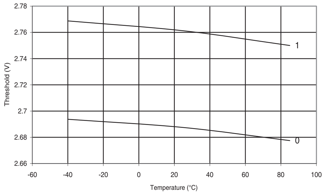
Figure 29-354. ATmega328P: BOD Thresholds vs. Temperature (BODLEVEL is 2.7 V)
