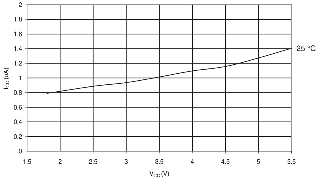
Figure 29-335. ATmega328P: Power-Save Supply Current vs. V_{CC} (Watchdog Timer Disabled and 32 kHz Crystal Oscillator Running)
