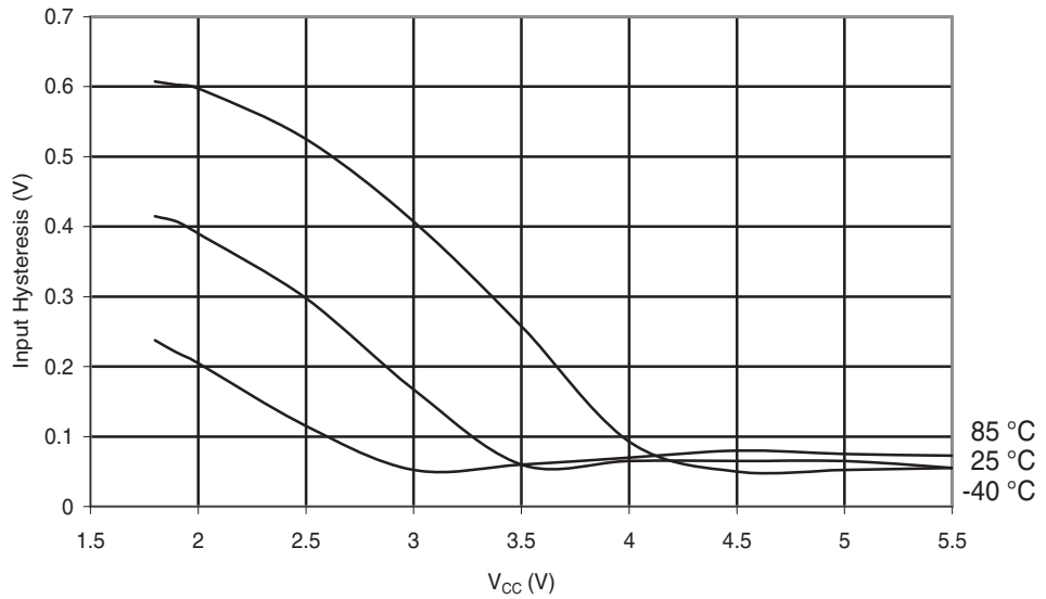
Figure 29-76. ATmega48PA: Reset Pin Input Hysteresis vs. V_{CC}
