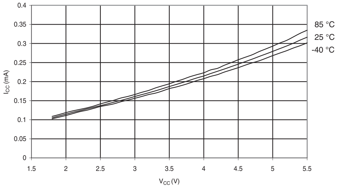
Figure 29-331. ATmega328P: Idle Supply Current vs. V_{CC} (Internal RC Oscillator, 1 MHz)
