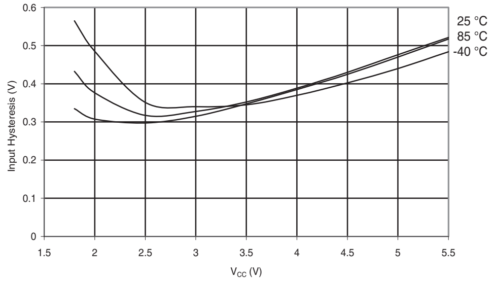
Figure 29-165. ATmega88PA: I/O Pin Input Hysteresis vs. V_{CC}
