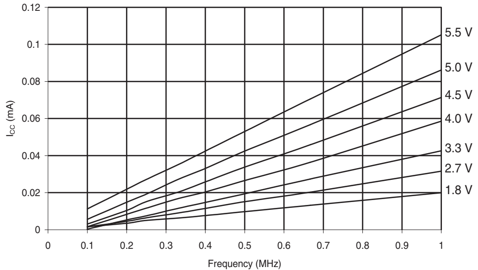
Figure 29-274. ATmega168PA: Reset Supply Current vs. Low Frequency (0.1 - 1.0 MHz)
