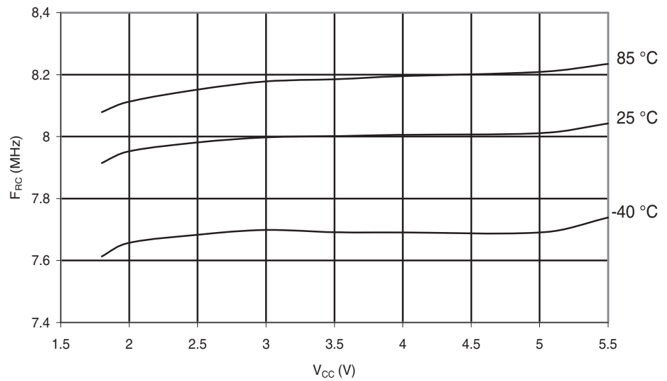
Figure 29-266. ATmega168PA: Calibrated 8 MHz RC Oscillator Frequency vs. V_{CC}
