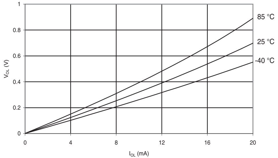
Figure 29-67. ATmega48PA: I/O Pin Output Voltage vs. Sink Current ( V_{CC} = 3\text{ V} )
