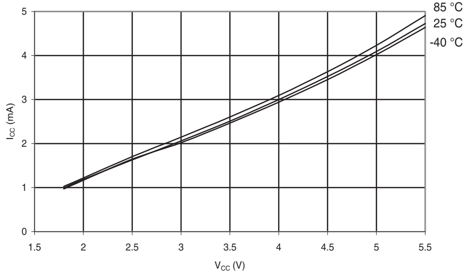
Figure 29-97. ATmega88A: Active Supply Current vs. V_{CC} (Internal RC Oscillator, 8 MHz)
