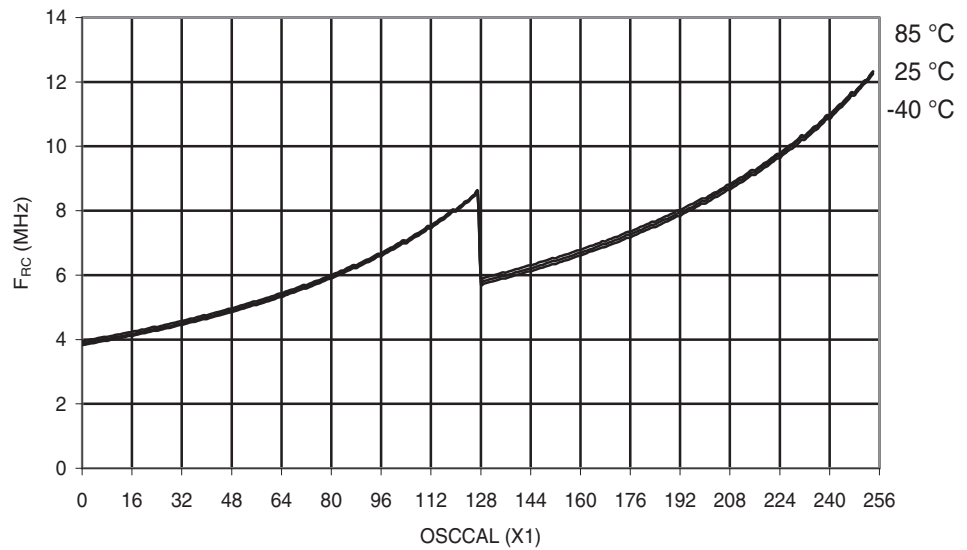
Figure 29-176. ATmega88PA: Calibrated 8 MHz RC Oscillator Frequency vs. OSCCAL Value
