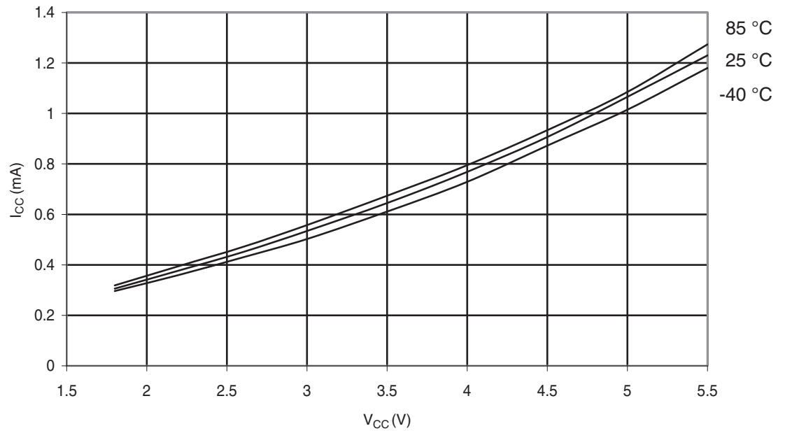
Figure 29-326. ATmega328P: Active Supply Current vs. V_{CC} (Internal RC Oscillator, 1 MHz)
