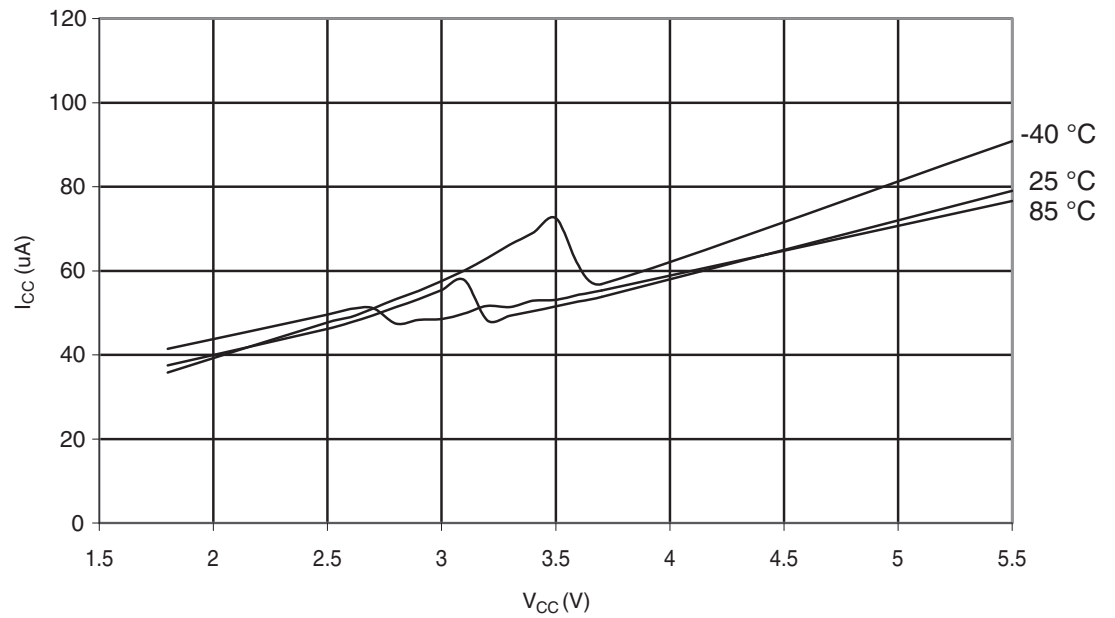
Figure 29-316. ATmega328: Analog Comparator Current vs. V_{CC}
