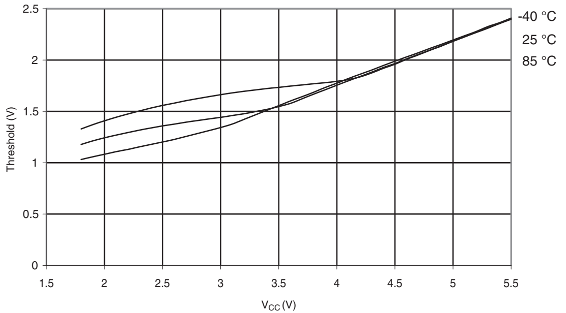
Figure 29-350. ATmega328P: Reset Input Threshold Voltage vs. V_{CC} ( V_{IH} , I/O Pin read as '1')
