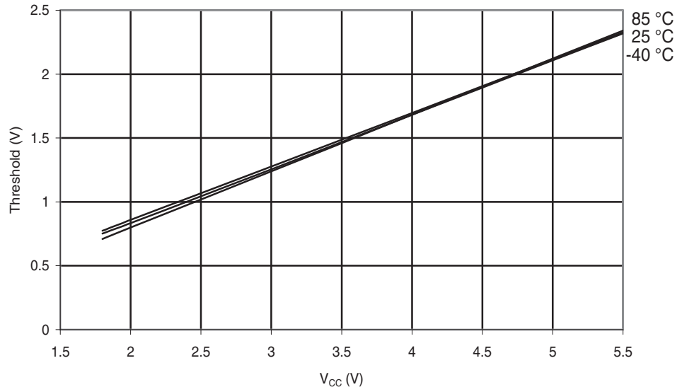
Figure 29-75. ATmega48PA: Reset Input Threshold Voltage vs. V_{CC} ( V_{IL} , I/O Pin read as '0')
