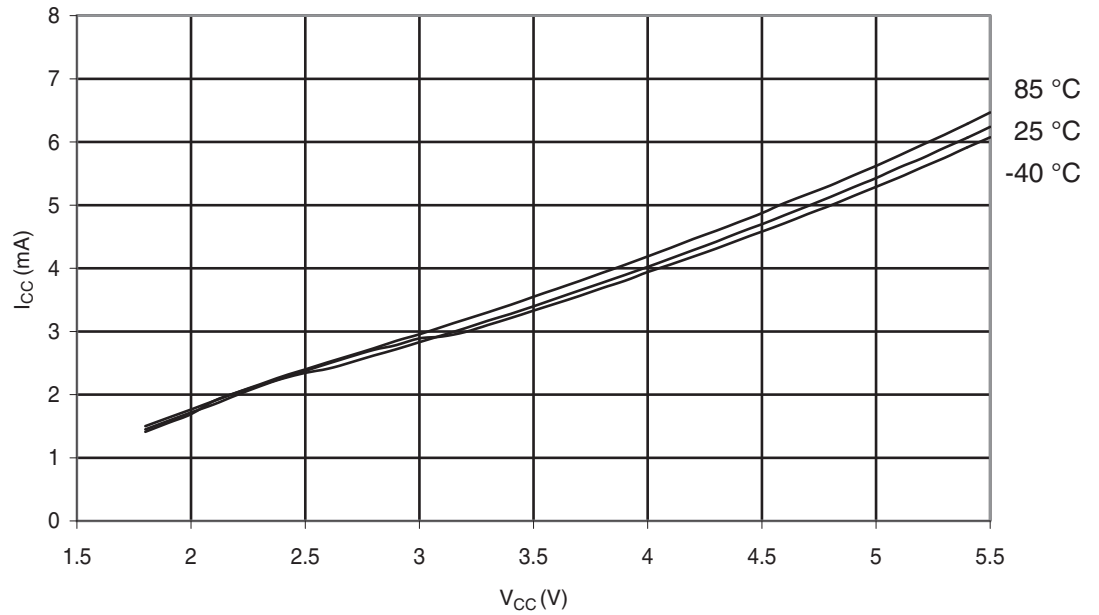
Figure 29-281. ATmega328: Active Supply Current vs. V_{CC} (Internal RC Oscillator, 8 MHz)
