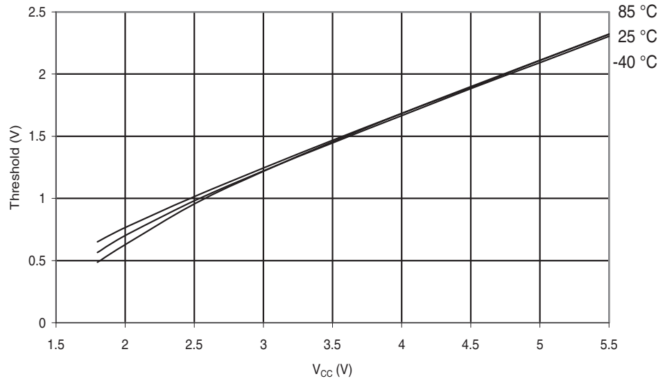
Figure 29-256. ATmega168PA: I/O Pin Input Threshold Voltage vs. V_{CC} ( V_{IL} , I/O Pin read as '0')
