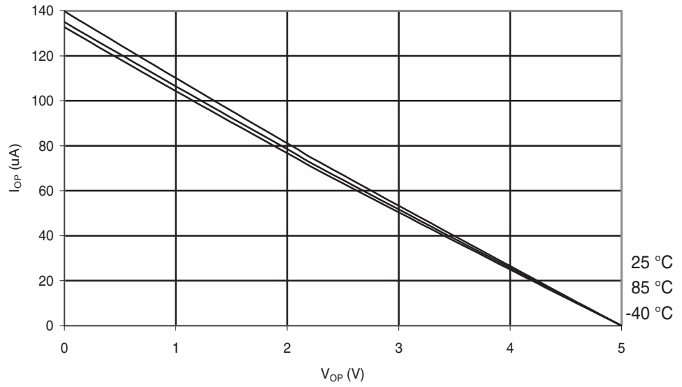
Figure 29-155. ATmega88PA: I/O Pin Pull-up Resistor Current vs. Input Voltage ( V_{CC} = 5\text{ V} )
