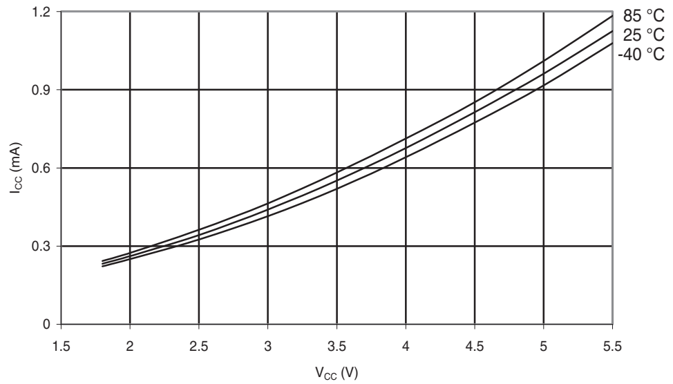
Figure 29-240. ATmega168PA: Idle Supply Current vs. V_{CC} (Internal RC Oscillator, 8 MHz)
