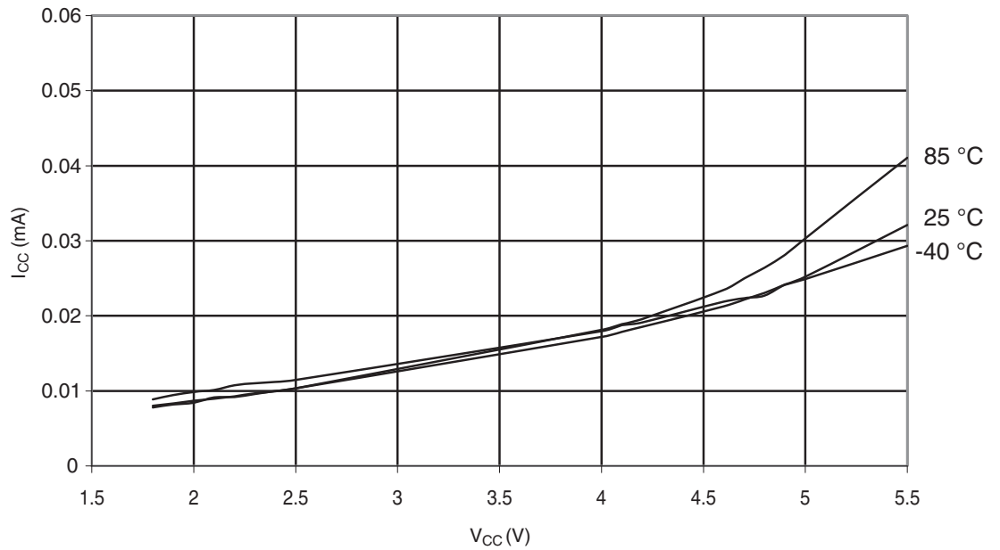
Figure 29-330. ATmega328P: Idle Supply Current vs. V_{CC} (Internal RC Oscillator, 128 kHz)
