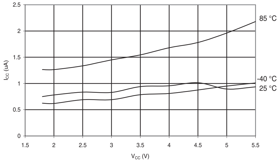
Figure 29-197. ATmega168A: Power-Save Supply Current vs. V_{CC} (Watchdog Timer Disabled and 32 kHz Crystal Oscillator Running)
