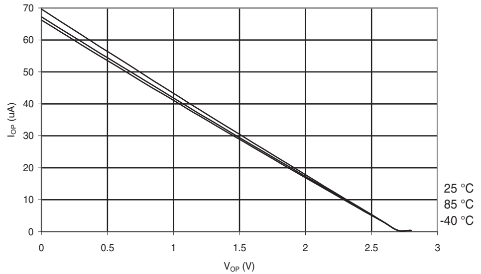
Figure 29-62. ATmega48PA: I/O Pin Pull-up Resistor Current vs. Input Voltage ( V_{CC} = 2.7\text{ V} )
