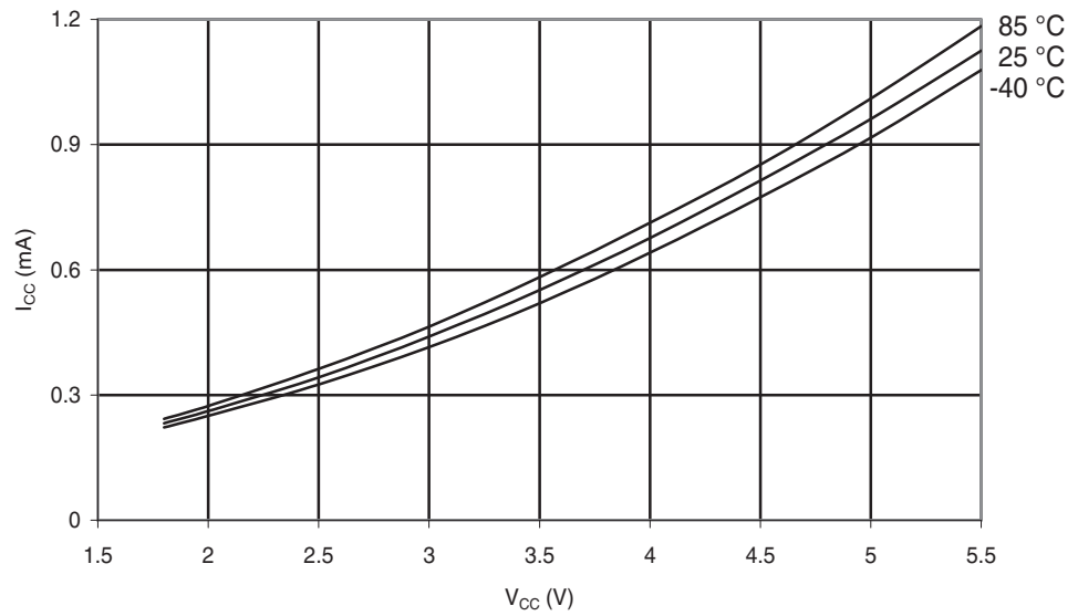
Figure 29-194. ATmega168A: Idle Supply Current vs. V_{CC} (Internal RC Oscillator, 8 MHz)
