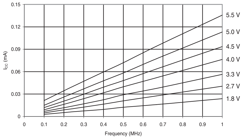
Figure 29-190. ATmega168A: Idle Supply Current vs. Low Frequency (0.1-1.0 MHz)
