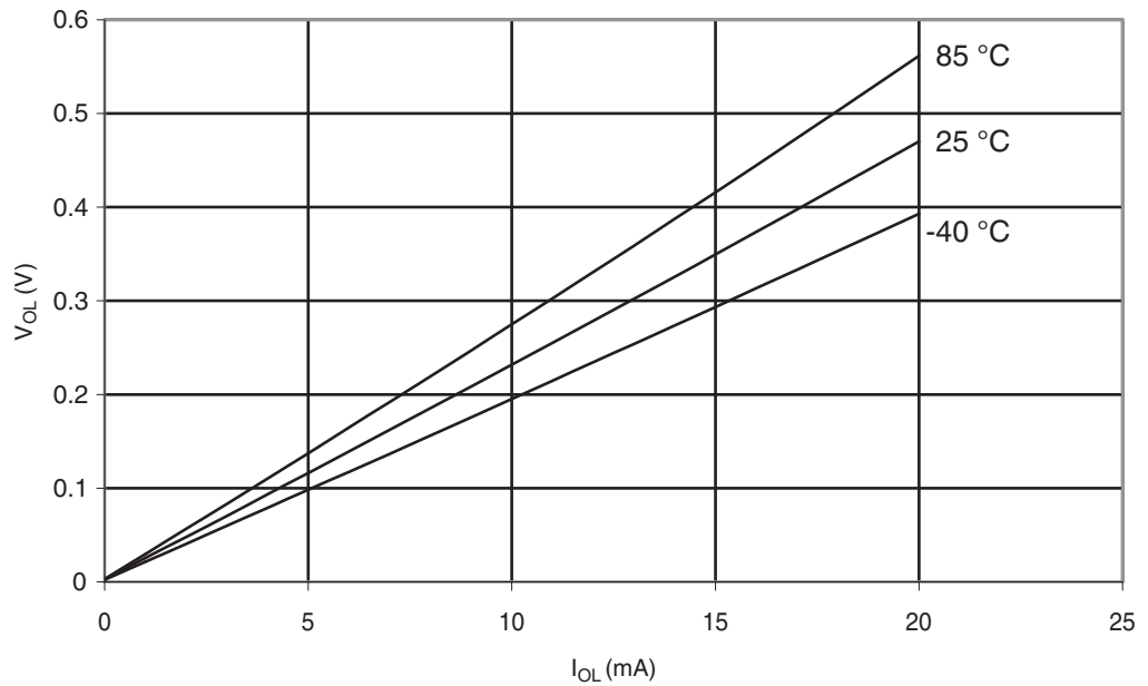
Figure 29-344. ATmega328P: I/O Pin Output Voltage vs. Sink Current ( V_{CC} = 5\text{ V} )
