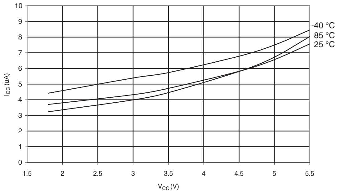
Figure 29-334. ATmega328P: Power-Down Supply Current vs. V_{CC} (Watchdog Timer Enabled)
