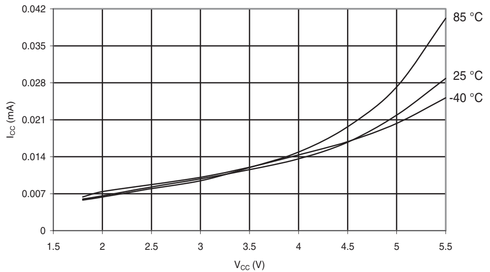
Figure 29-54. ATmega48PA: Idle Supply Current vs. V_{CC} (Internal RC Oscillator, 128 kHz)
