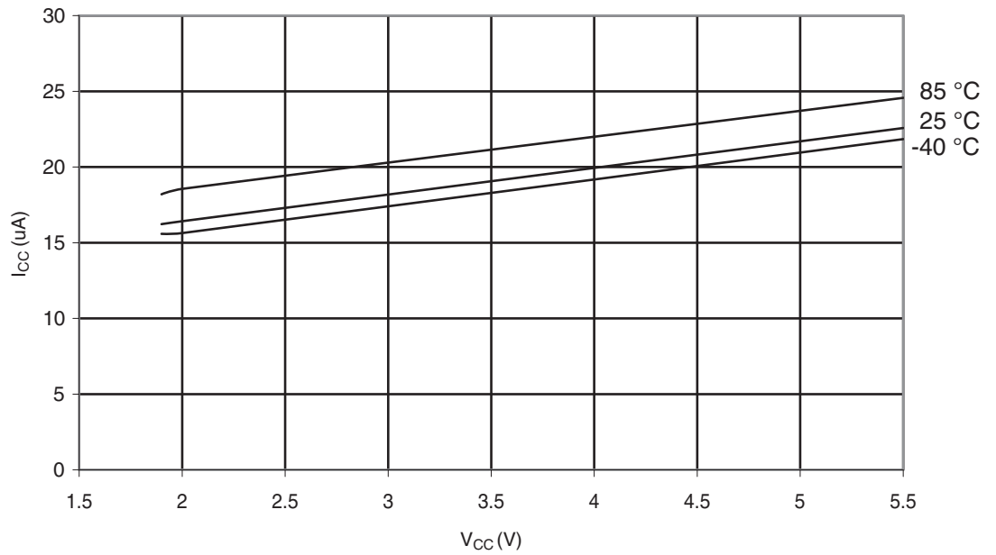
Figure 29-364. ATmega328P: Brownout Detector Current vs. V_{CC}
