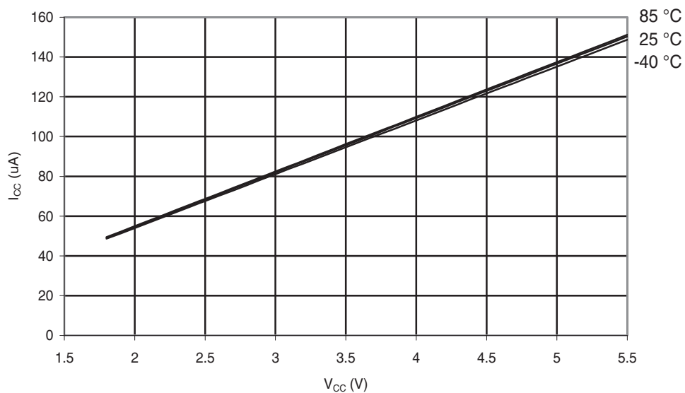
Figure 29-179. ATmega88PA: AREF External Reference Current vs. V_{CC}
