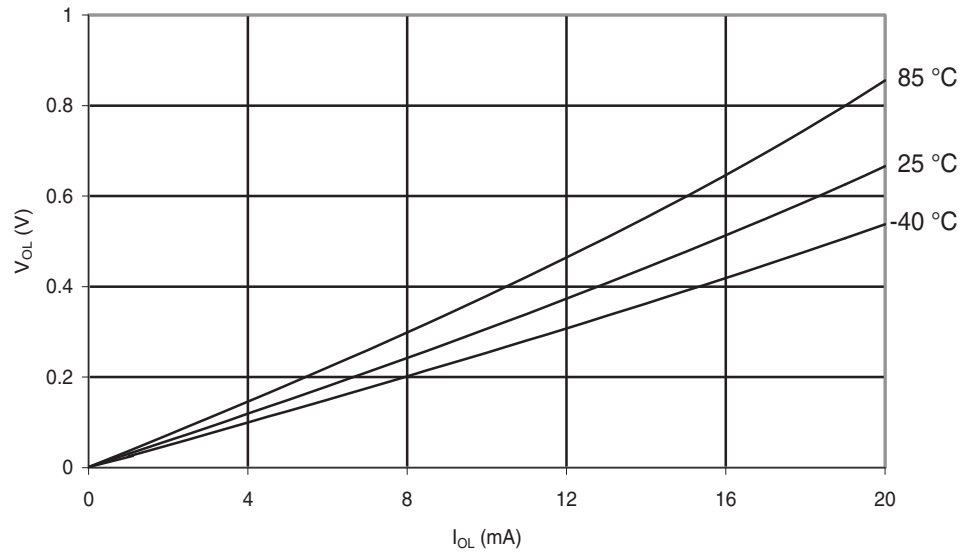
Figure 29-205. ATmega168A: I/O Pin Output Voltage vs. Sink Current ( V_{CC} = 3\text{ V} )
