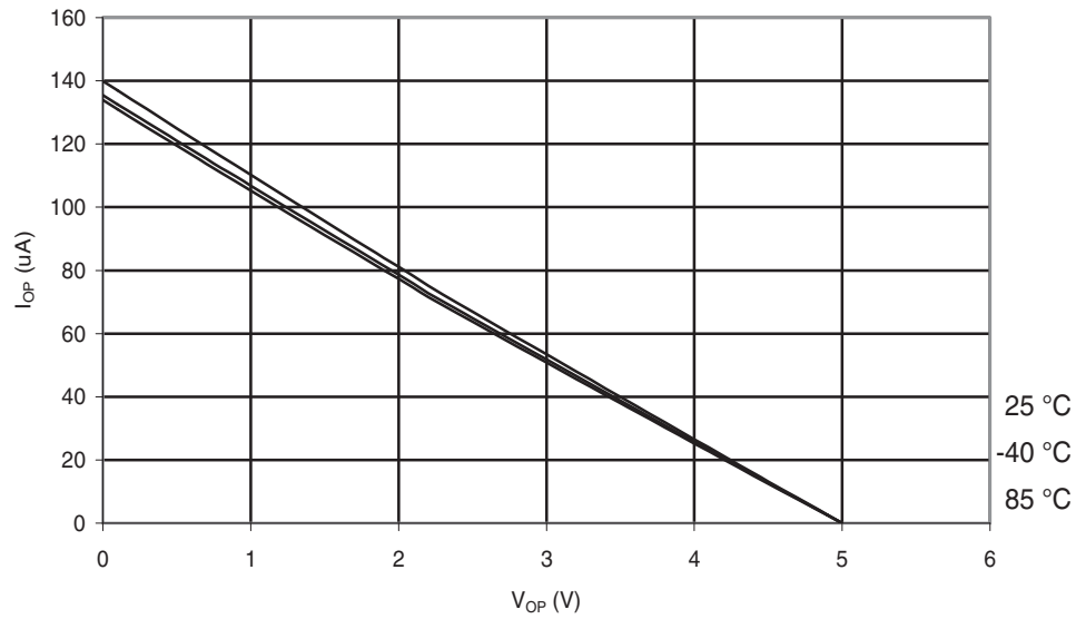
Figure 29-201. ATmega168A: I/O Pin Pull-up Resistor Current vs. Input Voltage ( V_{CC} = 5\text{ V} )
