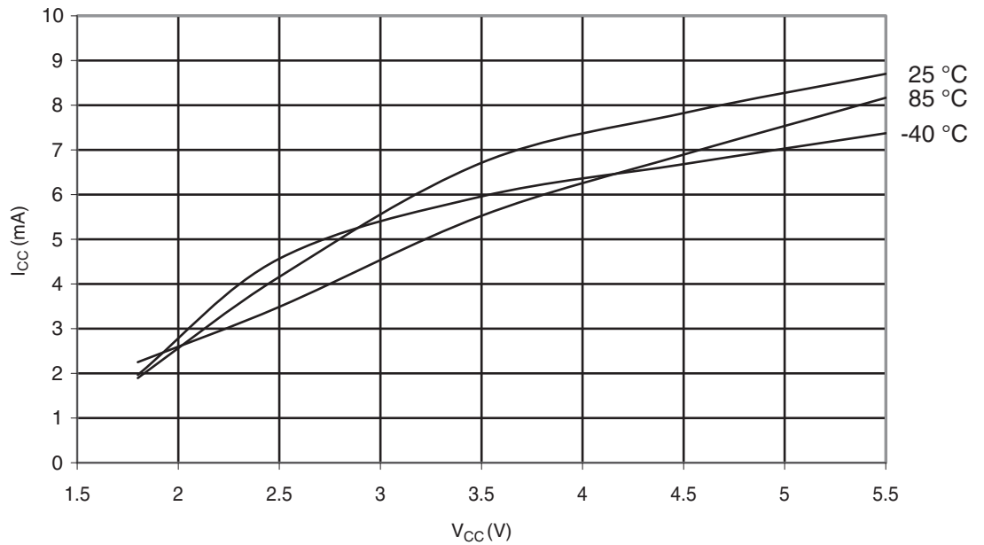
Figure 29-365. ATmega328P: Programming Current vs. V_{CC}
