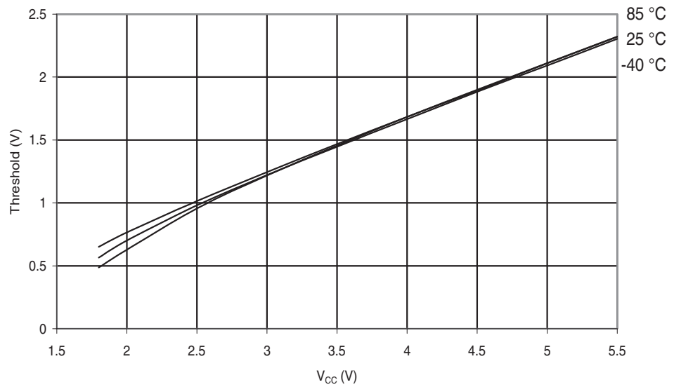
Figure 29-210. ATmega168A: I/O Pin Input Threshold Voltage vs. V_{CC} ( V_{IL} , I/O Pin read as '0')
