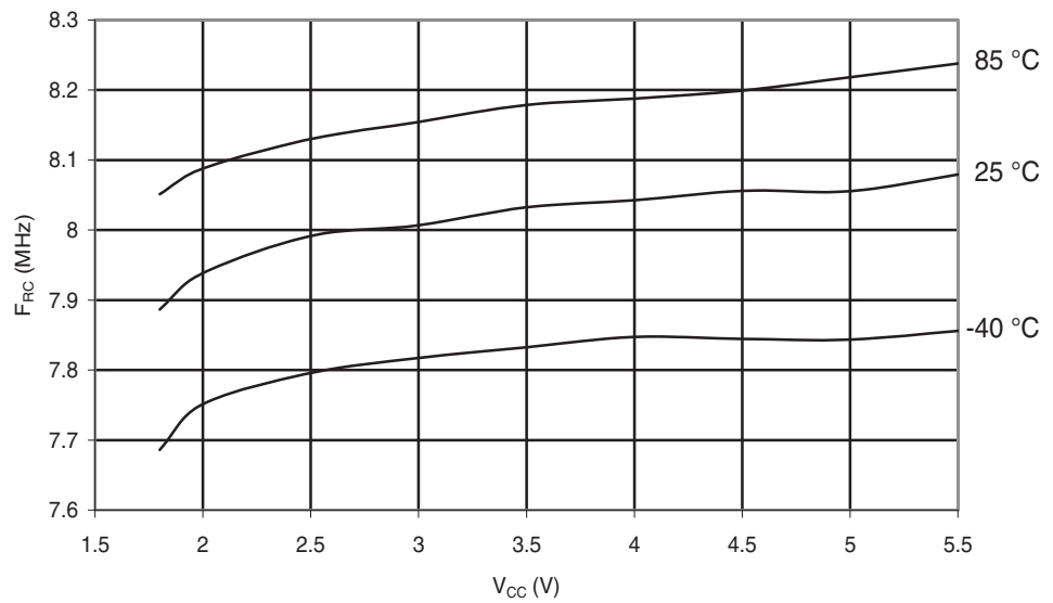
Figure 29-128. ATmega88A: Calibrated 8 MHz RC Oscillator Frequency vs. V_{CC}
