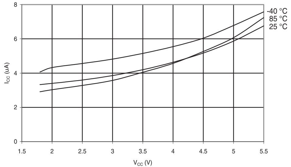
Figure 29-58. ATmega48PA: Power-Down Supply Current vs. V_{CC} (Watchdog Timer Enabled)
