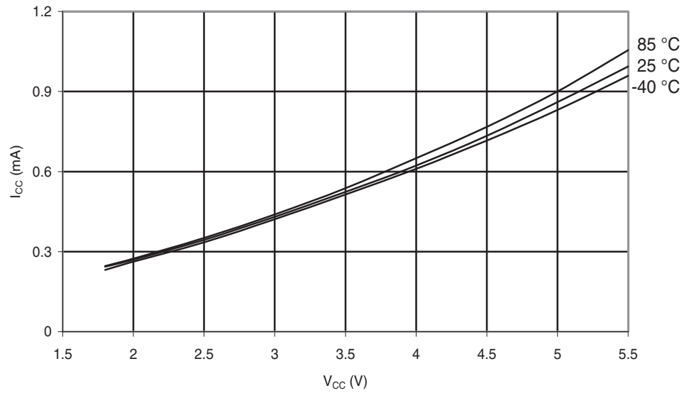
Figure 29-148. ATmega88PA: Idle Supply Current vs. V_{CC} (Internal RC Oscillator, 8 MHz)
