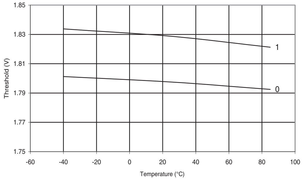
Figure 29-353. ATmega328P: BOD Thresholds vs. Temperature (BODLEVEL is 1.8 V)
