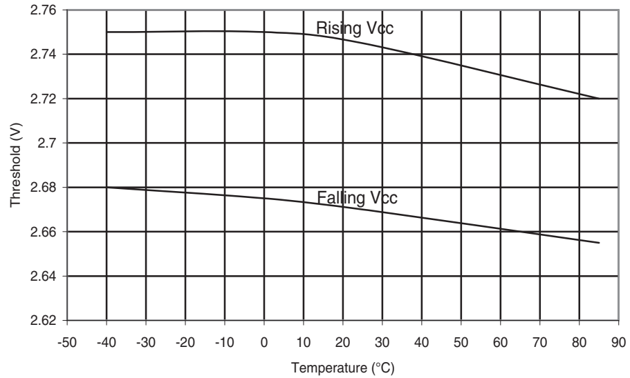
Figure 29-78. ATmega48PA: BOD Thresholds vs. Temperature (BODLEVEL is 2.7 V)
