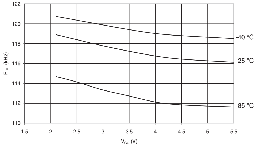
Figure 29-265. ATmega168PA: Watchdog Oscillator Frequency vs. V_{CC}
