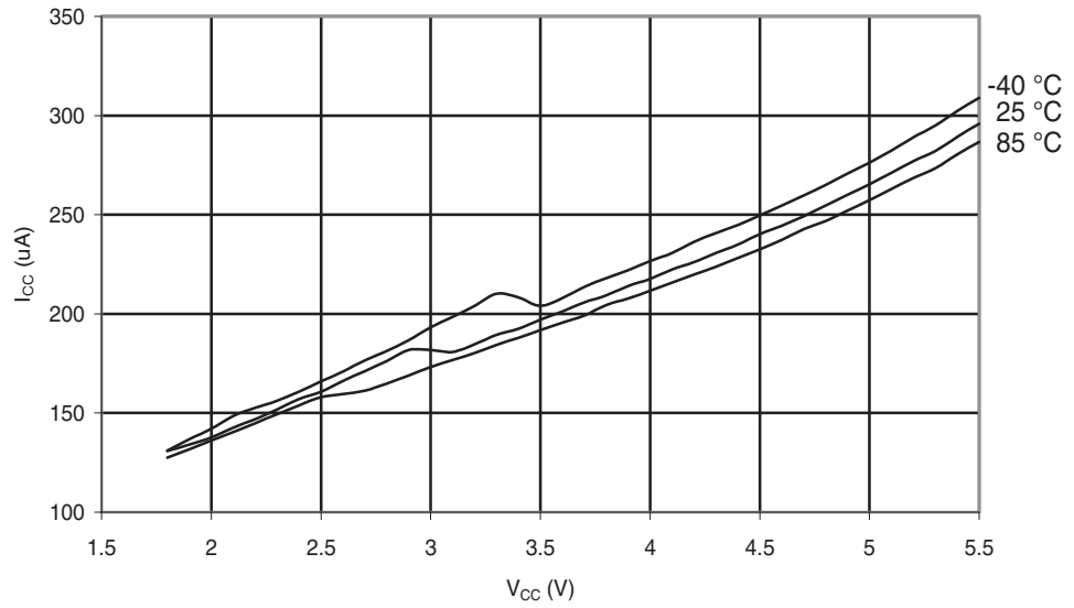
Figure 29-223. ATmega168A: ADC Current vs. V_{CC} (AREF = AV_{CC} )
