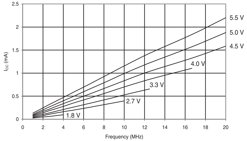
Figure 29-145. ATmega88PA: Idle Supply Current vs. Frequency (1 - 20 MHz)
