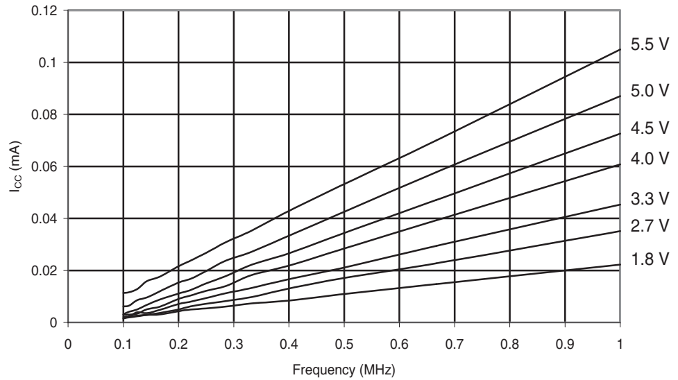
Figure 29-182. ATmega88PA: Reset Supply Current vs. Low Frequency (0.1 - 1.0 MHz)
