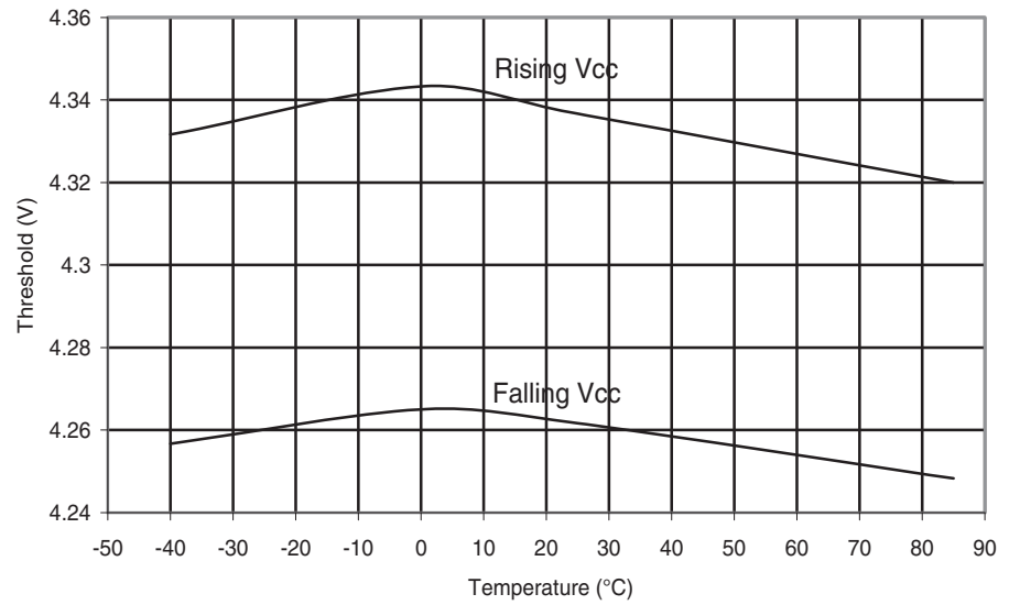
Figure 29-79. ATmega48PA: BOD Thresholds vs. Temperature (BODLEVEL is 4.3 V)
