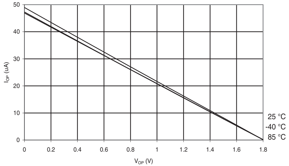
Figure 29-107. ATmega88A: I/O Pin Pull-up Resistor Current vs. Input Voltage ( V_{CC} = 1.8\text{ V} )
