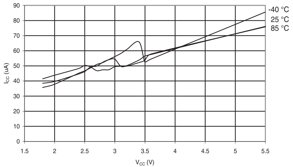
Figure 29-40. ATmega48A: Analog Comparator Current vs. V_{CC}
