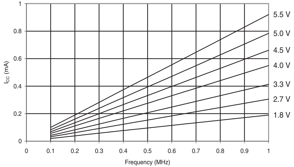
Figure 29-185. ATmega168A: Active Supply Current vs. Low Frequency (0.1-1.0 MHz)
