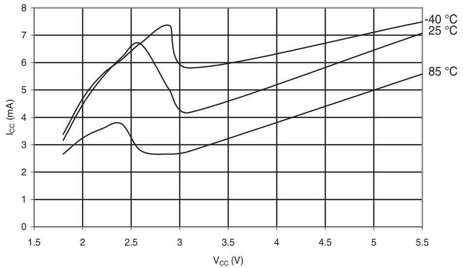
Figure 29-135. ATmega88A: Programming Current vs. V_{CC}
