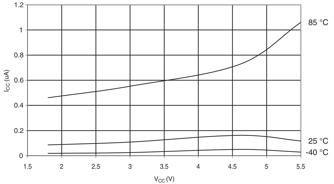
Figure 29-287. ATmega328: Power-Down Supply Current vs. V_{CC} (Watchdog Timer Disabled)
