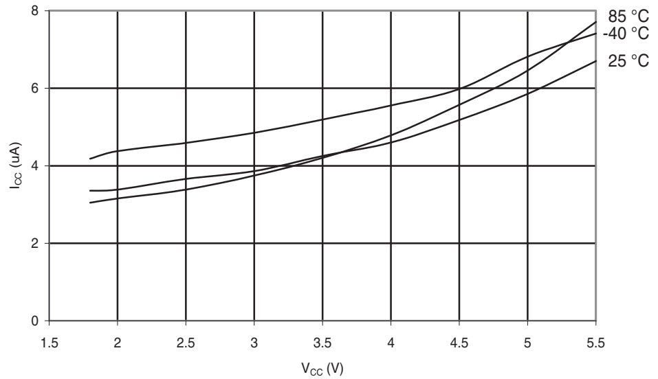
Figure 29-150. ATmega88PA: Power-Down Supply Current vs. V_{CC} (Watchdog Timer Enabled)
