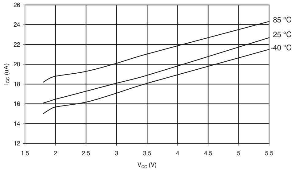
Figure 29-272. ATmega168PA: Brownout Detector Current vs. V_{CC}
