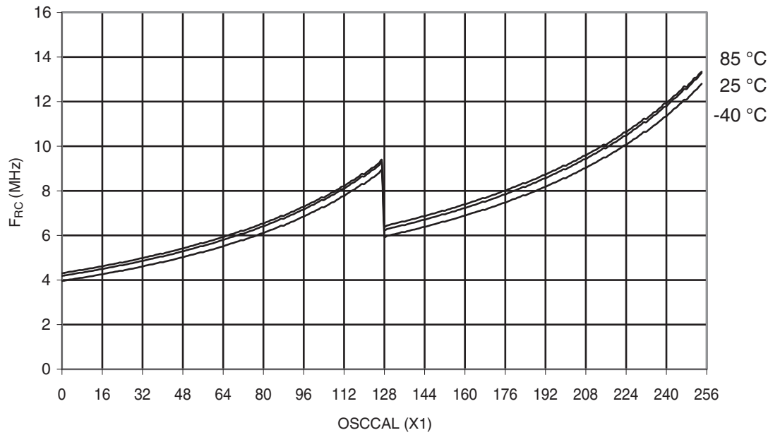
Figure 29-360. ATmega328P: Calibrated 8 MHz RC Oscillator Frequency vs. OSCCAL Value
