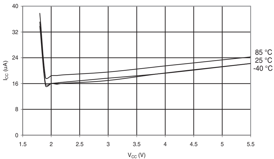
Figure 29-88. ATmega48PA: Brownout Detector Current vs. V_{CC}
