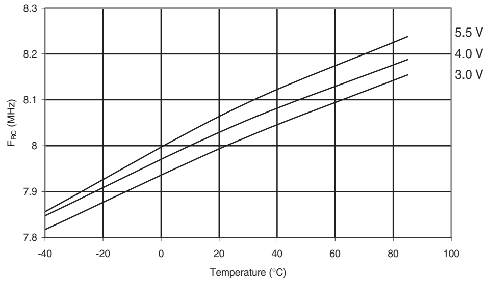
Figure 29-175. ATmega88PA: Calibrated 8 MHz RC Oscillator Frequency vs. Temperature
