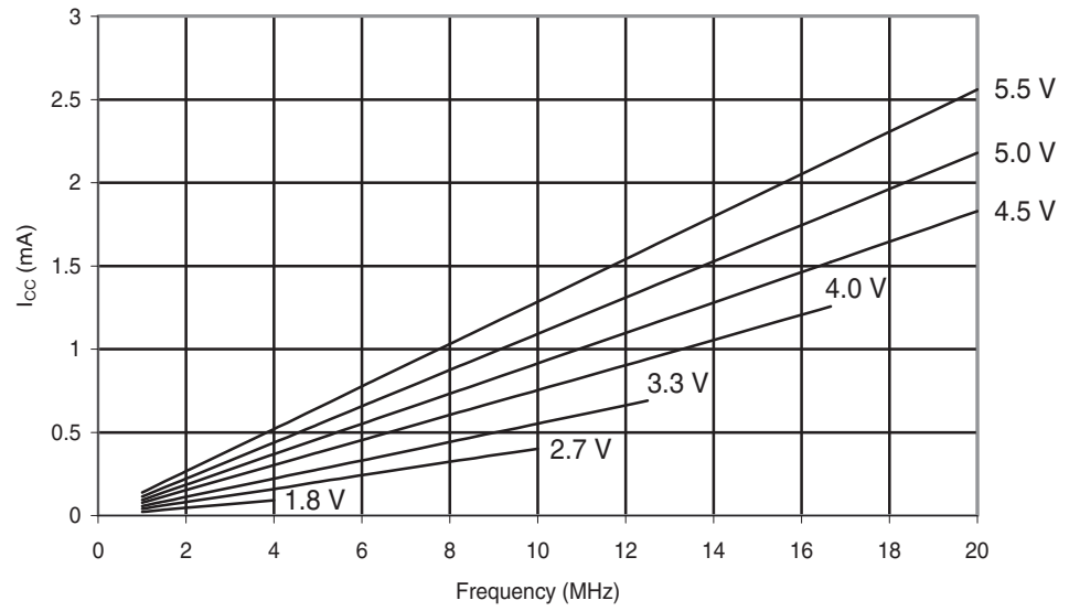
Figure 29-237. ATmega168PA: Idle Supply Current vs. Frequency (1-20 MHz)
