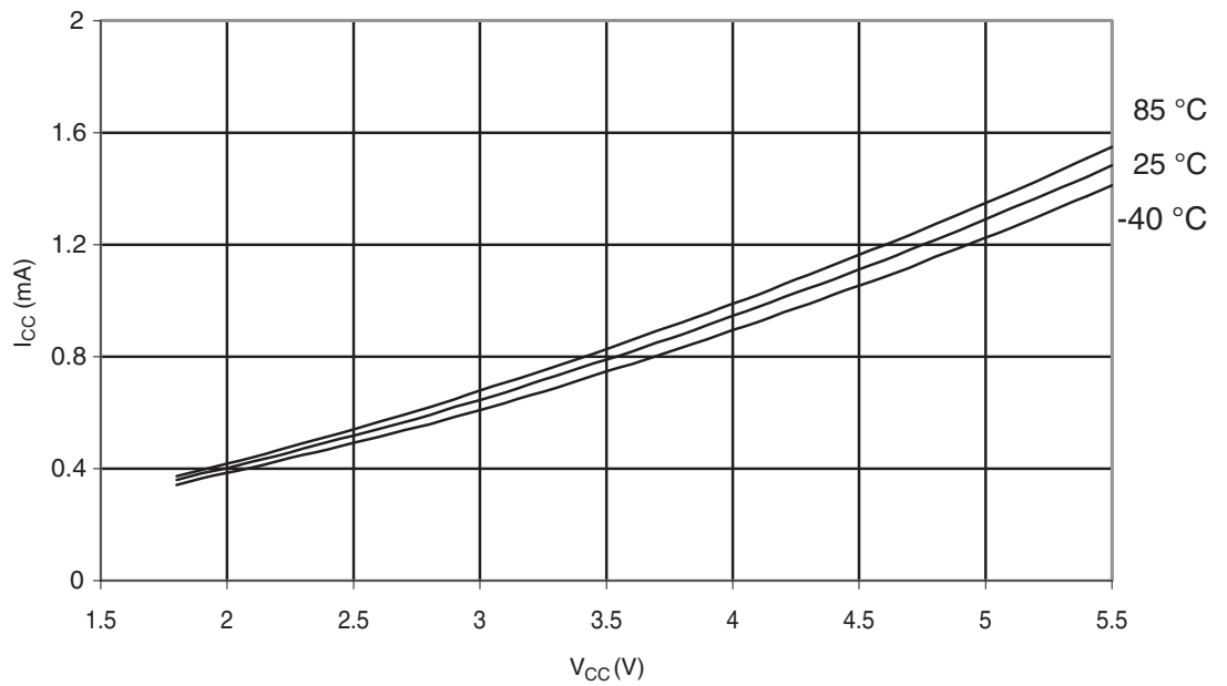
Figure 29-332. ATmega328P: Idle Supply Current vs. V_{CC} (Internal RC Oscillator, 8 MHz)
