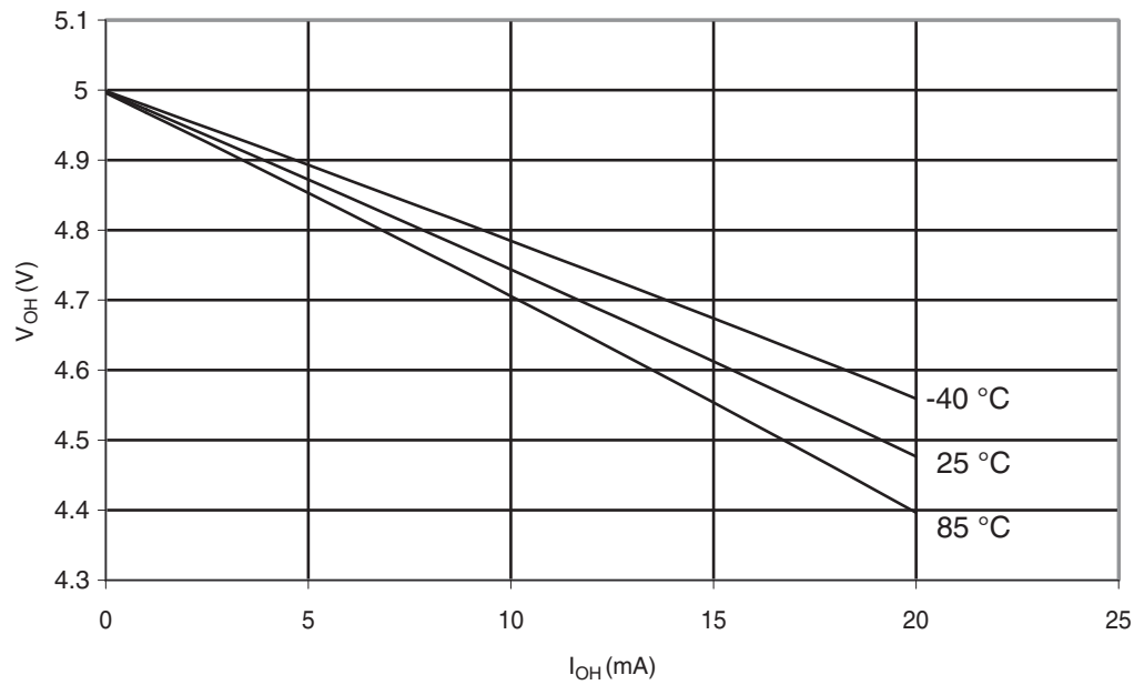
Figure 29-346. ATmega328P: I/O Pin Output Voltage vs. Source Current ( V_{CC} = 5\text{ V} )
