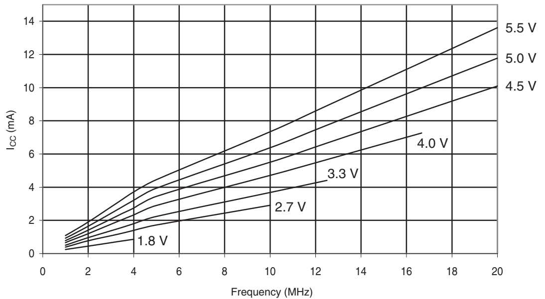
Figure 29-278. ATmega328: Active Supply Current vs. Frequency (1-20 MHz)
