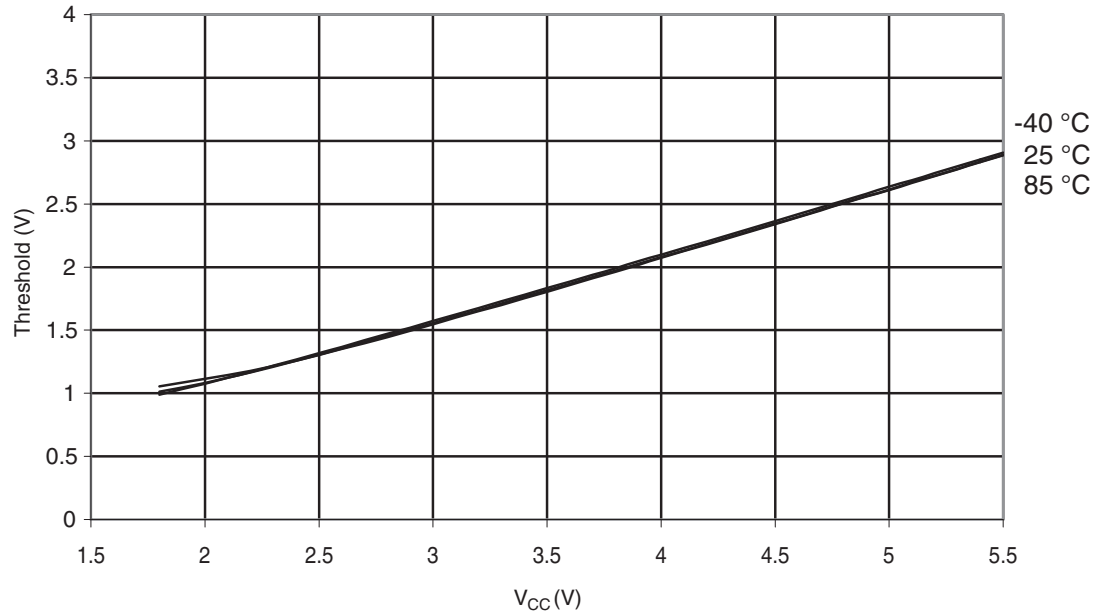
Figure 29-301. ATmega328: I/O Pin Input Threshold Voltage vs. V_{CC} ( V_{IH} , I/O Pin read as '1')
