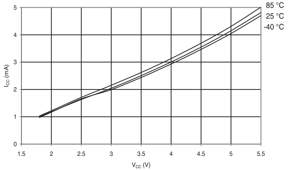
Figure 29-189. ATmega168A: Active Supply Current vs. V_{CC} (Internal RC Oscillator, 8 MHz)
