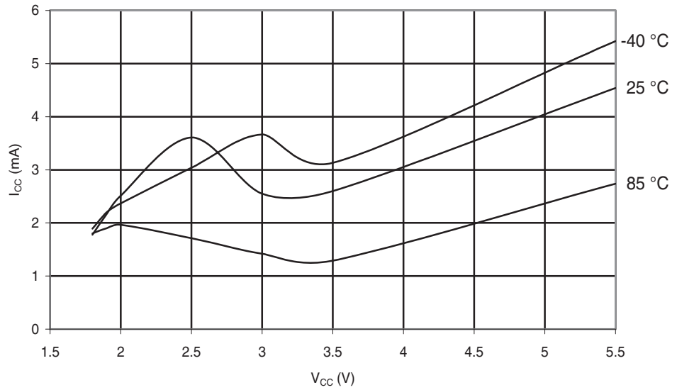
Figure 29-43. ATmega48A: Programming Current vs. V_{CC}
