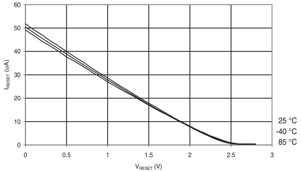
Figure 29-65. ATmega48PA: Reset Pull-up Resistor Current vs. Reset Pin Voltage ( V_{CC} = 2.7\text{ V} )
