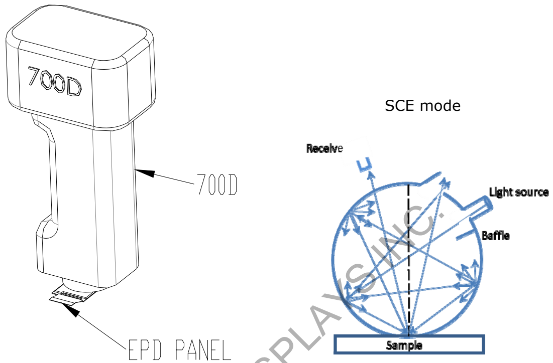
Figure 6-1 Optical measurement
